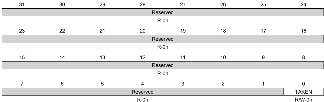
Figure 17-58. LOCK_REG_10 Register
