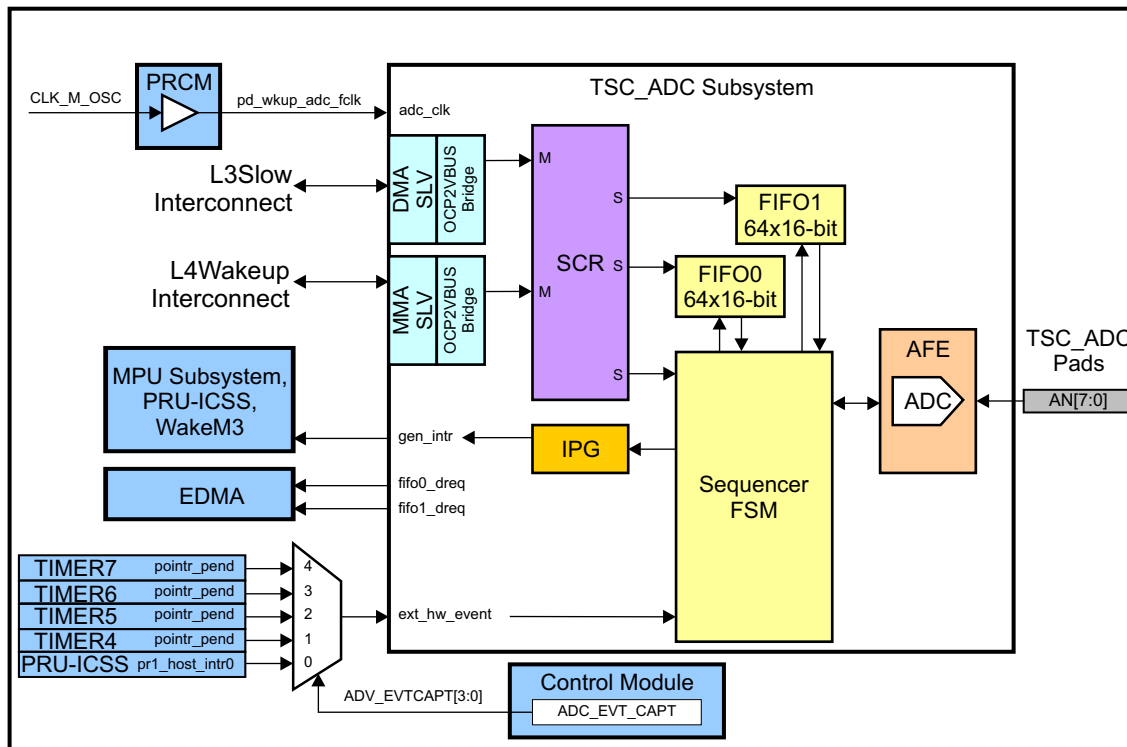
Figure 12-1. TSC_ADC Integration
