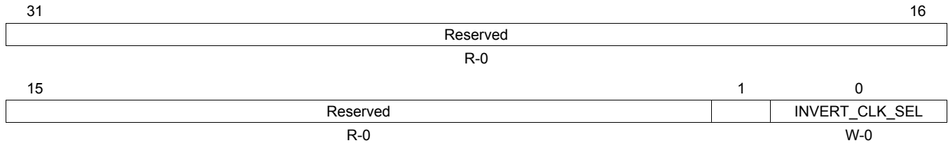
Figure 7-245. DDR PHY Command 0/1/2 Invert Clockout Selection Register( CMD0/1/2_REG_PHY_INVERT_CLKOUT_0)
