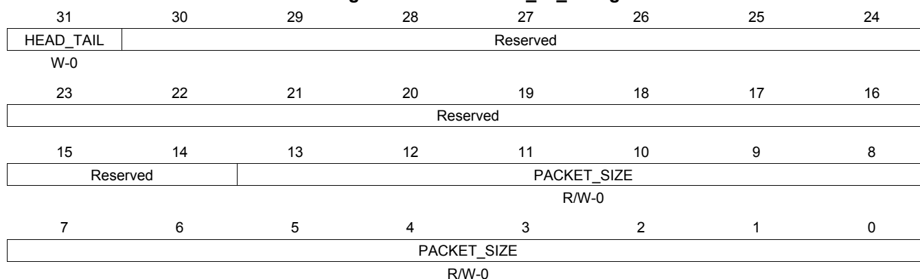
Figure 16-561. QUEUE_62_C Register
