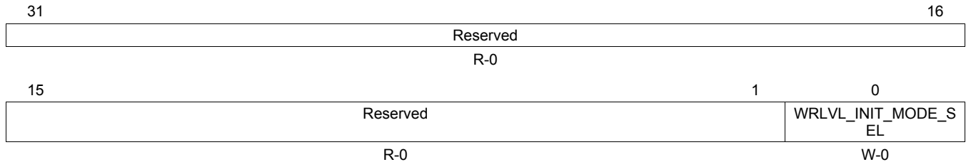
Figure 7-248. DDR PHY Data Macro 0 Write Leveling Init Mode Ratio Selection Register (DATA0/1_REG_PHY_WRLVL_INIT_MODE_0)
