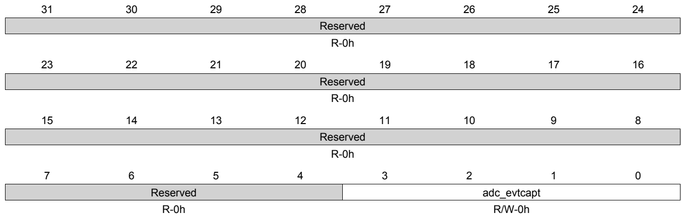
Figure 9-74. adc_evt_capt Register
