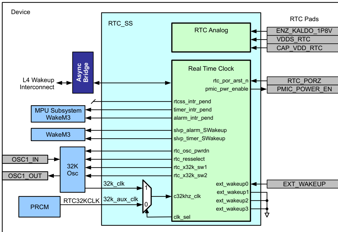
Figure 20-52. RTC Integration
