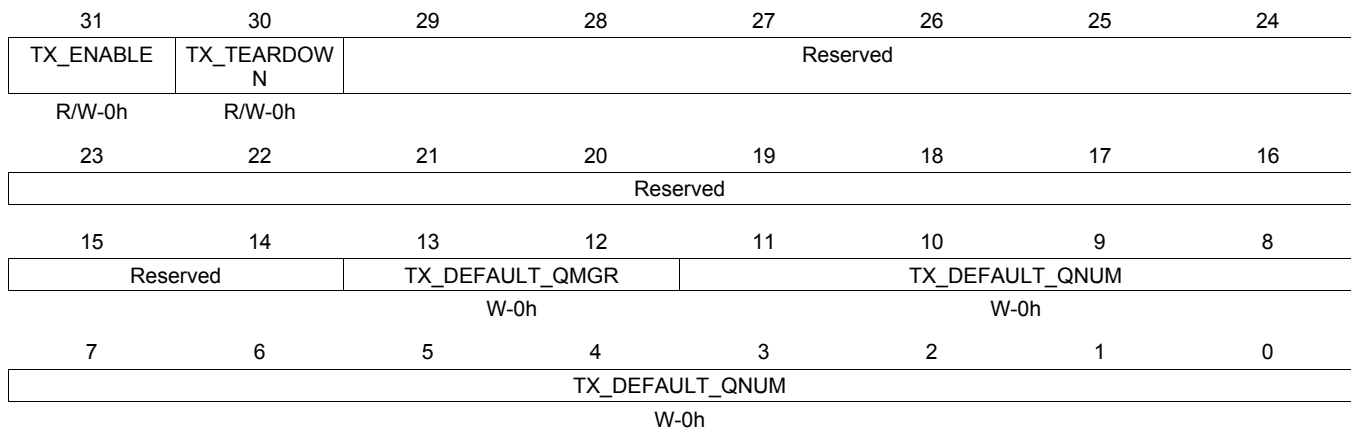
Figure 16-199. TXGCR11 Register
