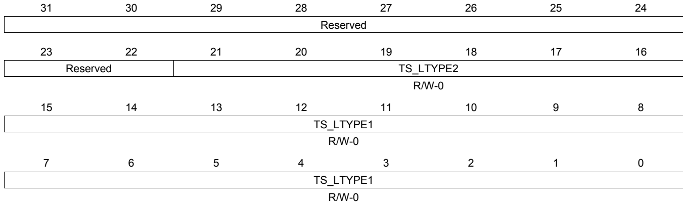
Figure 14-195. TS_LTYPE Register
