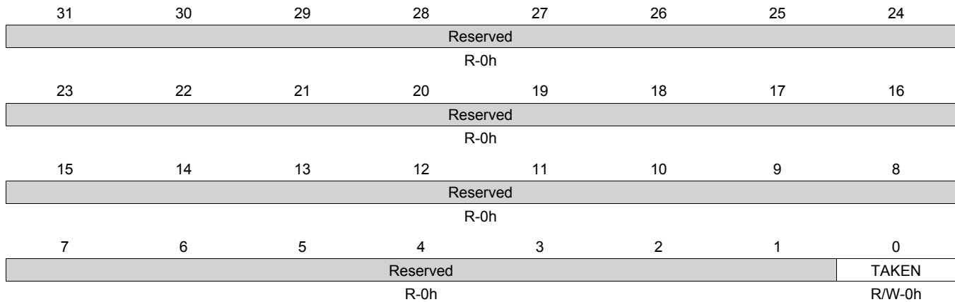
Figure 17-48. LOCK_REG_0 Register
