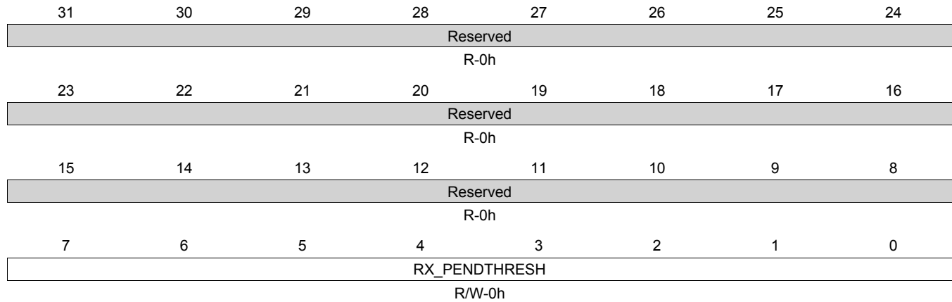
Figure 14-67. RX5_PENDTHRESH Register
