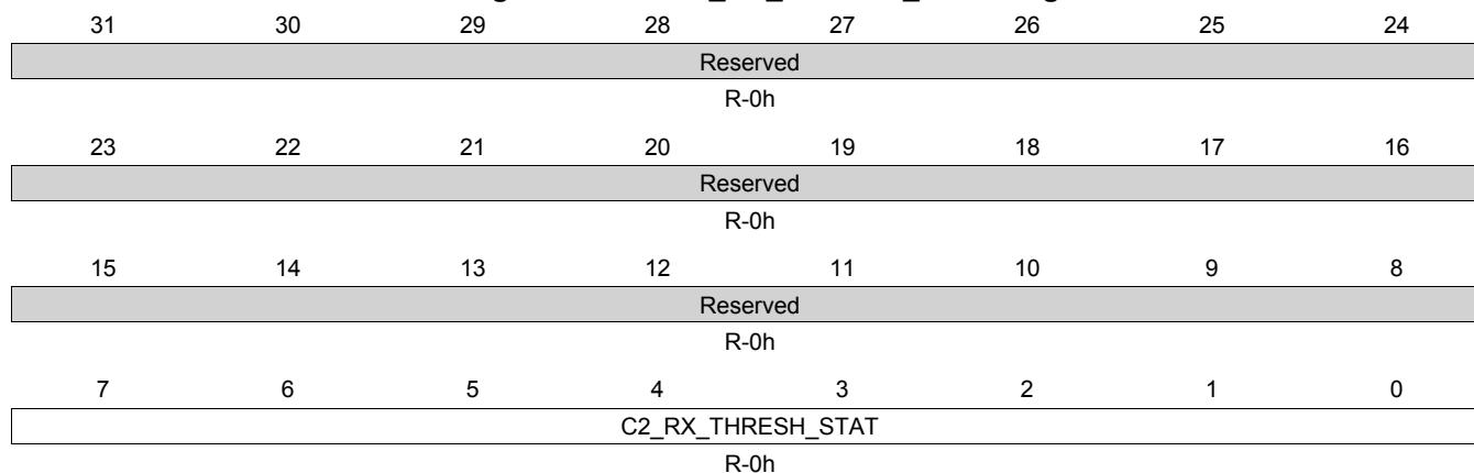
Figure 14-221. C2_RX_THRESH_STAT Register
