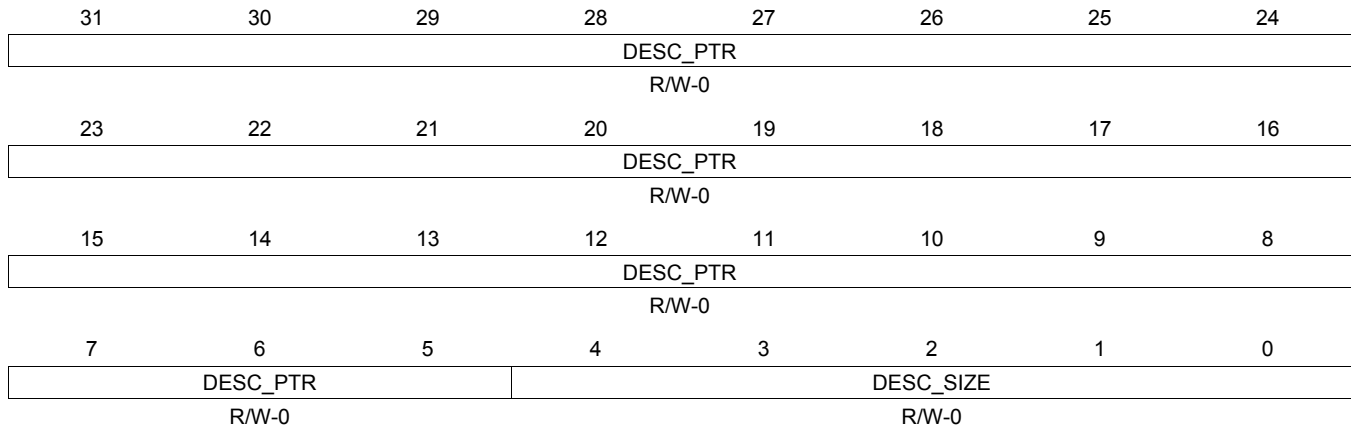
Figure 16-590. QUEUE_69_D Register
