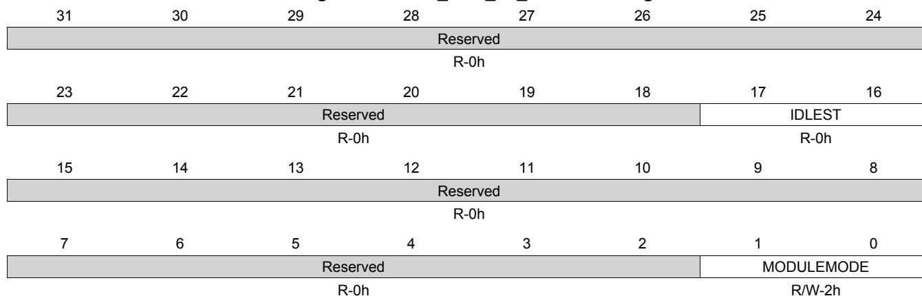
Figure 8-61. CM_PER_L3_CLKCTRL Register
