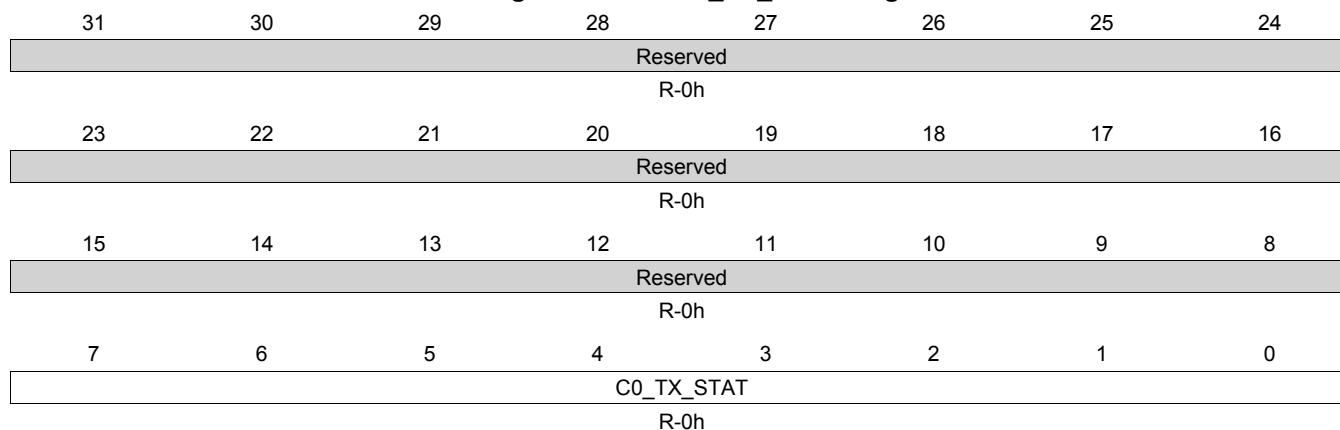
Figure 14-215. C0_TX_STAT Register
