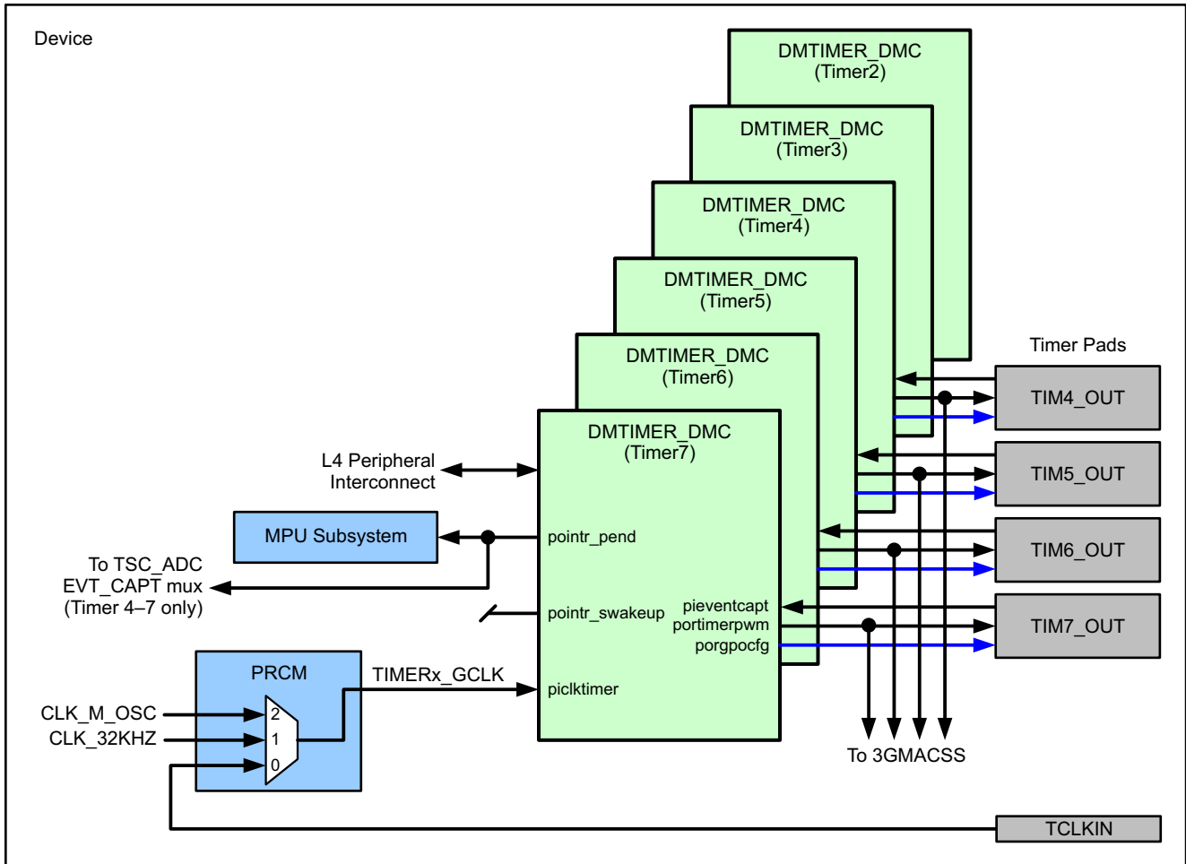
Figure 20-3. Timer2-7 Integration
