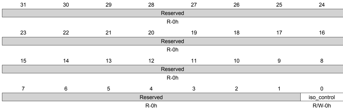
Figure 9-75. reset_iso Register
