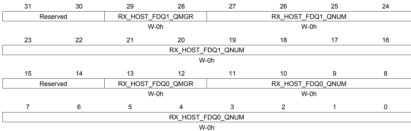
Figure 16-173. RXHPCRA4 Register
