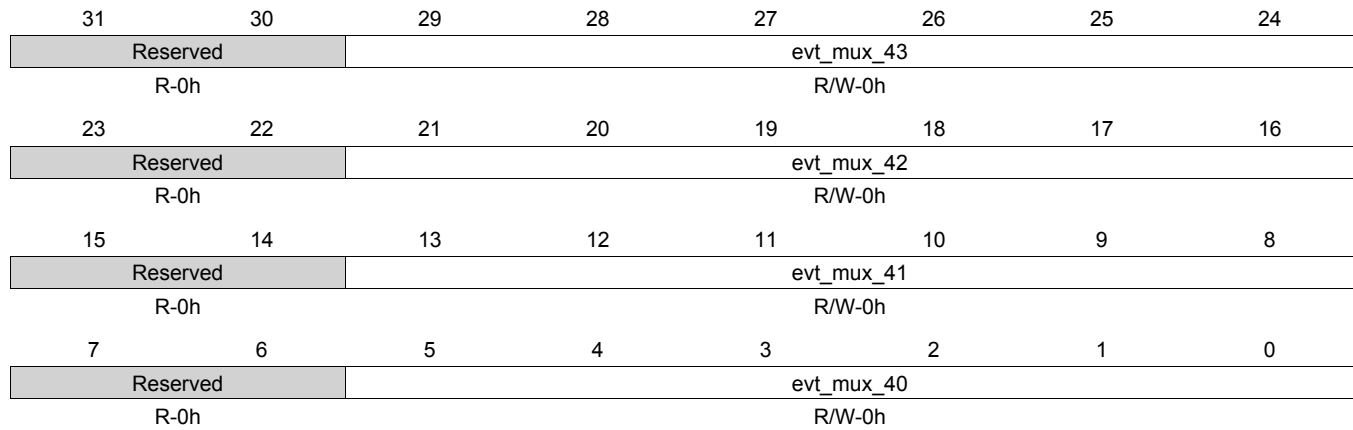
Figure 9-66. tpcc_evt_mux_40_43 Register
