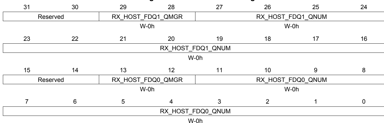
Figure 16-157. RXHPCRA0 Register
