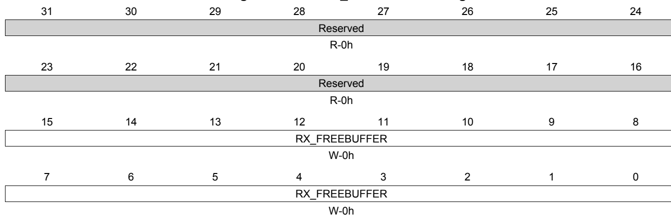
Figure 14-74. RX4_FREEBUFFER Register
