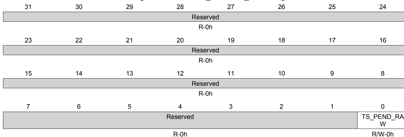
Figure 14-83. CPTS_INTSTAT_RAW Register
