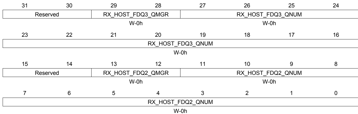
Figure 16-190. RXHPCRB8 Register
