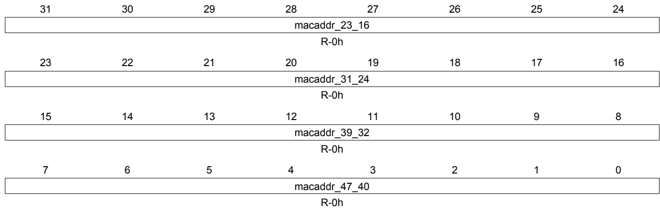
Figure 9-26. mac_id0_hi Register
