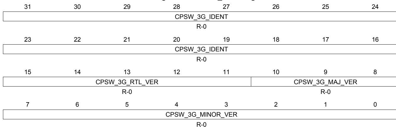
Figure 14-184. ID_VER Register
