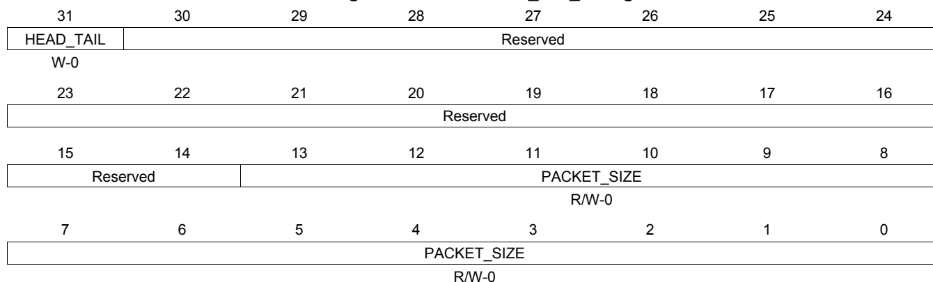
Figure 16-837. QUEUE_131_C Register
