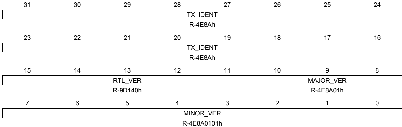
Figure 14-78. CPTS_IDVER Register
