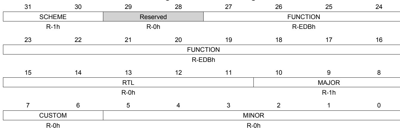
Figure 14-197. IDVER Register
