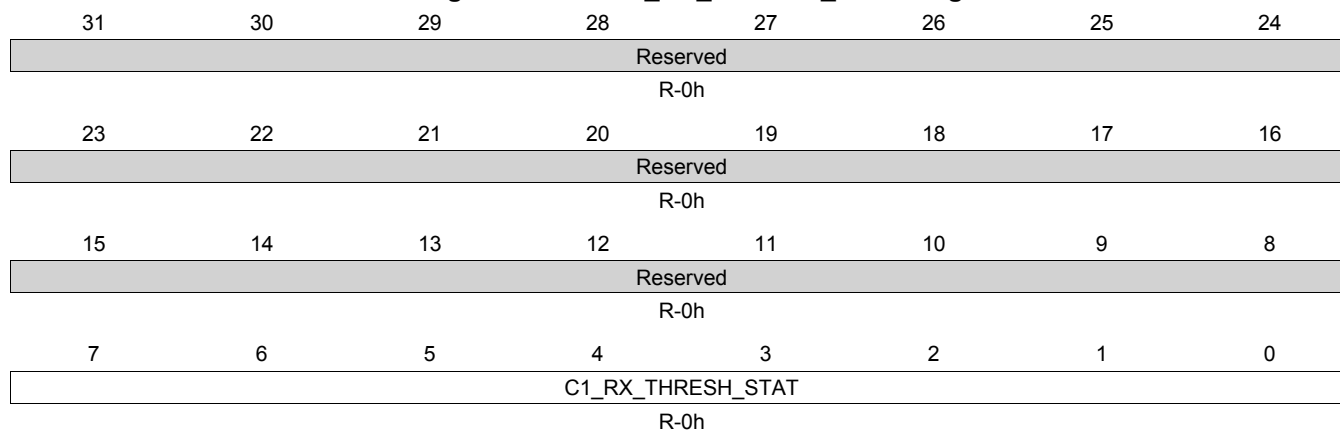
Figure 14-217. C1_RX_THRESH_STAT Register
