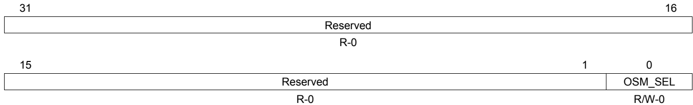
Figure 4-200. Mode Definition Register (MDR)
