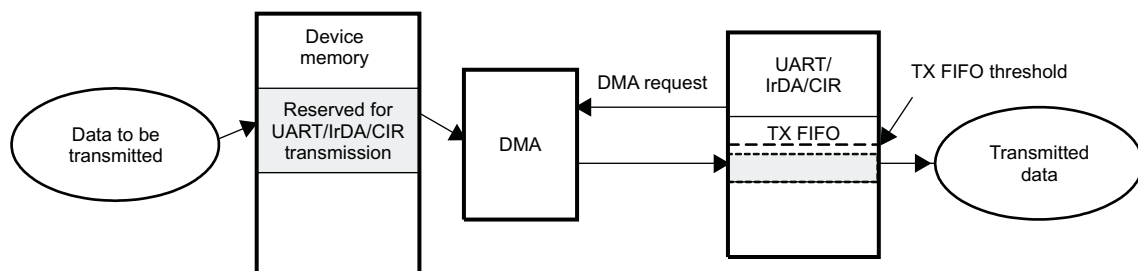
Figure 19-12. DMA Transmission
