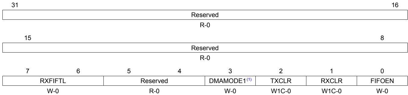
Figure 4-189. FIFO Control Register (FCR)
