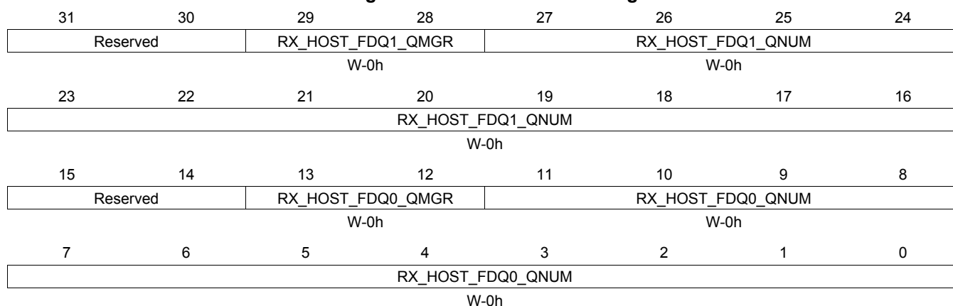
Figure 16-269. RXHPCRA28 Register
