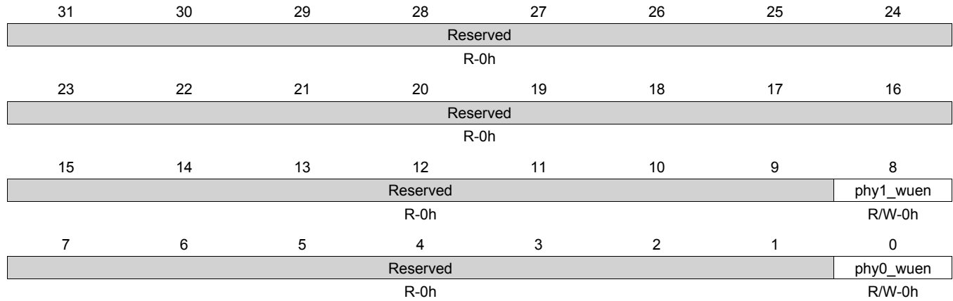
Figure 9-30. usb_wkup_ctrl Register
