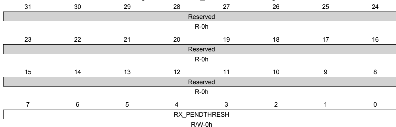
Figure 14-62. RX0_PENDTHRESH Register
