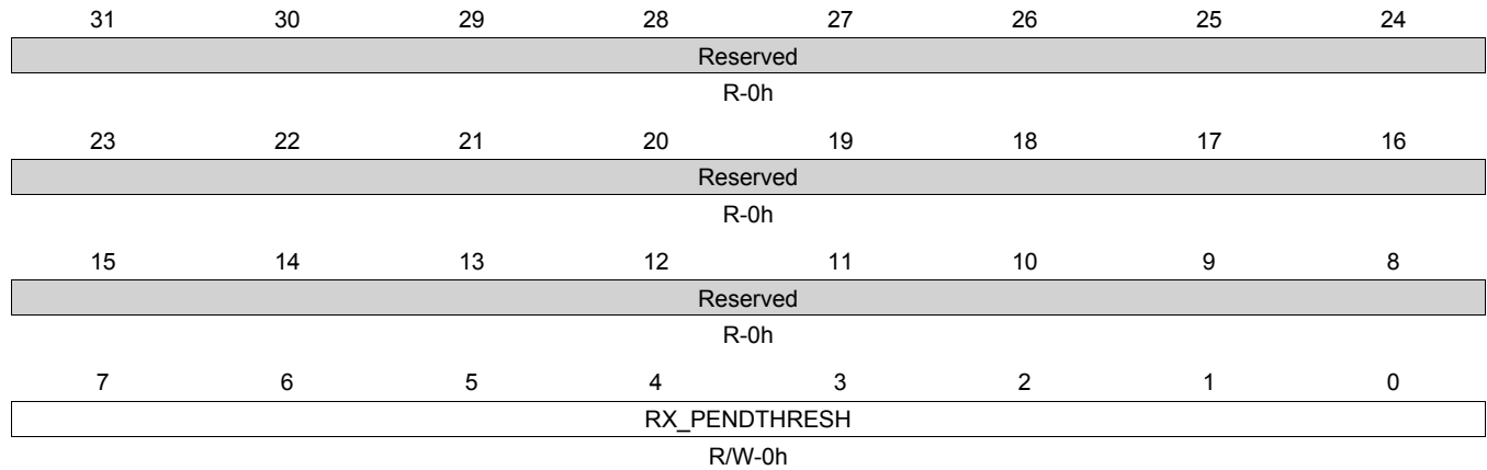
Figure 14-63. RX1_PENDTHRESH Register
