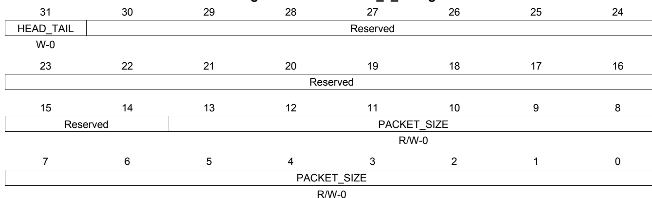
Figure 16-329. QUEUE_4_C Register
