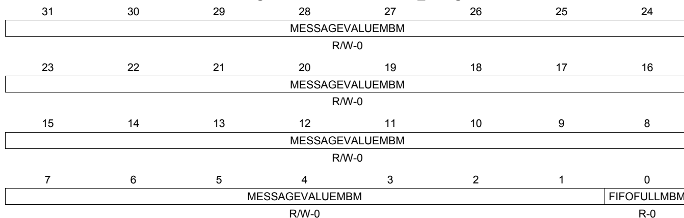
Figure 17-18. FIFOSTATUS_5 Register
