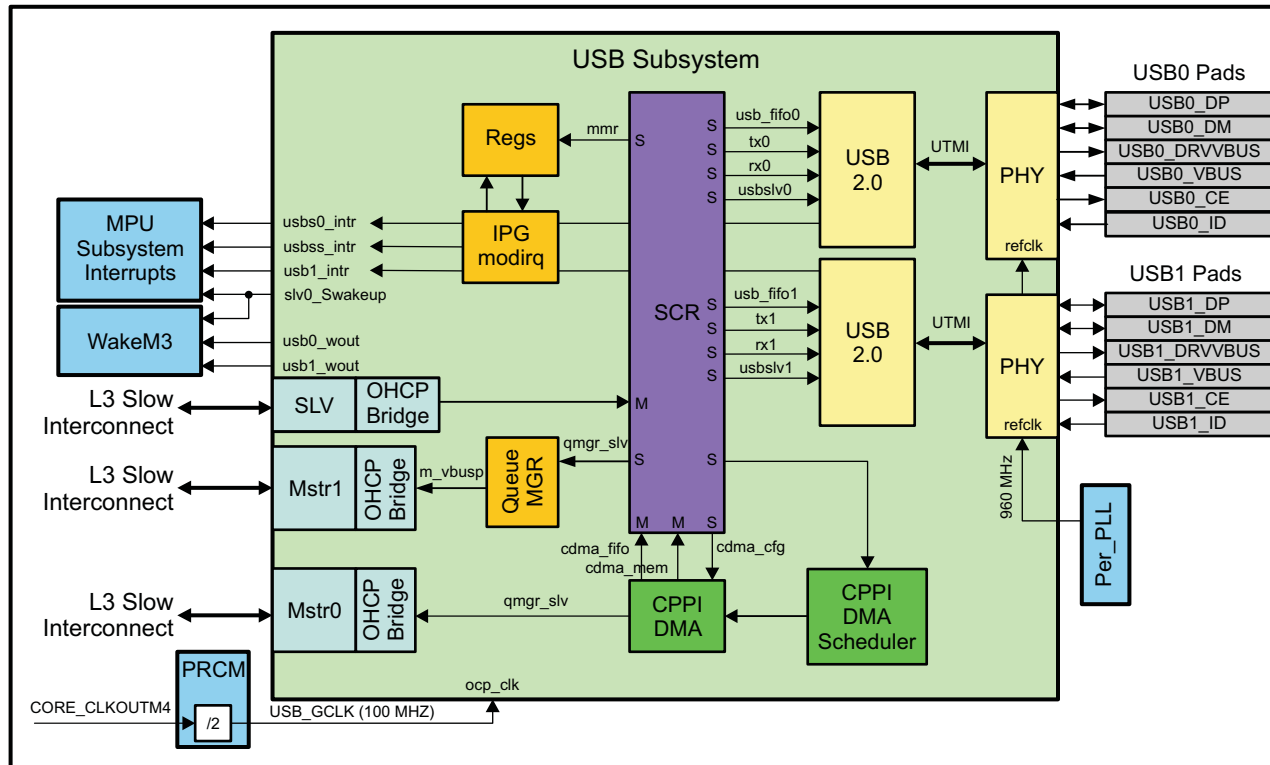
Figure 16-1. USB Integration
