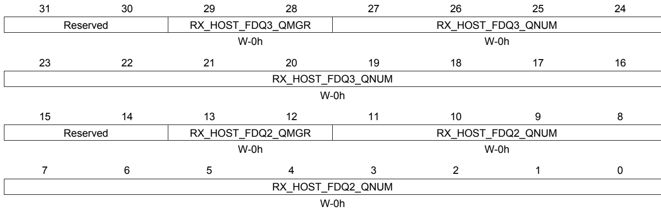
Figure 16-158. RXHPCR0 Register
