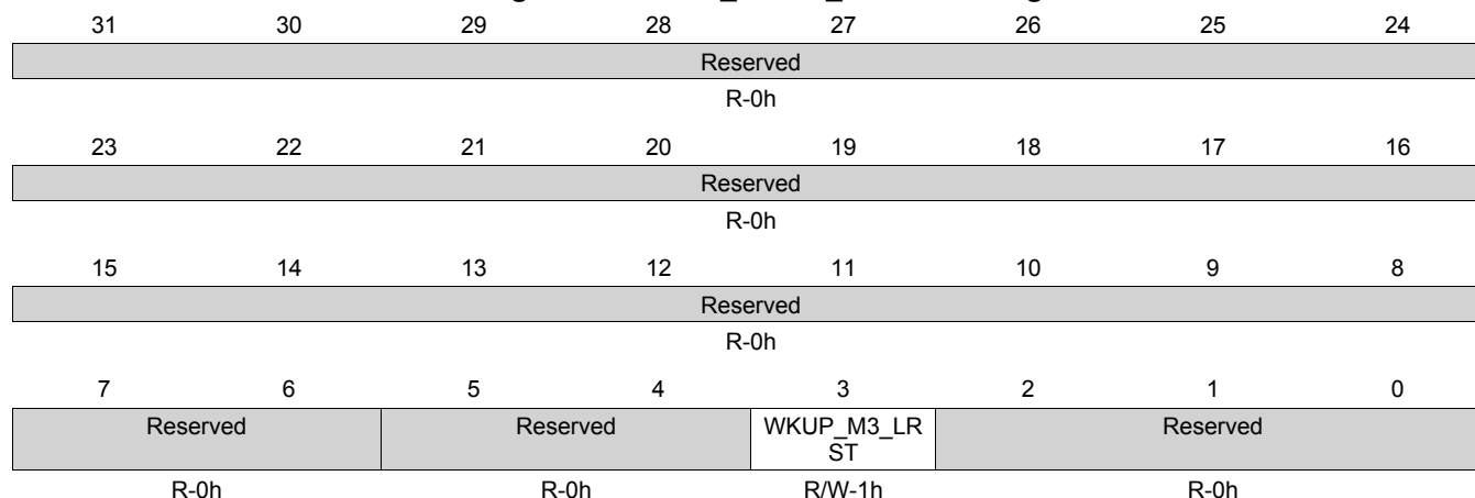
Figure 8-169. RM_WKUP_RSTCTRL Register
