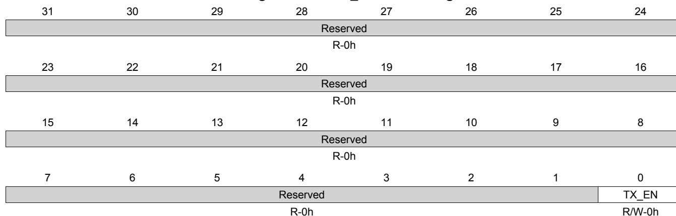
Figure 14-30. TX_CONTROL Register
