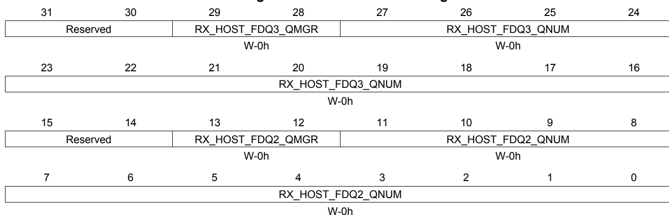
Figure 16-250. RXHPCRB23 Register
