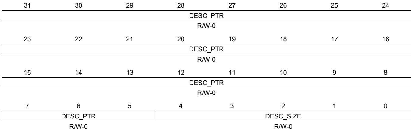
Figure 16-646. QUEUE_83_D Register
