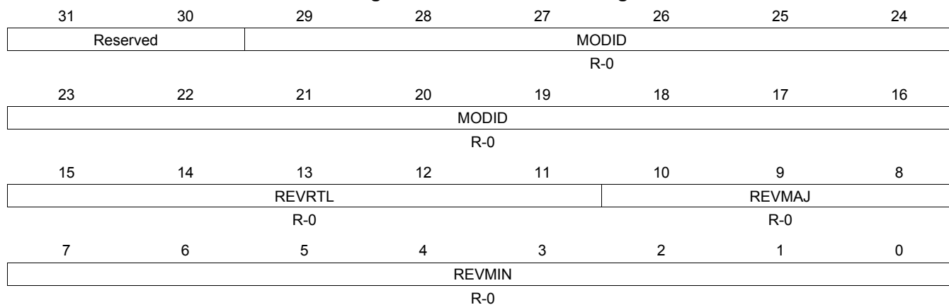
Figure 16-152. DMAREVID Register
