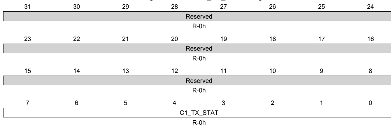
Figure 14-219. C1_TX_STAT Register
