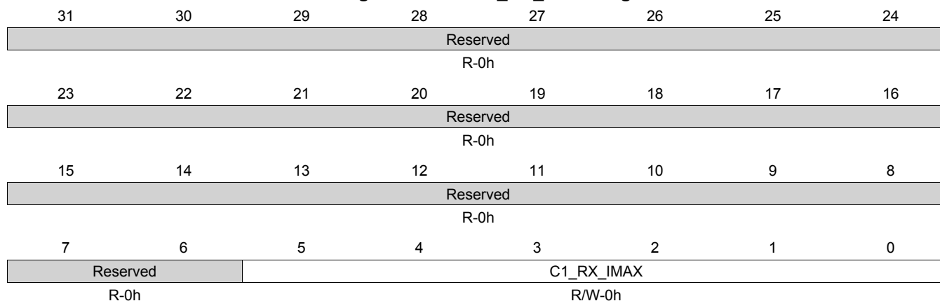
Figure 14-227. C1_RX_IMAX Register
