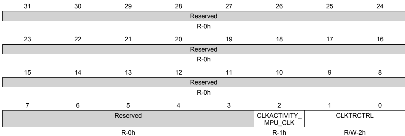
Figure 8-149. CM_MPU_CLKSTCTRL Register
