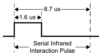
Figure 19-22. SIP Pulse
