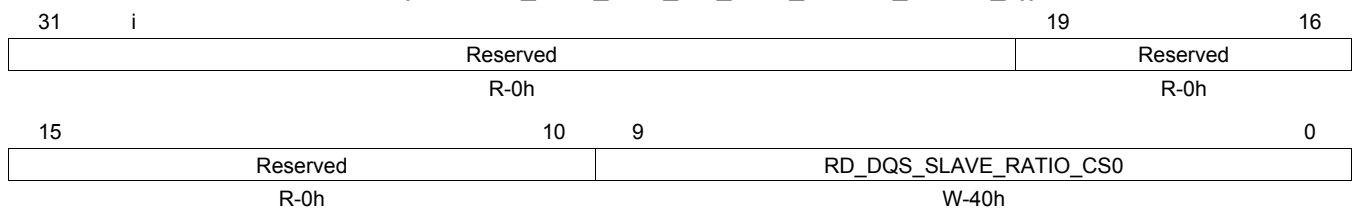
Figure 7-246. DDR PHY Data Macro 0/1 Read DQS Slave Ratio Register (DATA0/1_REG_PHY_RD_DQS_SLAVE_RATIO_0)
