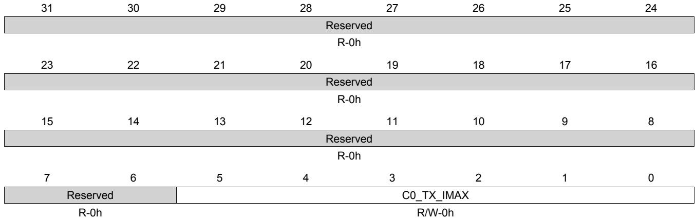
Figure 14-226. C0_TX_IMAX Register
