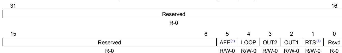
Figure 4-191. Modem Control Register (MCR)
