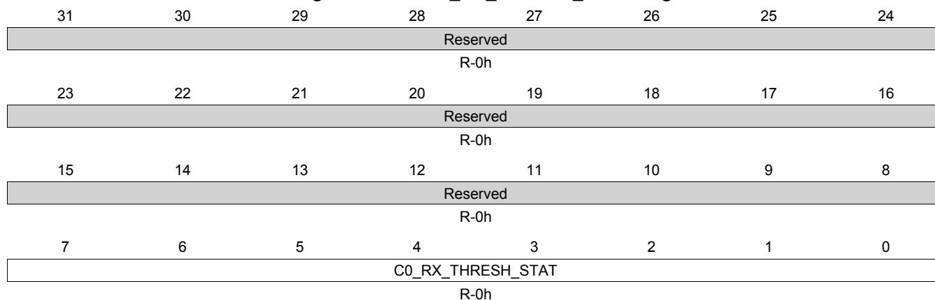
Figure 14-213. C0_RX_THRESH_STAT Register
