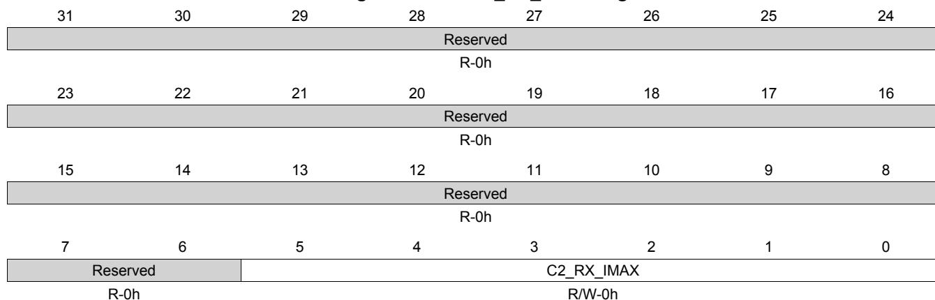
Figure 14-229. C2_RX_IMAX Register
