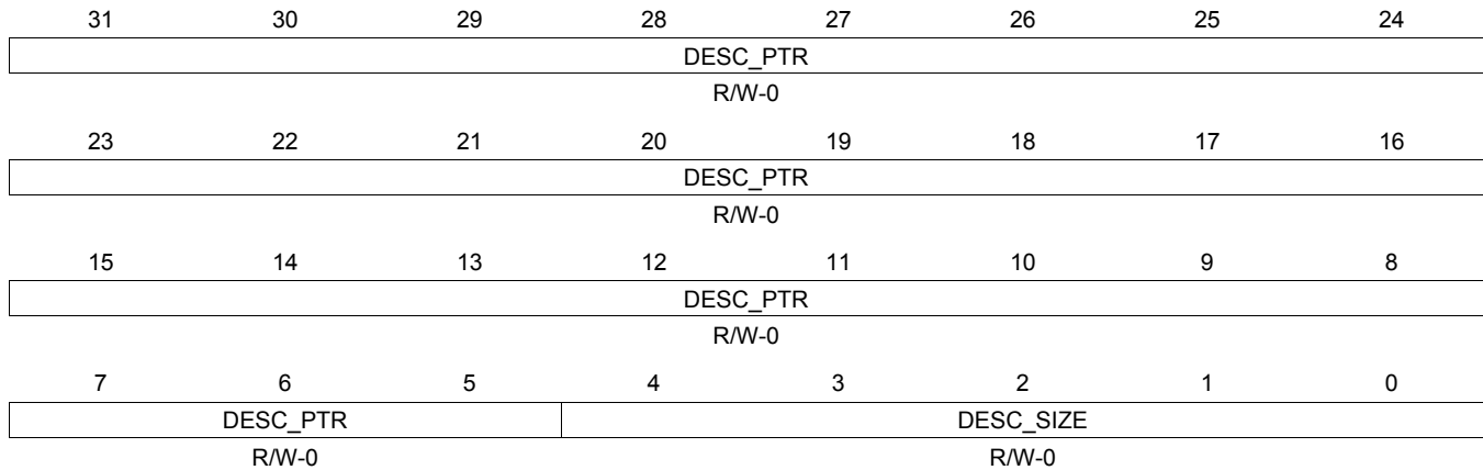
Figure 16-598. QUEUE_71_D Register
