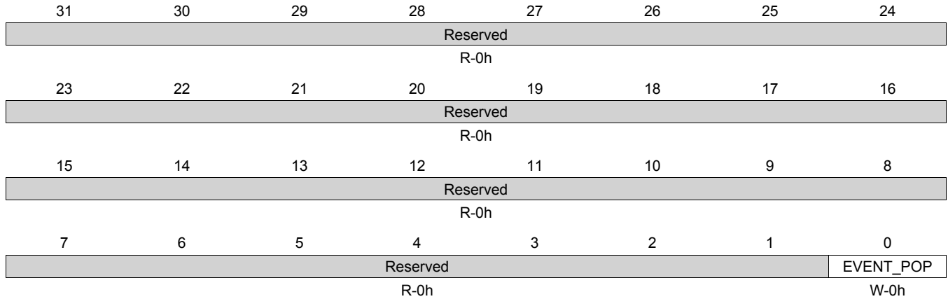
Figure 14-86. CPTS_EVENT_POP Register
