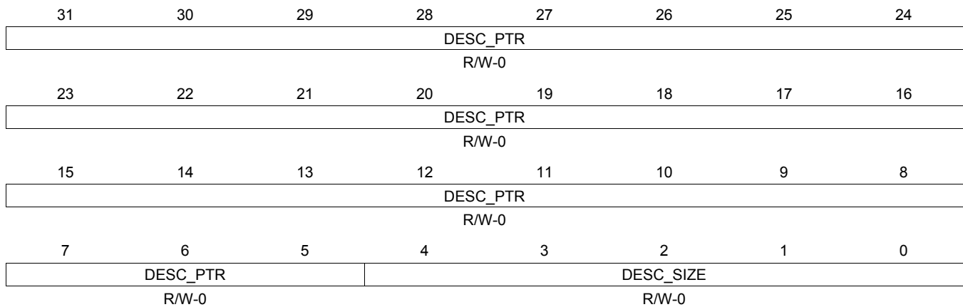
Figure 16-798. QUEUE_121_D Register
