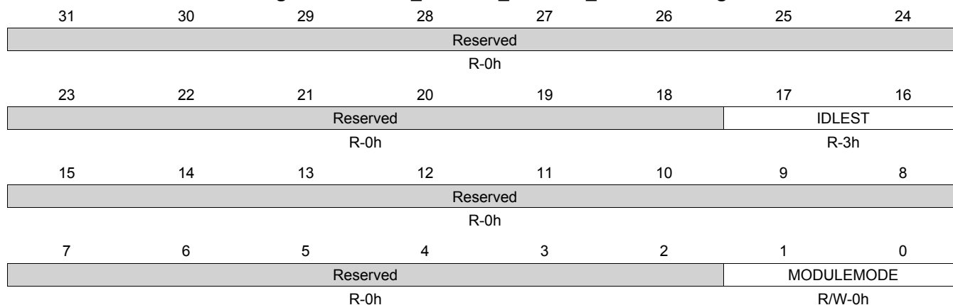
Figure 8-160. CM_CEFUSE_CEFUSE_CLKCTRL Register
