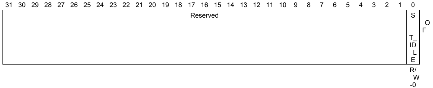
Figure 14-189. SOFT_IDLE Register
