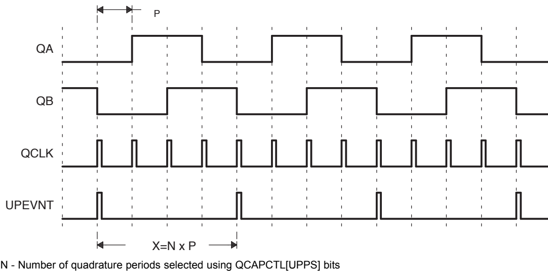
Figure 15-145. Unit Position Event for Low Speed Measurement (QCAPCTL[UPPS] = 0010)
