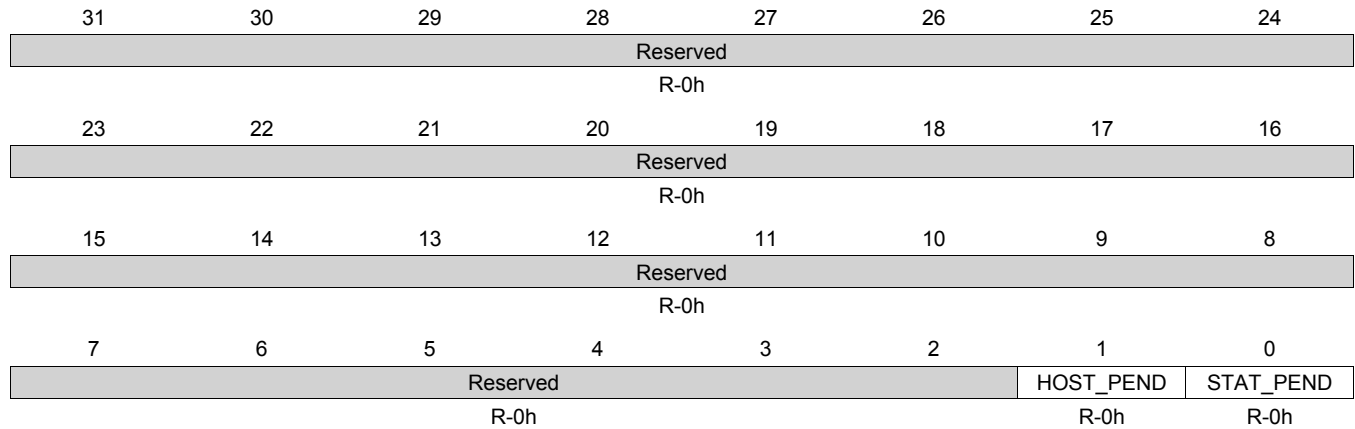
Figure 14-59. DMA_INTSTAT_MASKED Register
