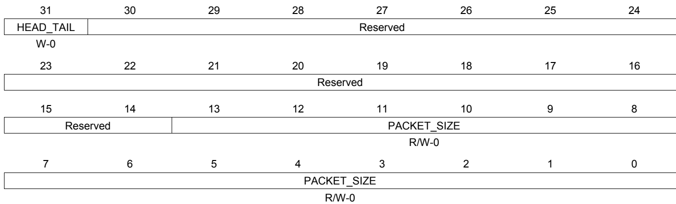
Figure 16-841. QUEUE_132_C Register
