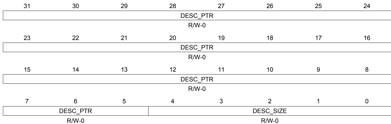
Figure 16-314. QUEUE_0_D Register
