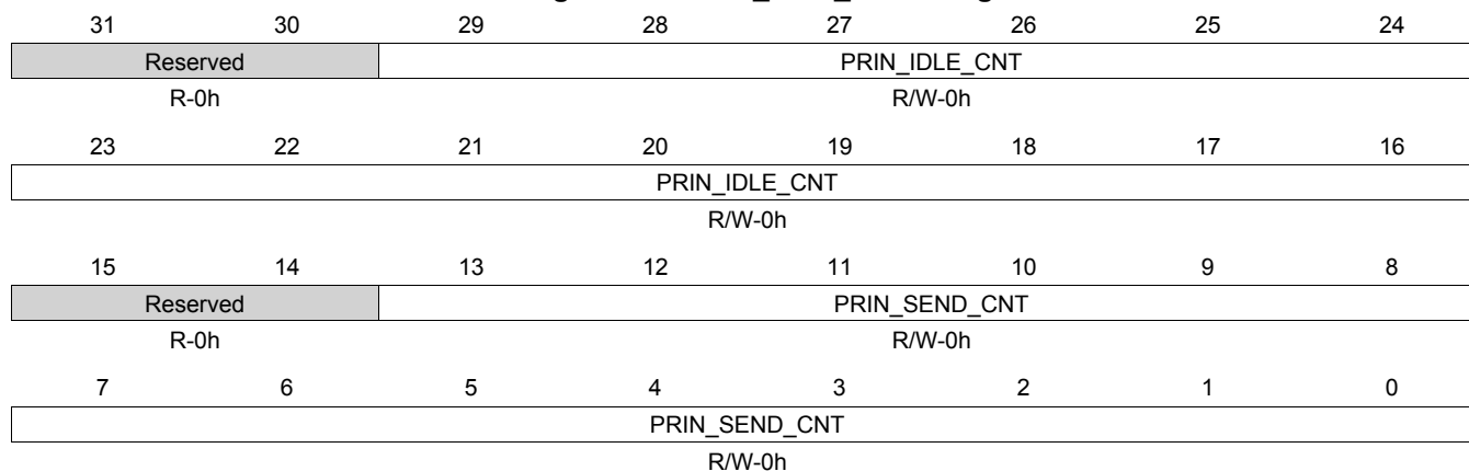
Figure 14-40. TX_PRI0_RATE Register
