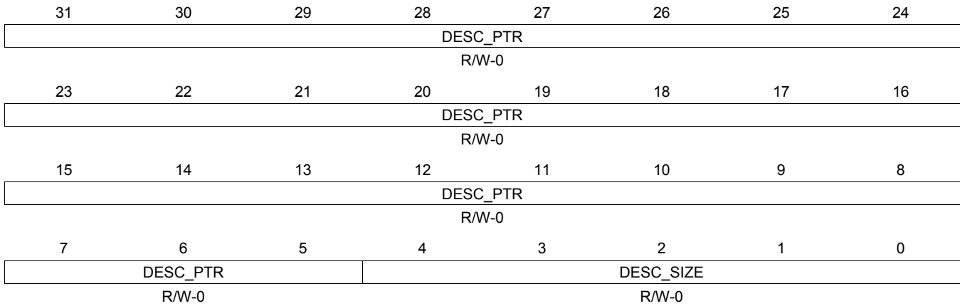
Figure 16-510. QUEUE_49_D Register
