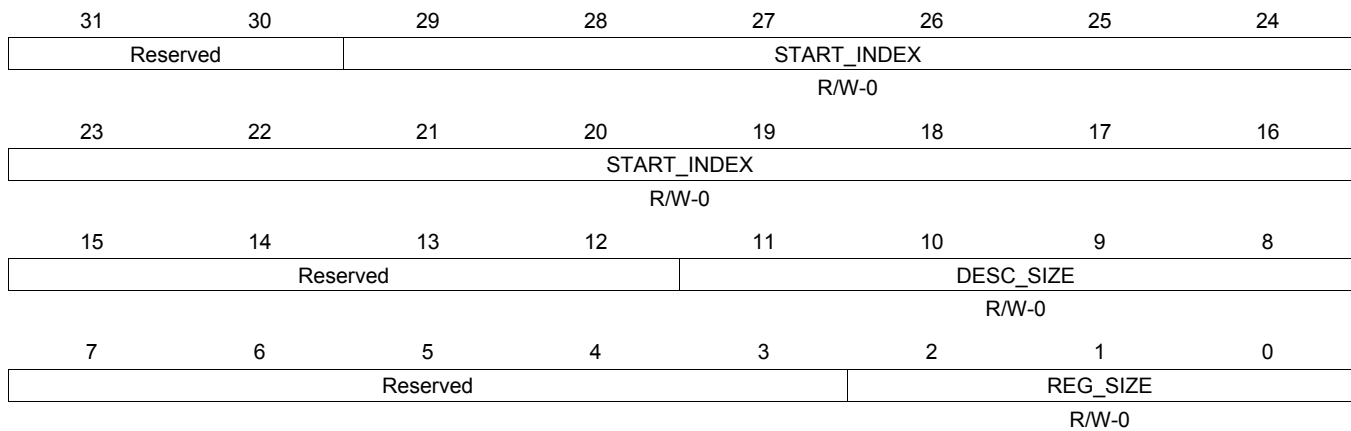
Figure 16-296. QMEMCTRL0 Register
