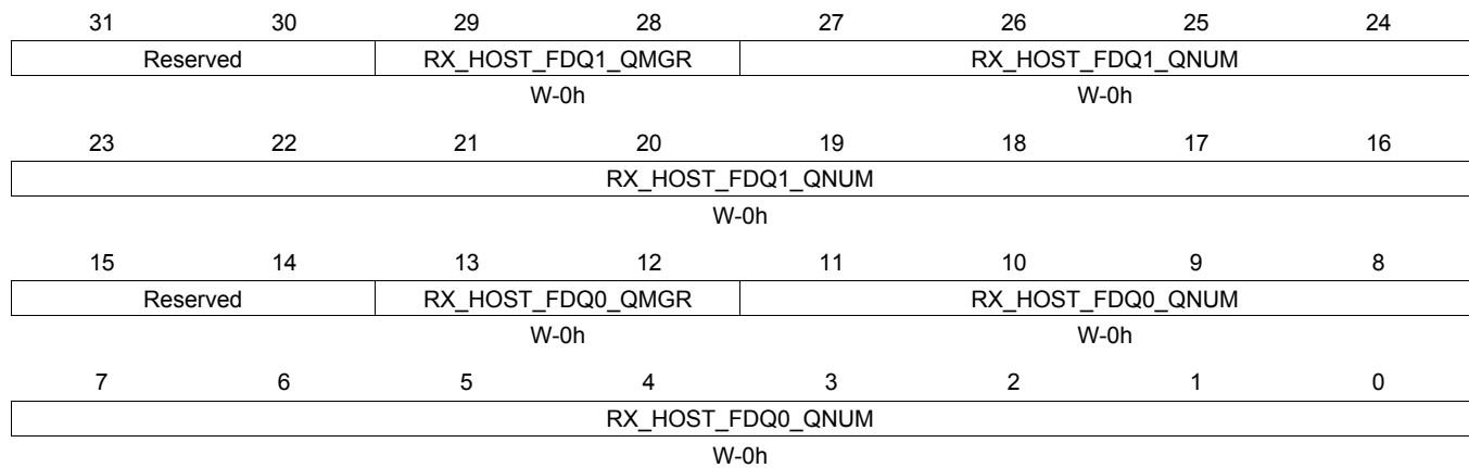
Figure 16-225. RXHPCRA17 Register
