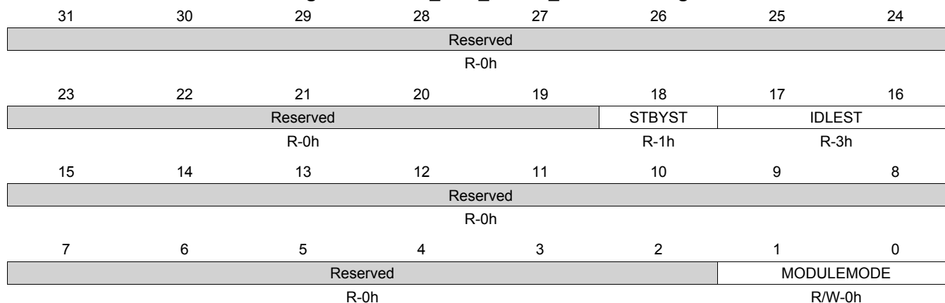
Figure 8-29. CM_PER_TPTC0_CLKCTRL Register
