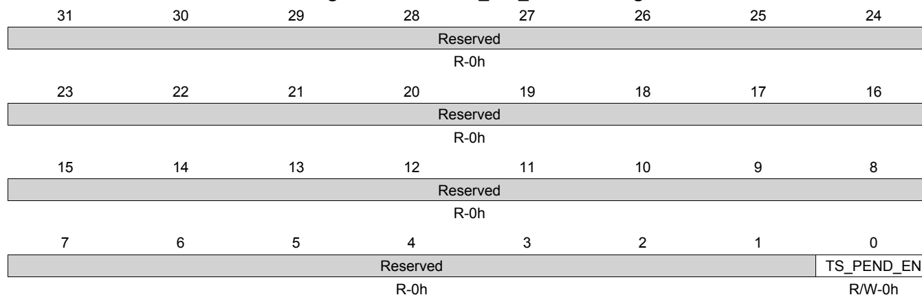
Figure 14-85. CPTS_INT_ENABLE Register
