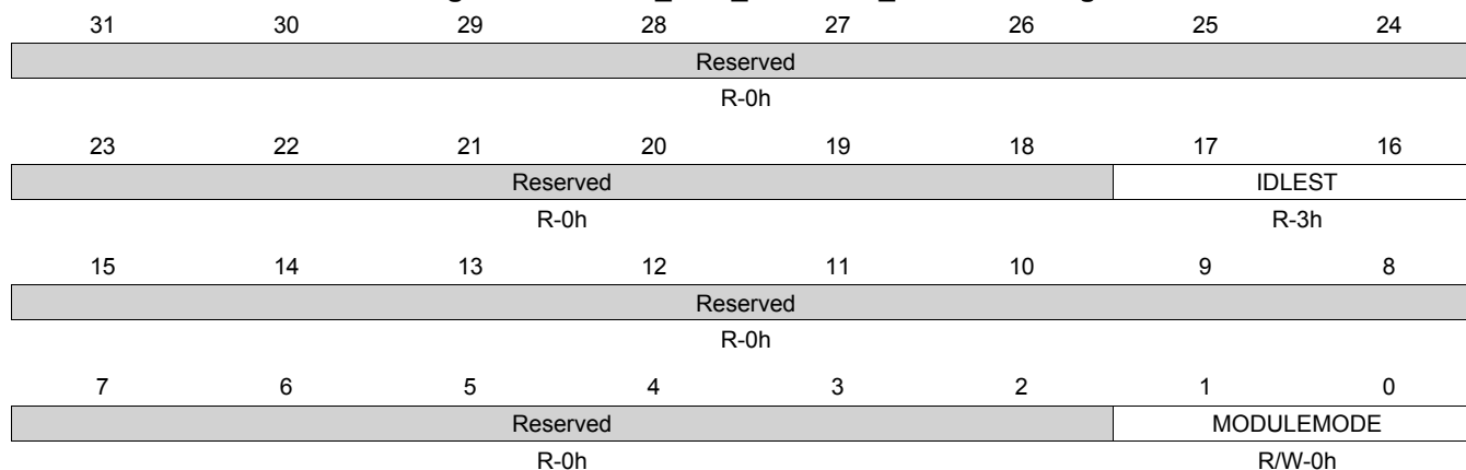
Figure 8-157. CM_GFX_MMUCFG_CLKCTRL Register
