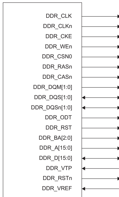
Figure 7-202. DDR2/3/mDDR Memory Controller Signals
