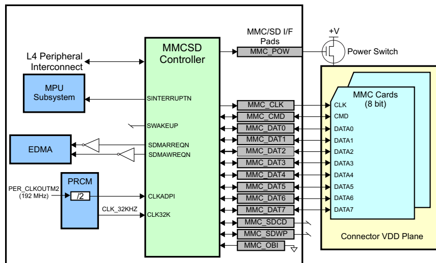
MMCHS Module MMC Application
