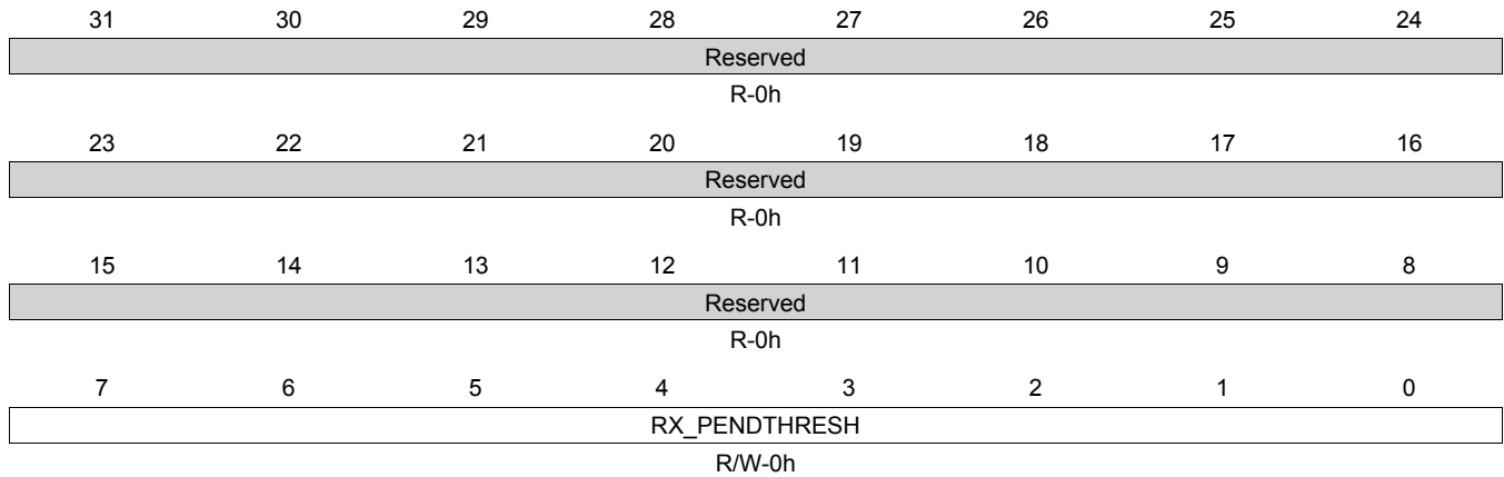
Figure 14-69. RX7_PENDTHRESH Register
