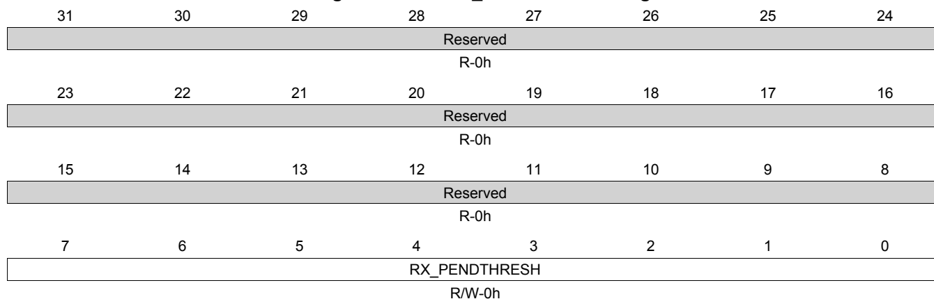
Figure 14-64. RX2_PENDTHRESH Register
