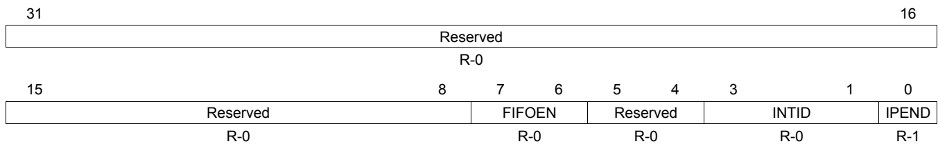
Figure 4-188. Interrupt Identification Register (IIR)
