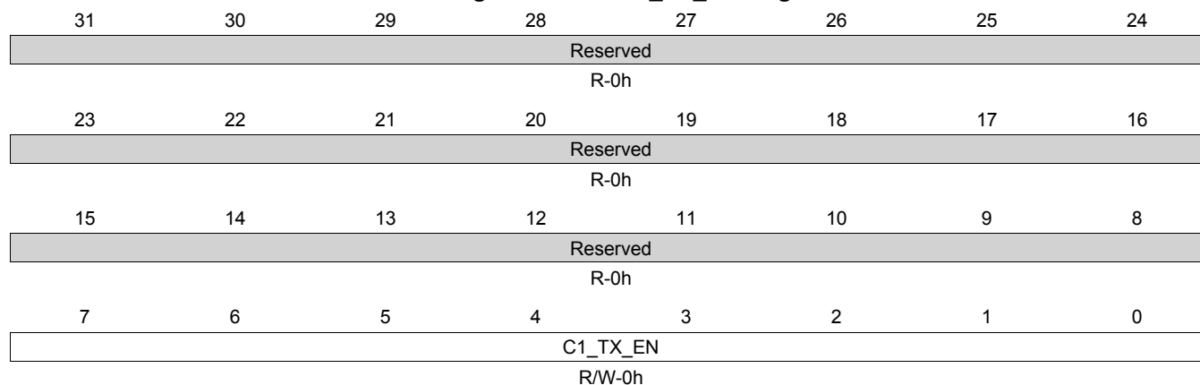
Figure 14-207. C1_TX_EN Register
