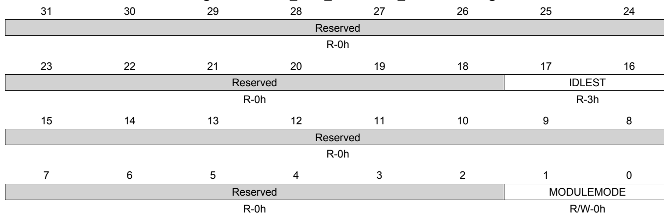
Figure 8-57. CM_PER_EPWMSS1_CLKCTRL Register
