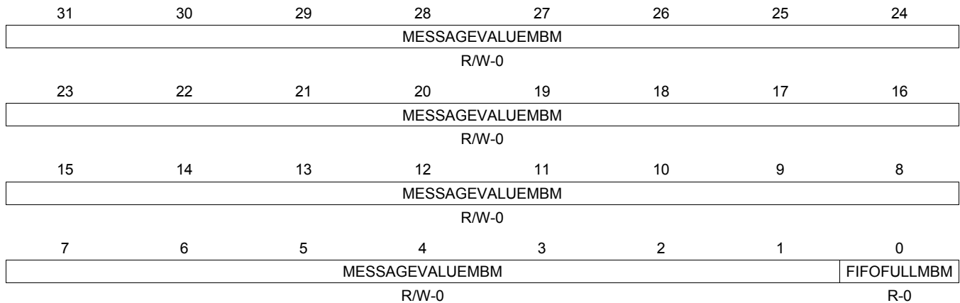
Figure 17-15. FIFOSTATUS_2 Register
