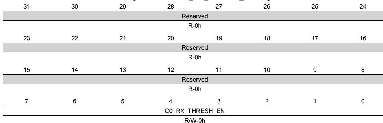
Figure 14-201. C0_RX_THRESH_EN Register
