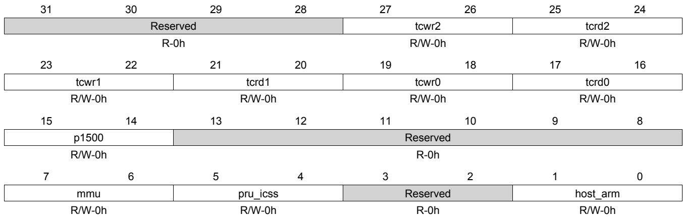
Figure 9-18. init_priority_0 Register
