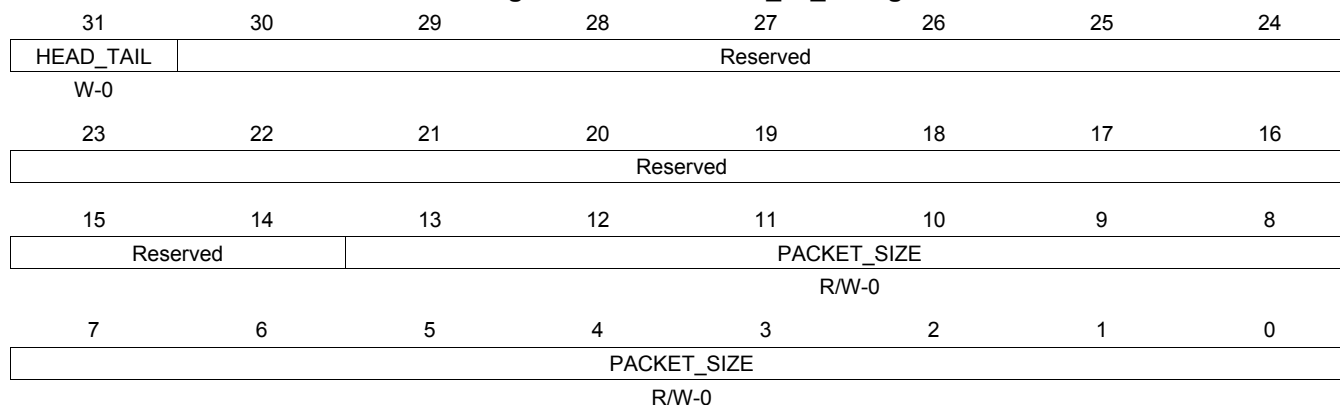
Figure 16-617. QUEUE_76_C Register
