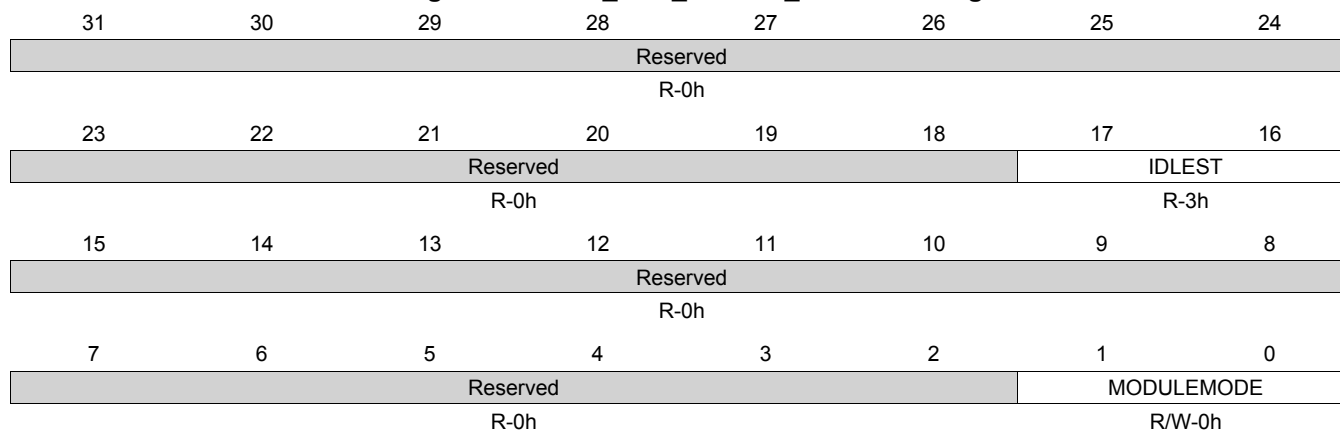
Figure 8-49. CM_PER_TIMER3_CLKCTRL Register
