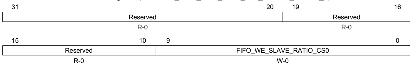
Figure 7-251. DDR PHY Data Macro 0/1 DQS Gate Slave Ratio Register (DATA0/1_REG_PHY_FIFO_WE_SLAVE_RATIO_0)
