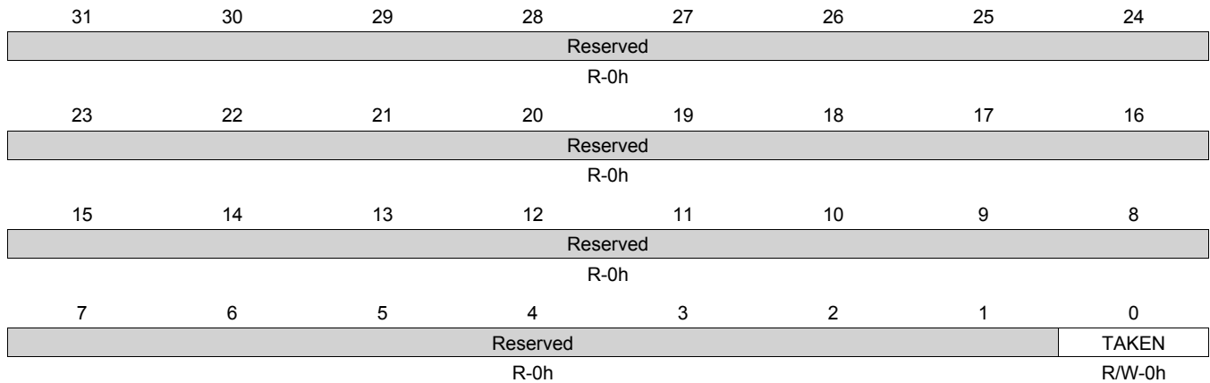
Figure 17-72. LOCK_REG_24 Register
