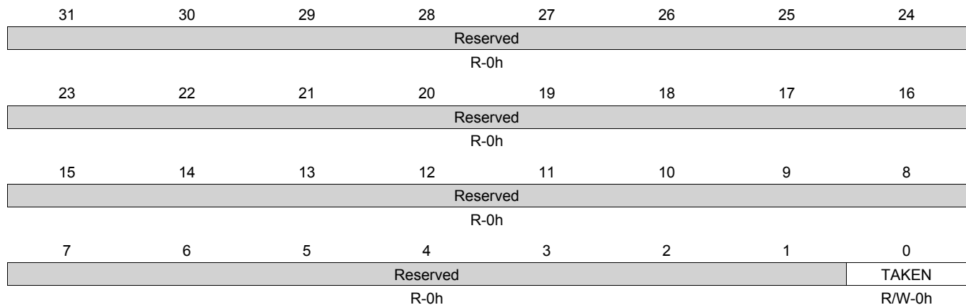
Figure 17-56. LOCK_REG_8 Register
