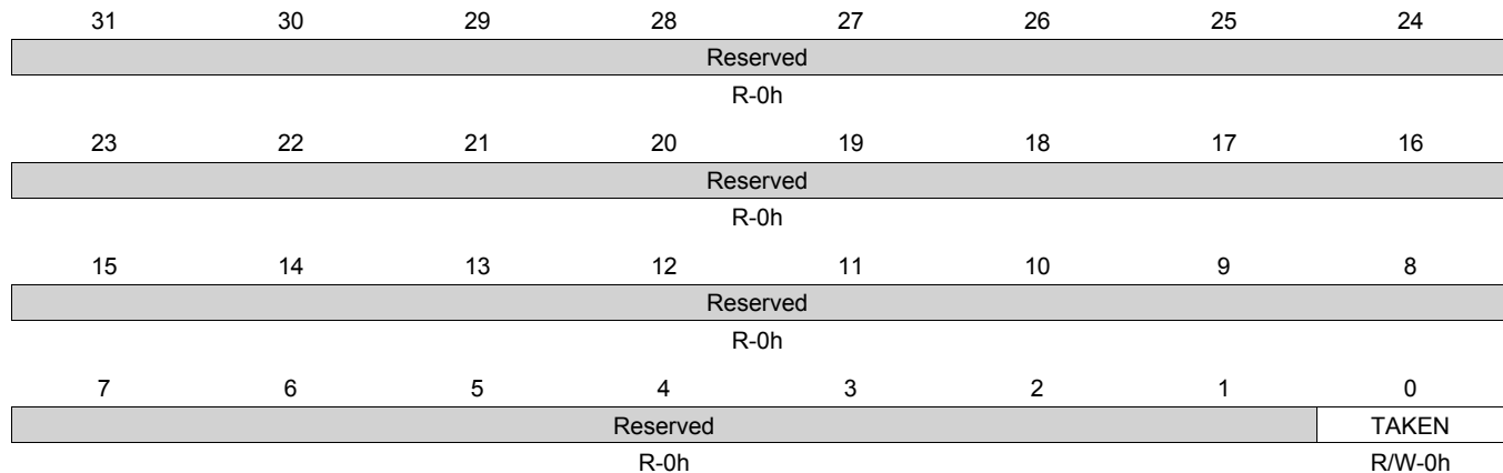
Figure 17-78. LOCK_REG_30 Register
