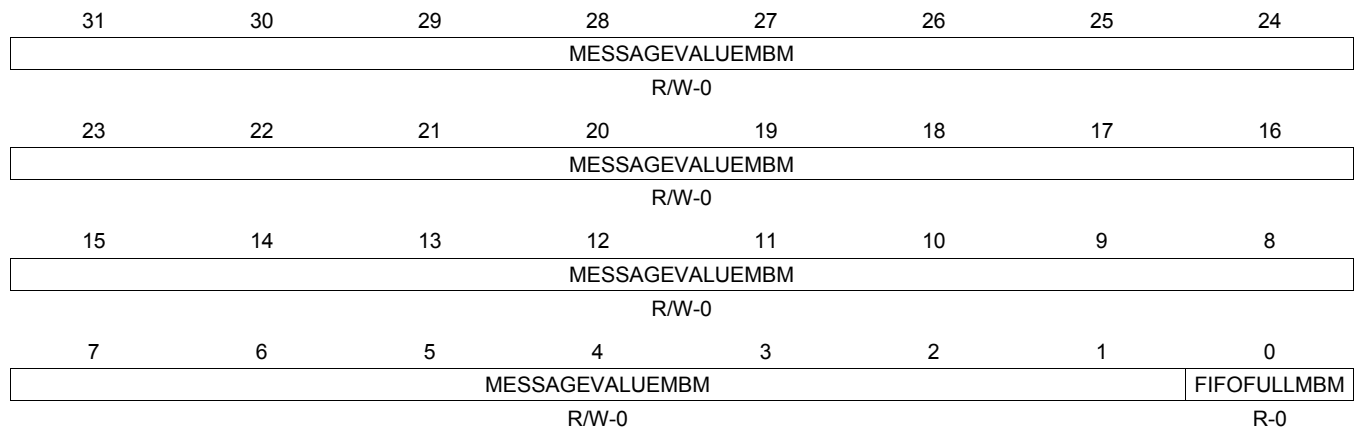
Figure 17-19. FIFOSTATUS_6 Register
