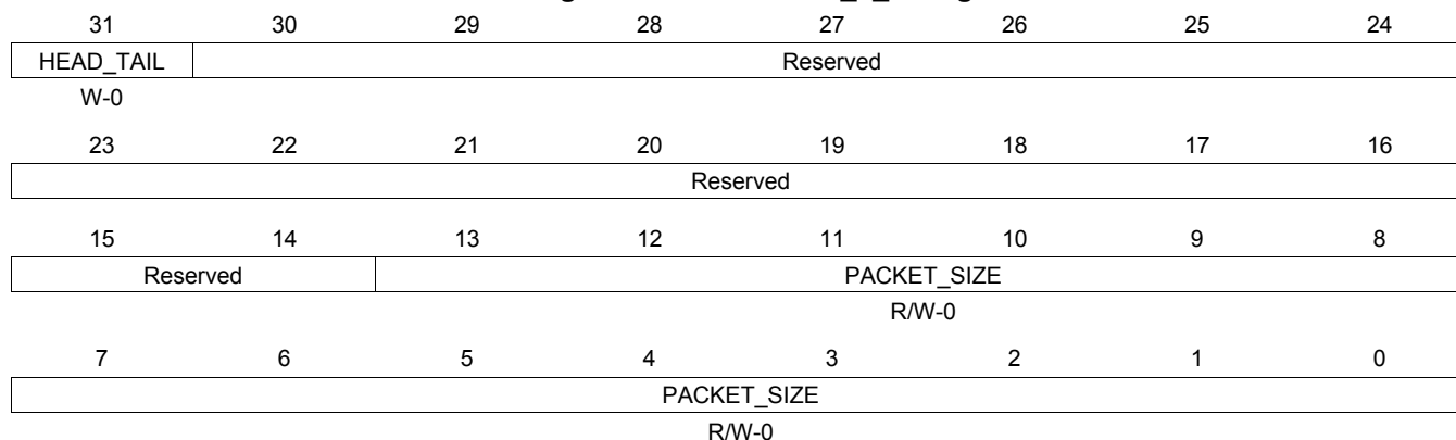
Figure 16-333. QUEUE_5_C Register
