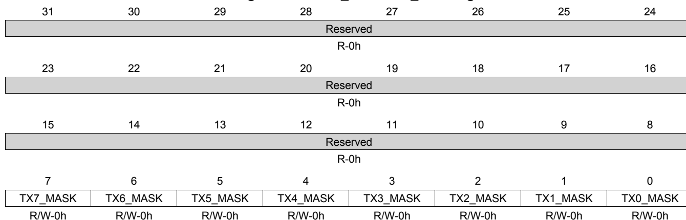
Figure 14-50. TX_INTMASK_SET Register
