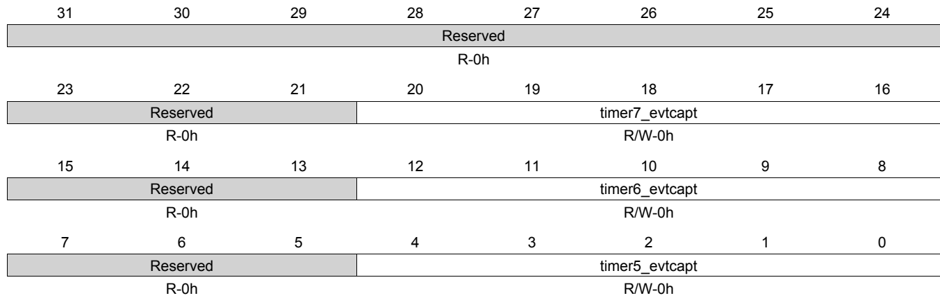
Figure 9-72. timer_evt_capt Register
