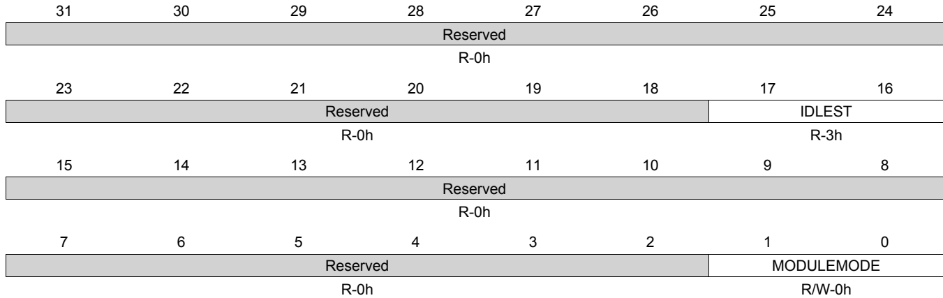
Figure 8-158. CM_GFX_MMUDATA_CLKCTRL Register
