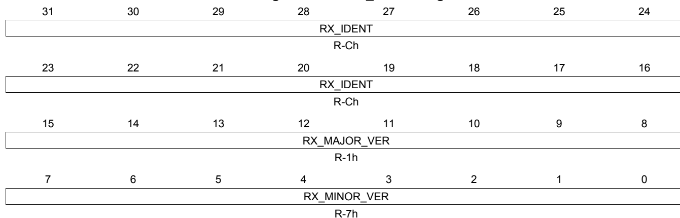
Figure 14-32. RX_IDVER Register
