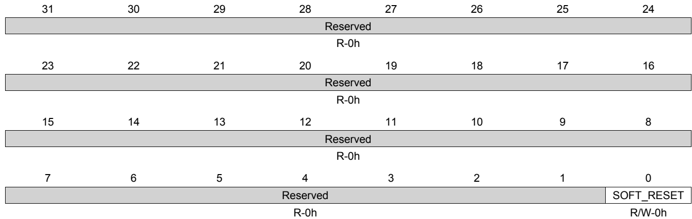
Figure 14-198. SOFT_RESET Register
