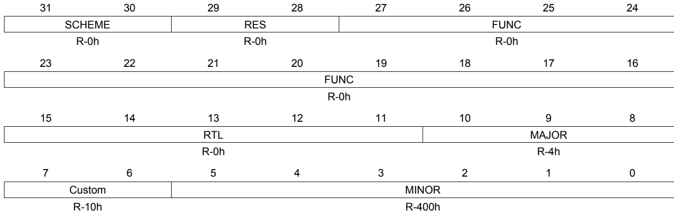
Figure 17-3. REVISION Register
