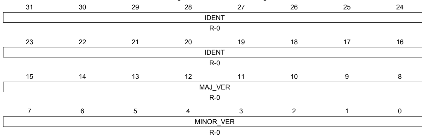
Figure 14-15. IDVER Register
