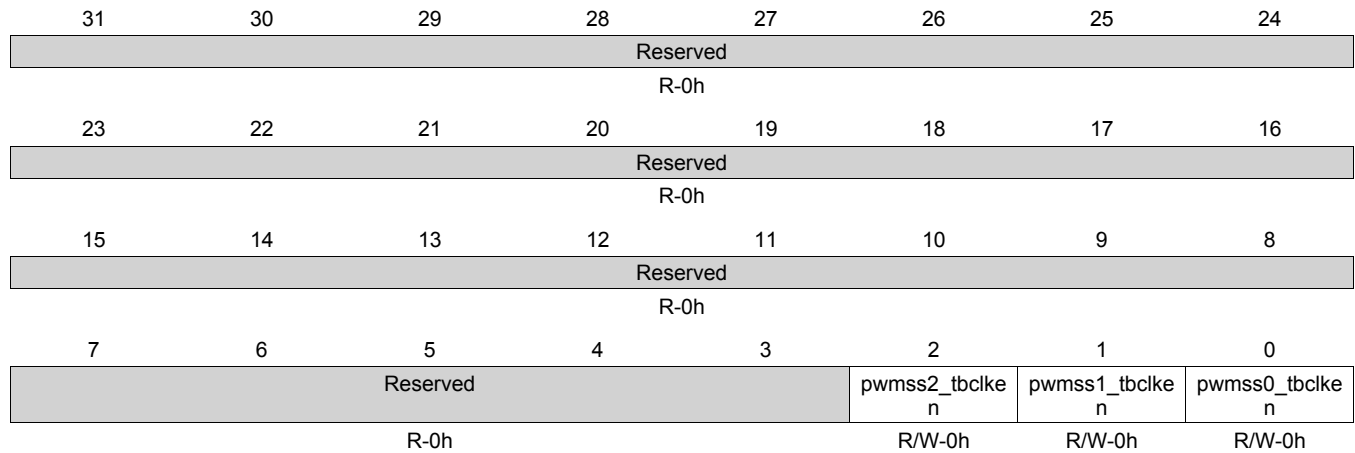
Figure 9-32. pwmss_ctrl Register
