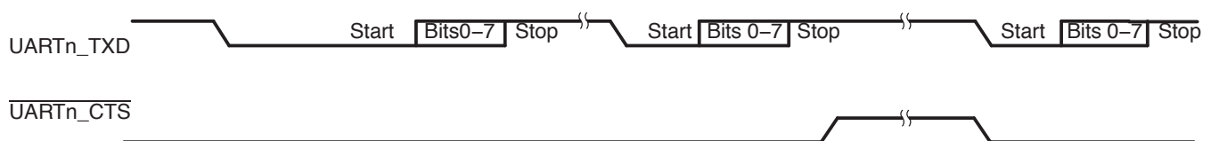
Figure 4-27. Autoflow Functional Timing Waveforms for \overline{\text{UARTn\_CTS}}
