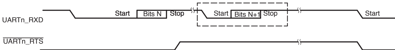
Figure 4-26. Autoflow Functional Timing Waveforms for \overline{\text{UARTn\_RTS}}
