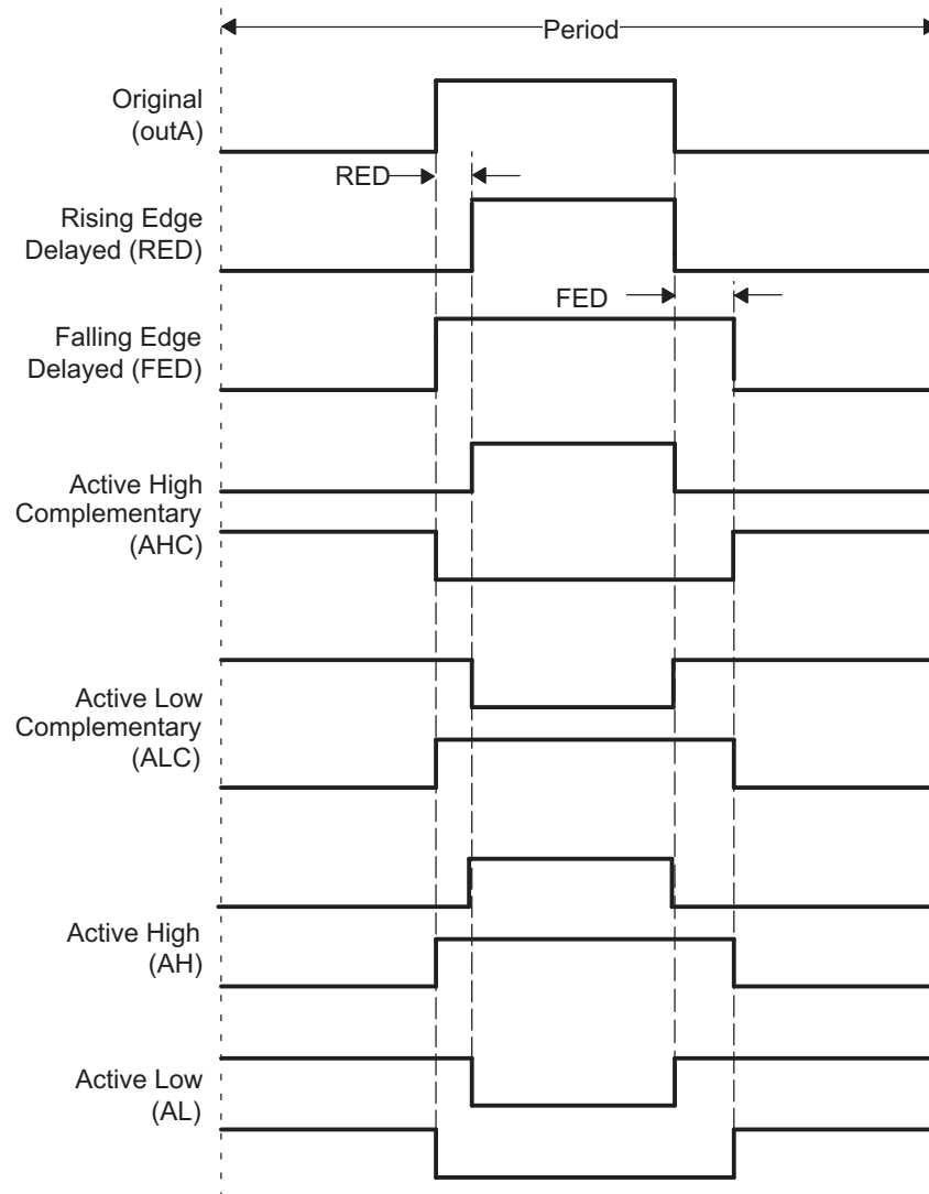
Figure 15-36. Dead-Band Waveforms for Typical Cases ( 0\% < \text{Duty} < 100\% )
