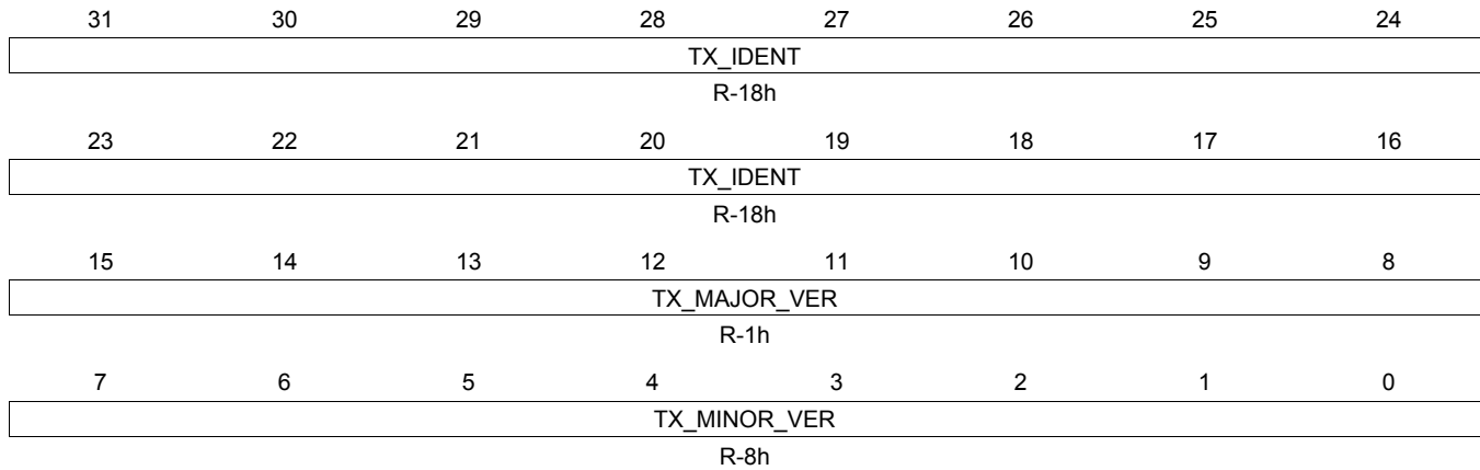
Figure 14-29. TX_IDVER Register
