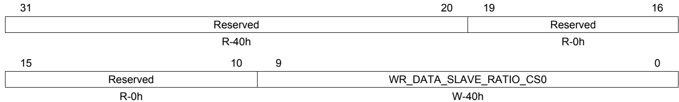
Figure 7-252. DDR PHY Data Macro 0/1 Write Data Slave Ratio Register (DATA0/1_REG_PHY_WR_DATA_SLAVE_RATIO_0)
