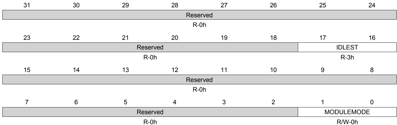
Figure 8-70. CM_PER_SPINLOCK_CLKCTRL Register
