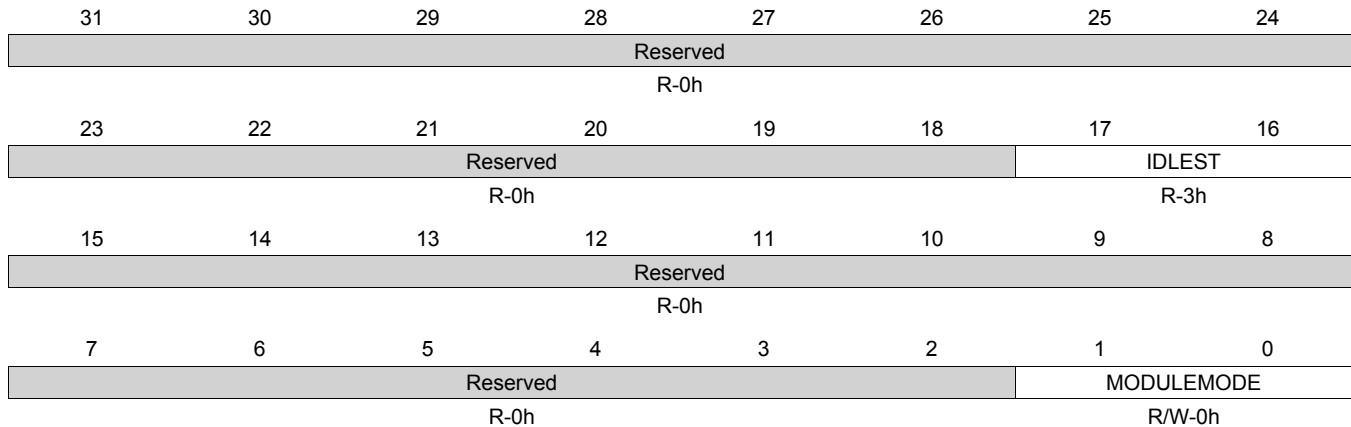
Figure 8-64. CM_PER_TIMER5_CLKCTRL Register
