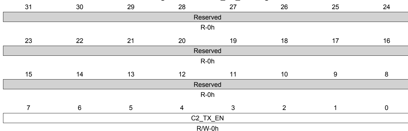
Figure 14-211. C2_TX_EN Register
