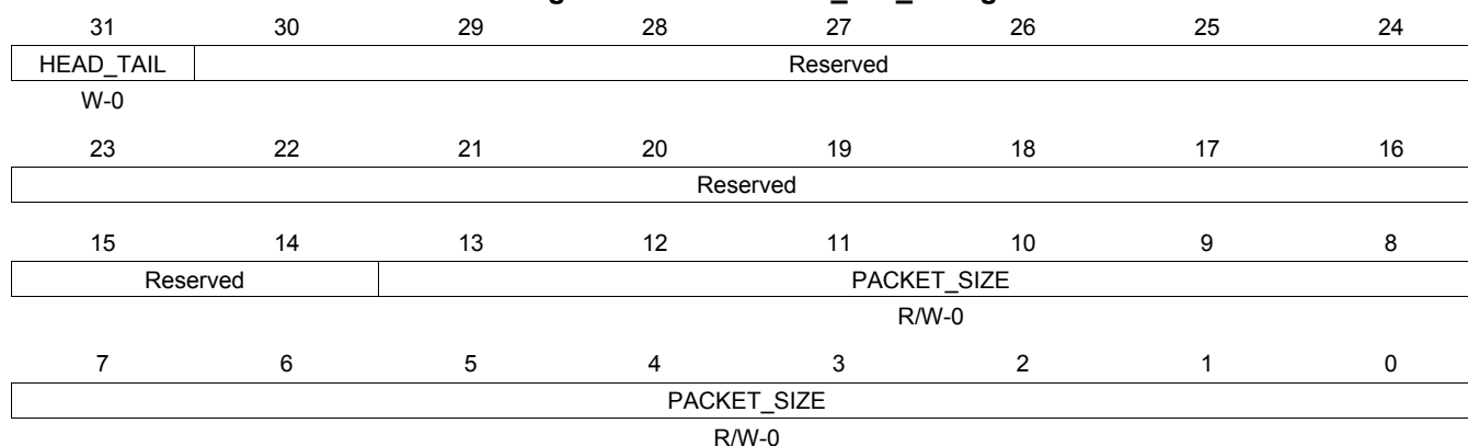
Figure 16-865. QUEUE_138_C Register
