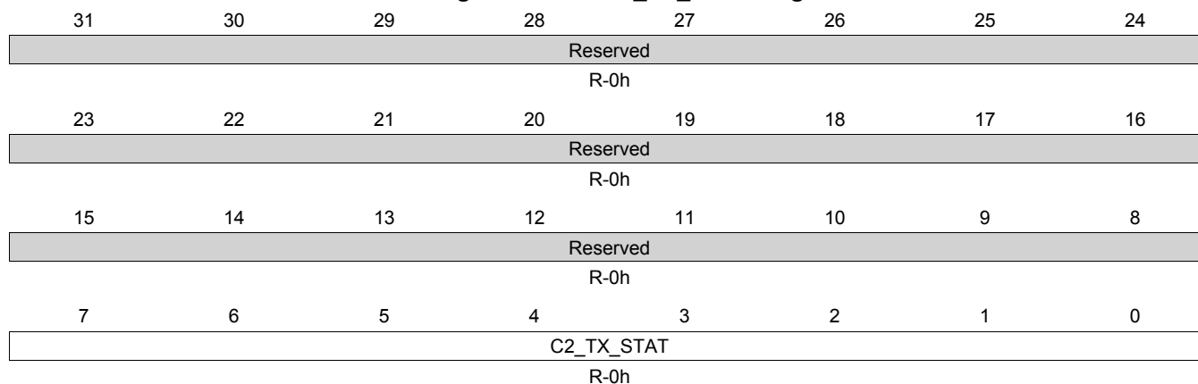
Figure 14-223. C2_TX_STAT Register
