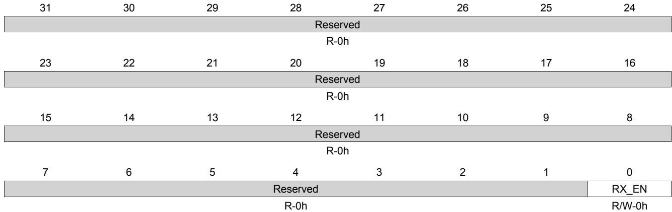
Figure 14-33. RX_CONTROL Register
