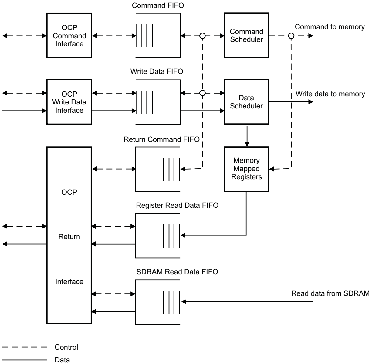
Figure 7-204. DDR2/3/mDDR Memory Controller FIFO Block Diagram
