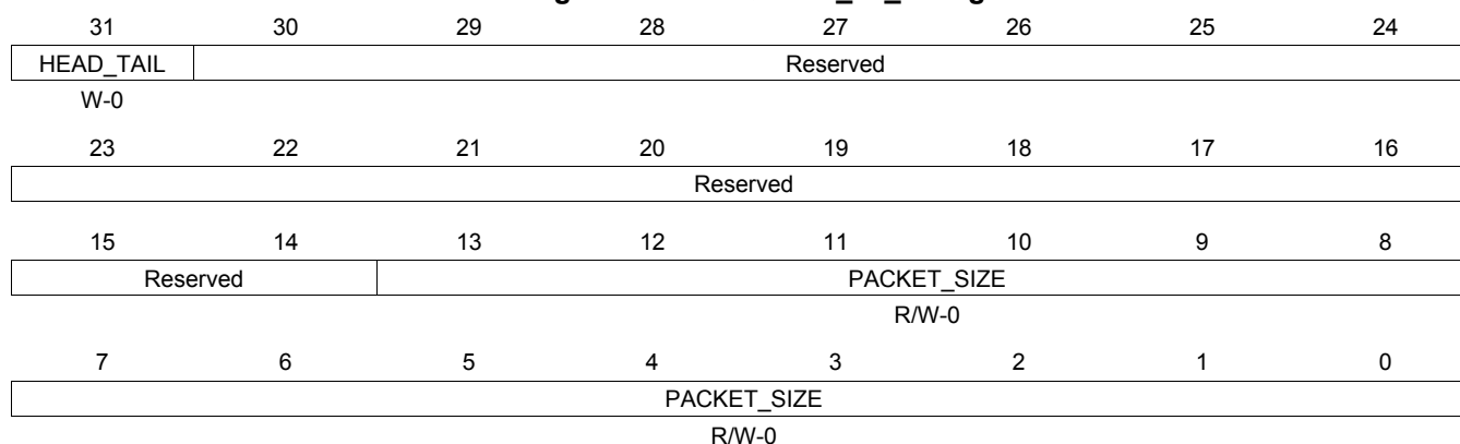
Figure 16-565. QUEUE_63_C Register
