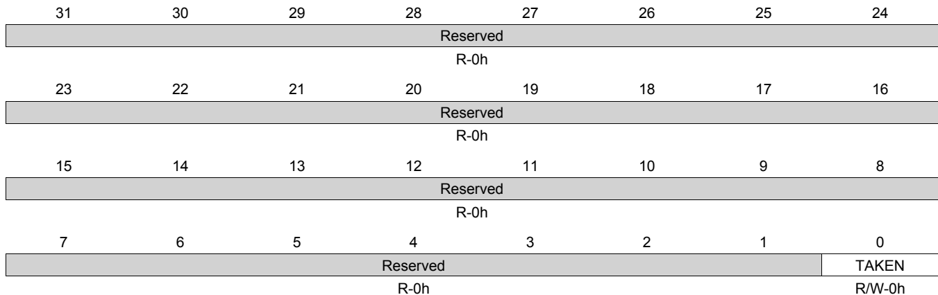
Figure 17-68. LOCK_REG_20 Register
