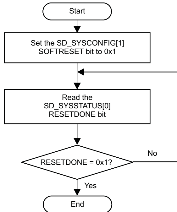
Figure 18-29. MMC/SD/SDIO Controller Software Reset Flow
