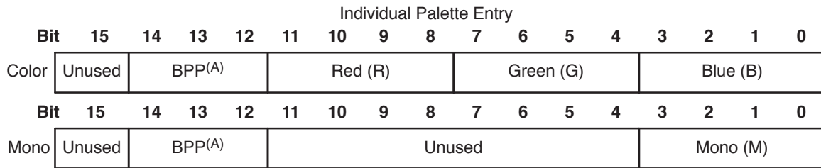
Figure 13-7. 256-Entry Palette/Buffer Format (8 BPP)
