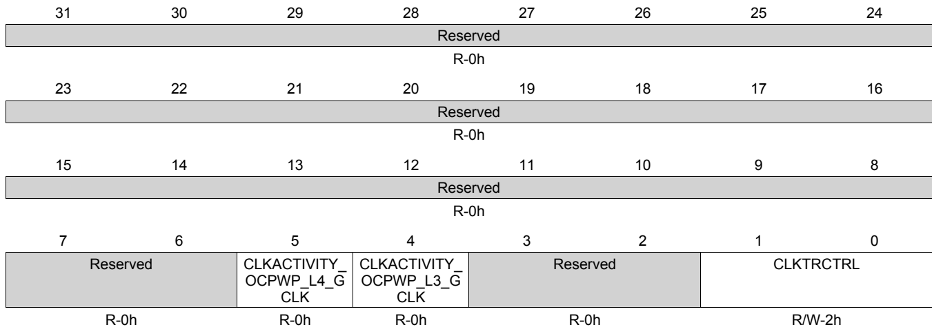
Figure 8-74. CM_PER_OCPWP_L3_CLKSTCTRL Register
