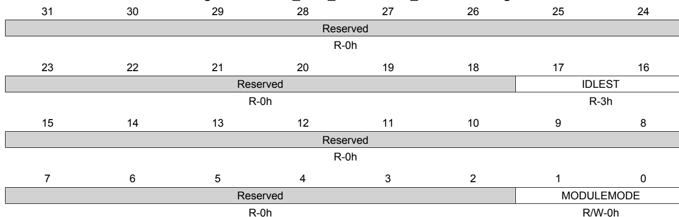
Figure 8-79. CM_PER_CLKDIV32K_CLKCTRL Register
