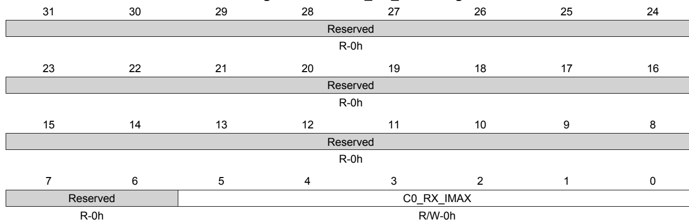
Figure 14-225. C0_RX_IMAX Register
