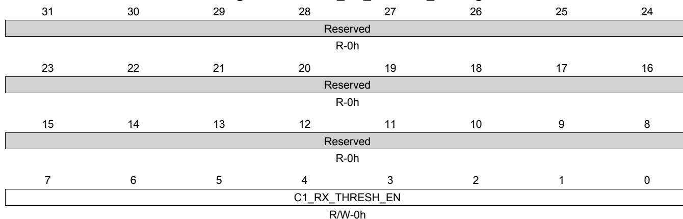
Figure 14-205. C1_RX_THRESH_EN Register
