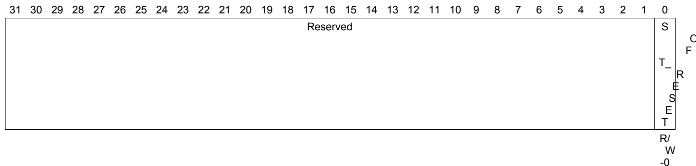
Figure 14-186. SOFT_RESET Register
