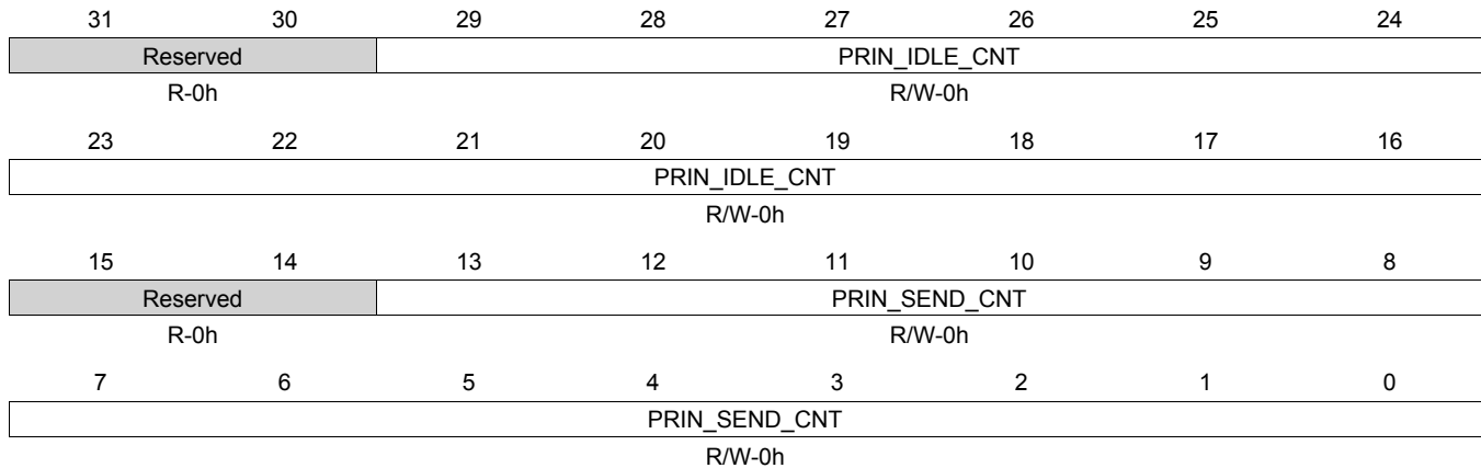
Figure 14-45. TX_PRI5_RATE Register
