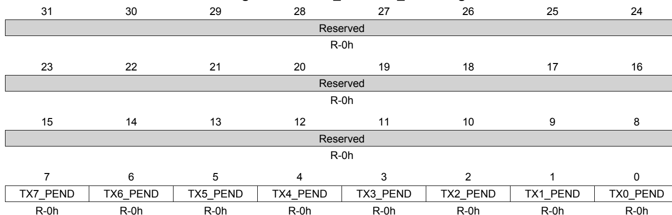
Figure 14-48. TX_INTSTAT_RAW Register
