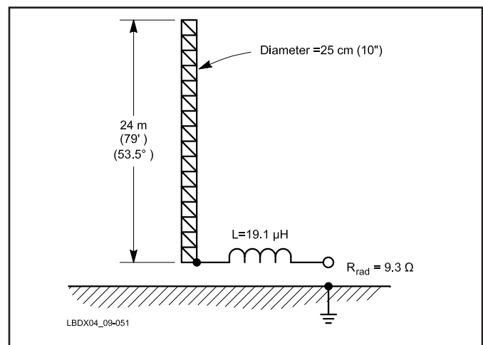
Fig 9-51—Base-loaded tower for 160 meters. See text for details on how to calculate the radiation resistance as well as the value of the loading coil. The loss resistance is effectively in series with the radiation resistance. With 60 \lambda/8 radials over good ground, the feed-point impedance will be approximately 20 \Omega and the radiation efficiency about 50%.
