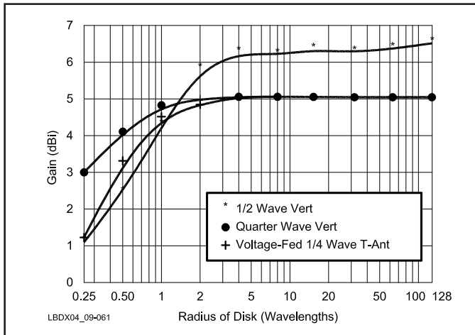
Fig 9-61—Gain of three types of verticals over a perfectly conducting disk of varying radius. The ground beyond the disk is of good quality. This means that the \lambda/2 vertical requires 0.6- \lambda radials to perform as well as the \lambda/4 vertical with \lambda/4 radials. Be aware that the radiation angle of the \lambda/2 vertical will be much lower, however.
