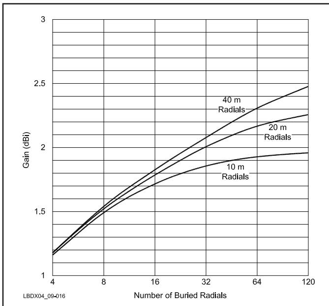
Fig 9-16 —Gain of \lambda/4 80-meter vertical over very good ground as a function of radial length and number of radials.
