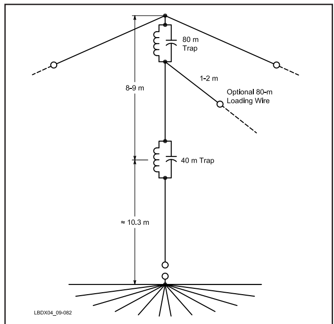
Fig 9-82 (below) —This version of the famous Battle Creek vertical is about 18 to 19 meters tall. If resonance on 80 cannot be achieved where wanted (if the support is not high enough), an 80-meter loading wire (typically 1 to 2 m long) can be added as shown. Slope this wire at right angle to the 40 and 160-meter loading wires if possible. The sloping angle of the 160-meter loading wire has a pronounced influence of the impedance of the antenna. You can use this to tune the antenna on 160. Keep the wire as horizontal as possible, however, it's better is to trim the length of the wire to tune it.
