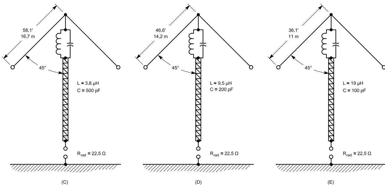
Fig 9-71—Evolution of a duoband trap-antenna design for 80 and 160 meters. For reference the equivalent 80 and 160-meter antennas without the trap are shown at A and B. Three trap configurations with discrete components (low, medium and high L/C ratios) are shown at C, D and E, while that at F uses a coaxial-cable trap. The four final designs show the matching networks for an equivalent ground resistance of 12 and 8 Ω respectively on 160 and 80 meters.
