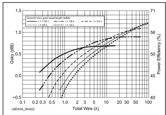
Fig 9-22—Total sky-gain results over very good ground for various radial systems using standard radials, shaped as the spokes of a wheel. The graph shows that with small amounts of wire, many short radials are the answer. It also tells us that 10 \lambda of radial wire used to make 80 \lambda/8 radials is only 0.2 dB down from 30 \lambda of radial wire used to make 120 \lambda/4 radials.
