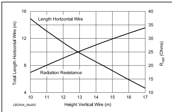
Fig 9-55—Design chart for a wire-type \lambda/4 current-fed T antenna made of 2-mm OD wire (AWG #12) for a design frequency of 3.5 MHz. For 160 meters the dimension should be multiplied by a factor of 1.9.
