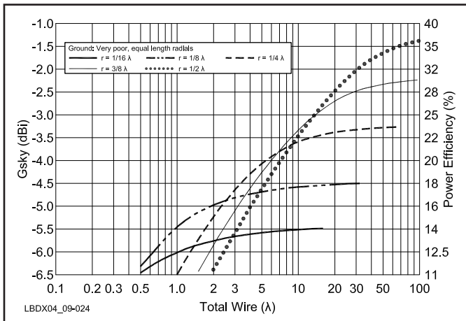
Fig 9-24—Have a look at the gain axis: No matter what you do (lots of \lambda/2 long radials), -1.3 dBi is the limit for very poor ground (as compared to 0 dBi for good ground and approximately +1.5 dB over very good ground). The nearly 3-dB difference is due to the Fresnel-zone reflection efficiency.
