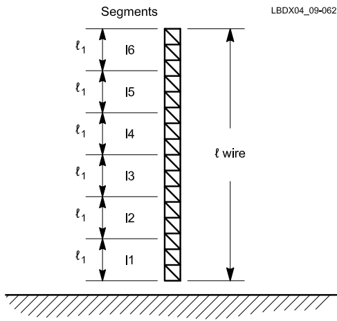
Fig 9-62— MININEC analysis of a straight 19-meter vertical antenna shown in the drawing. The analysis frequency is 3.8 MHz. MININEC impedance results are shown as a function of the number of segments in the table. Note that for reliability with a “fat” (200-mm) vertical, the maximum number of segments (in this case segments = pulses) is 70. The MININEC documentation states that the segment length should be greater than 2.5 times the wire diameter (2.5×200 mm = 500 mm). In this particular case errors occur when the segment length is smaller than the wire diameter.
