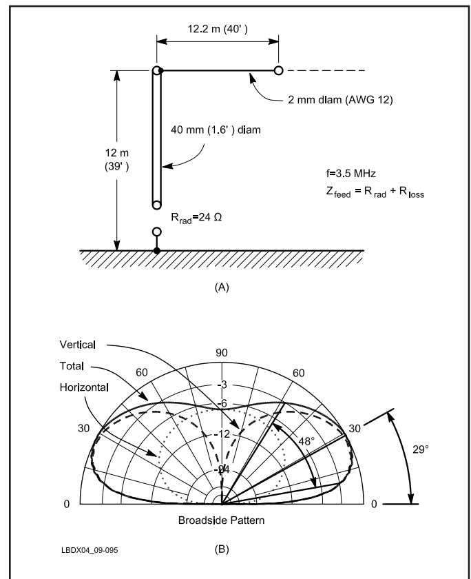
Fig 9-95—At A, a 3.5-MHz inverted L with a 12-meter vertical mast. The vertical radiation pattern is shown at B. The pattern has both vertically and horizontally polarized components and these components are also plotted at B. The pattern is generated over average ground, using 60 \lambda/4 radials. Note that the angle of maximum radiation is 29°, not bad for a DX antenna.
