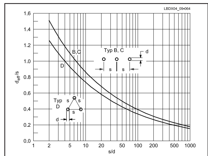
Fig 9-64—Normalized (round solid conductor) effective diameter of a triangular tower section as a function of the vertical tube diameter (d) and the tower width (s). The graph for three parallel conductors is also given (curve BC). (After Gerd Janzen, Kurze Antennen .)
