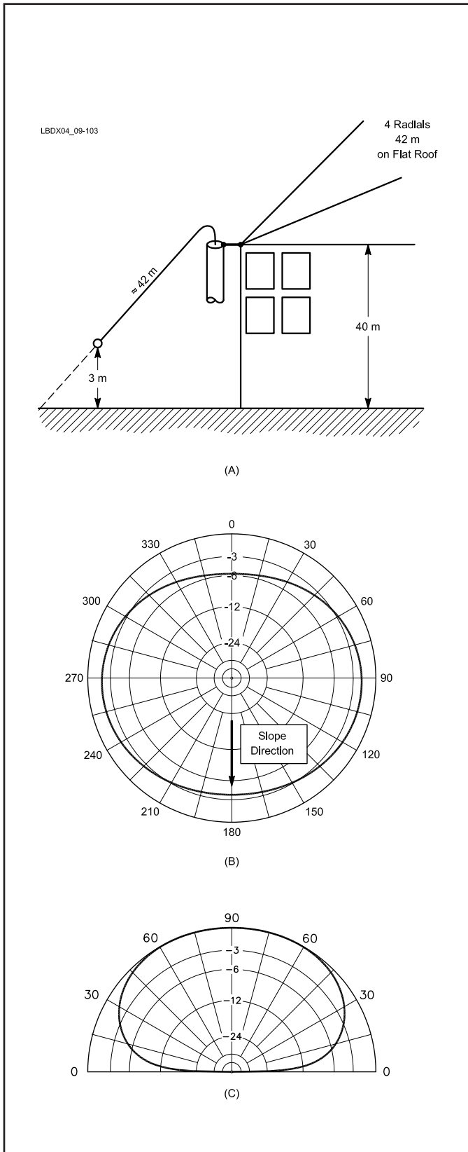
Fig 9-103—Configuration and radiation patterns of the inverted \lambda/4 sloper antenna used by 9M2AX. The azimuth pattern is shown at B for an elevation angle of 30°, and at C is the elevation pattern. (The elevation pattern is taken in the 90-270° direction as displayed in the azimuth pattern.) Note the relative high amount of high-angle radiation. Using just two radials in-line would improve this situation considerably.
