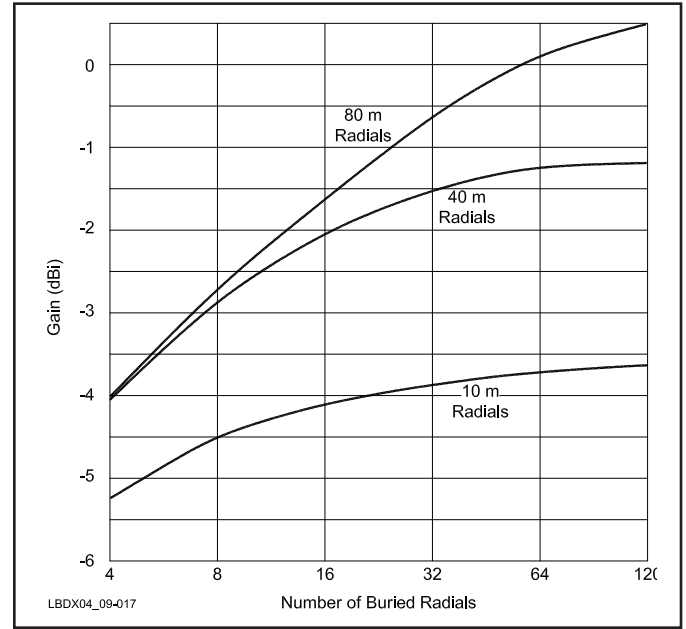
Fig 9-17 —Gain of \lambda/4 160-meter vertical over very poor ground as a function of radial length and number of radials. Note that 10-meter radials, no matter how many, are really too short for 160 meters.
