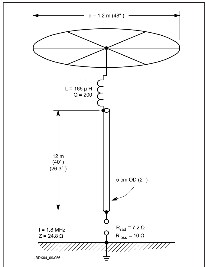
Fig 9-56—Top-loaded vertical for 160 meters, using a combination of a capacitance hat and a loading coil. See text for details.
