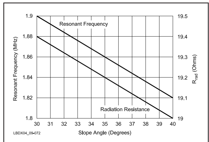
Fig 9-72—This chart shows the variation in resonant frequency and radiation resistance for a 27-meter vertical with 19-meter long sloping top-load wires. A change in slope angle of 30^\circ to 40^\circ shifts the resonant frequency by 80 kHz.
