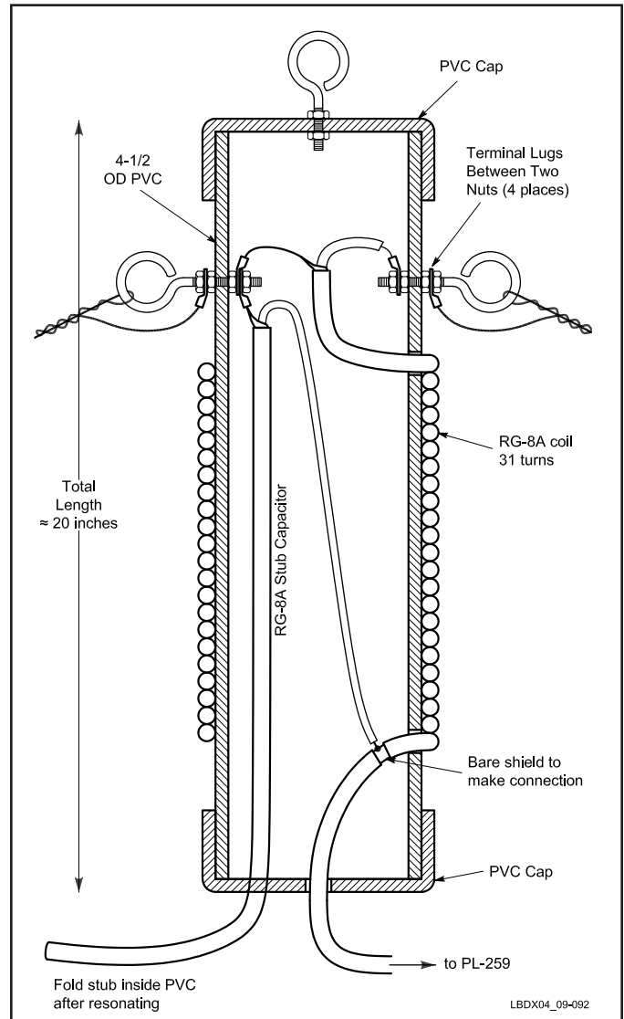
Fig 9-92—Construction details of the K9RJ decoupling trap.
