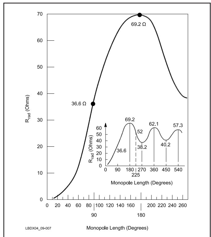
Fig 9-7 —Radiation resistances ( R_{rad(I)} , at the current maximum) of monopoles with sinusoidal current distribution. The chart can also be used for dipoles, but all values must be doubled.
