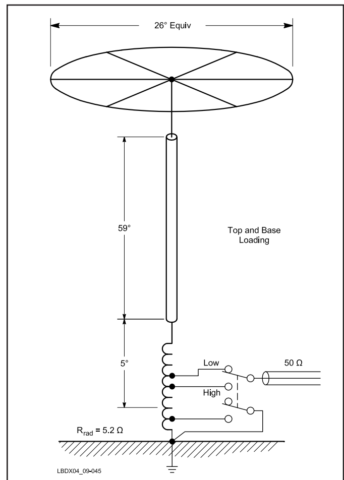
Fig 9-45—Instead of series-feeding the antenna, we can look for a tap on the coil that gives 50 \Omega . The coil serves two purposes: Some base loading and also impedance matching. Using a DPDT relay you could make provisions for a perfect 50\text{-}\Omega match on two frequencies; eg, on CW and on phone.
