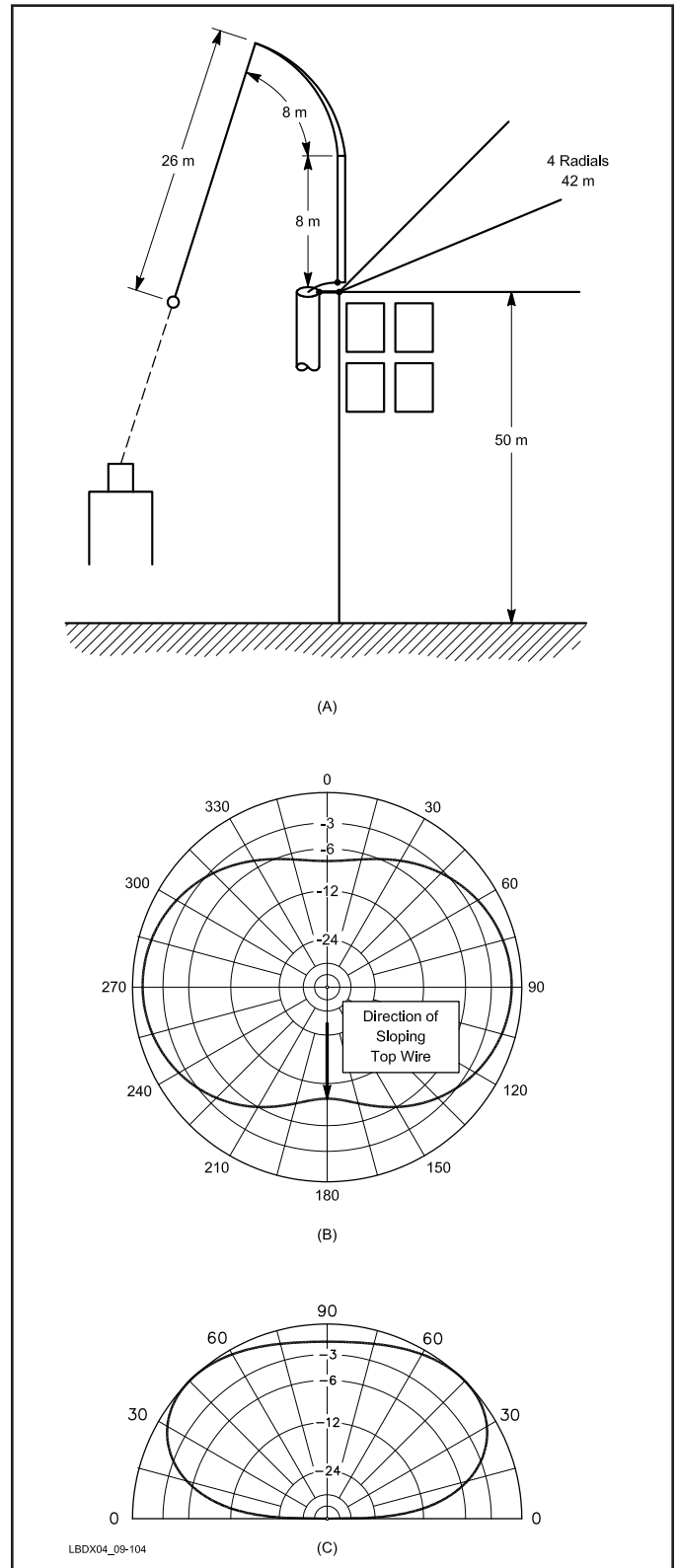
Fig 9-104—Configuration and radiation patterns of the inverted \lambda/4 sloper antenna used by 9M2AX during his expedition from East Malaysia (Sarawak) as 9M8AX. The azimuth pattern is shown at B, and the elevation pattern at C. (The elevation pattern is taken in the 90-270° direction as displayed in the azimuth pattern.) The antenna was installed on the edge of a 50-meter high flat roof. Four \lambda/4 long radials were laid on the roof. The metal mast plus the fiberglass rod are 16 meters long. The sloping wire was adjusted for minimum SWR at resonance.
