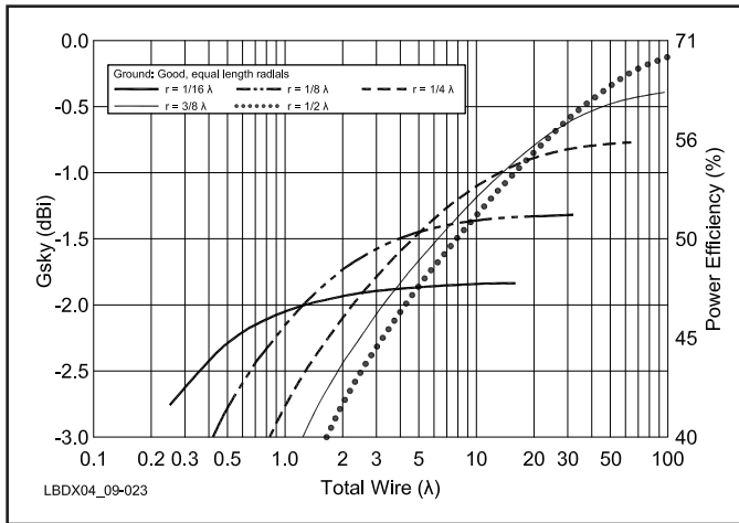
Fig 9-23—The same graph as in Fig 9-22 but for good ground. Unless you only have 4 \lambda of wire, \lambda/8 radials are really too short; \lambda/4 radials are just fine for up to about 20 \lambda of wire (this about 3.3 km or 10,000 ft of radials on 160 meters). Notice that this study also shows that there is little to be gained beyond approximately 100 \lambda/4 radials. 300 \lambda/2 radials only gain about 0.7 dB (a power increase of only 20%) over 100 \lambda/4 radials—not really a whole lot!
