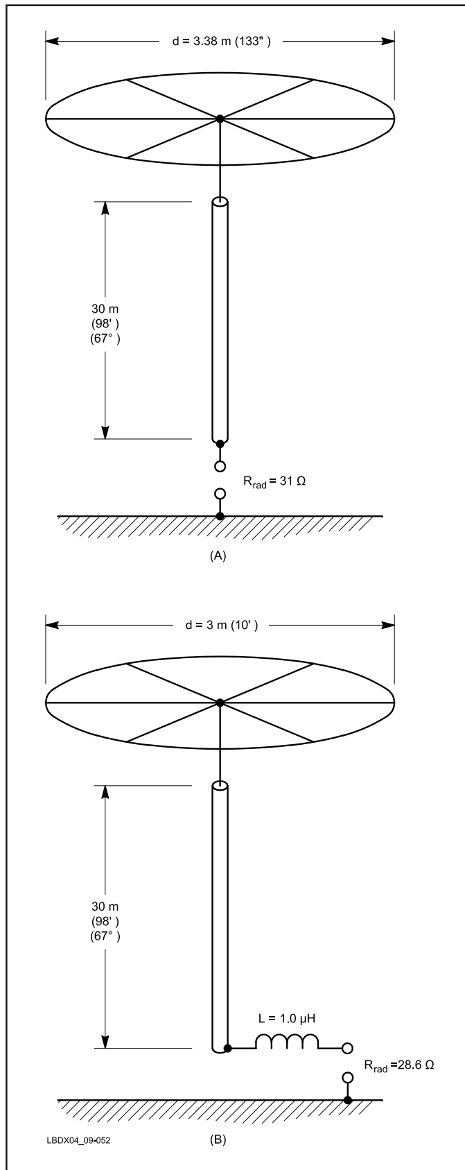
Fig 9-52—Examples of 160-meter verticals using capacitance hats. At A, the hat is dimensioned to tune the vertical to resonance at 1830 kHz. The antenna at B uses a capacitance hat of a given dimension, and resonance is achieved by using a small amount of base loading.
