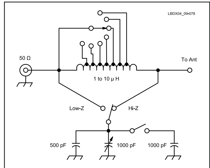
Fig 9-78 —L network to be used with Inverted-L antennas and other loaded 160-meter verticals. With the component values shown, impedances in the range 20 - j 100 to 100 + j 100 \Omega can easily be matched on 160 meters.
