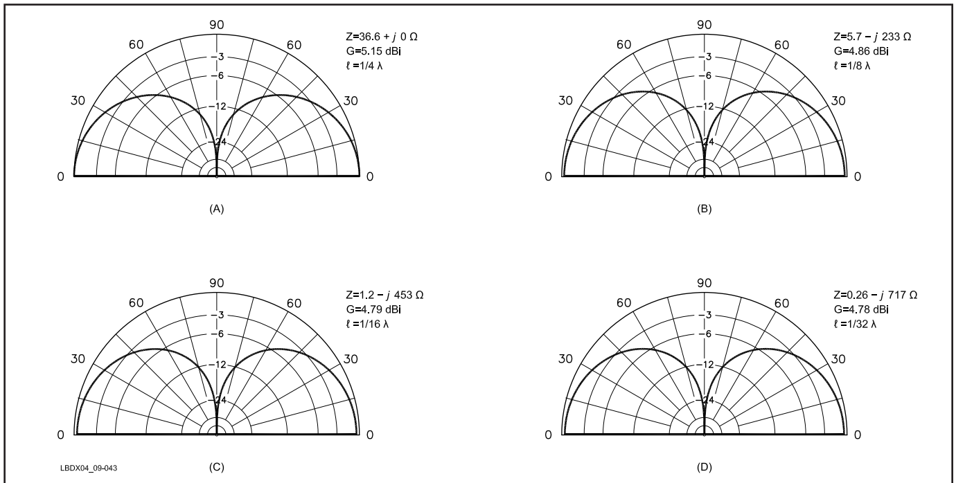
Fig 9-43—Elevation-plane radiation patterns and gain in dBi of verticals with different heights. The 0-dB reference for all patterns is 5.2 dBi. Note that the gain as well as the shape of the radiation patterns remain practically unchanged with height differences. The patterns were calculated with ELNEC over perfect ground, using a modeling frequency of 3.5 MHz and a conductor diameter of 2 mm. At A, height = \lambda/4 . At B, height = \lambda/8 . At C, height = \lambda/16 . At D, height = \lambda/32 .
