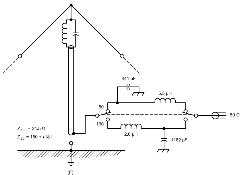
Fig 9-71—Evolution of a duoband trap-antenna design for 80 and 160 meters. For reference the equivalent 80 and 160-meter antennas without the trap are shown at A and B. Three trap configurations with discrete components (low, medium and high L/C ratios) are shown at C, D and E, while that at F uses a coaxial-cable trap. The four final designs show the matching networks for an equivalent ground resistance of 12 and 8 Ω respectively on 160 and 80 meters.
