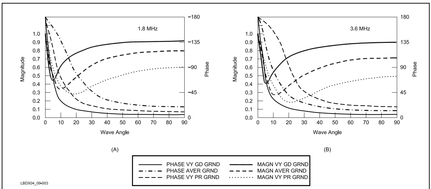
Fig 9-3—Reflection coefficient (magnitude and phase) for vertically polarized waves over three different types of ground (very good, average, and very poor).
