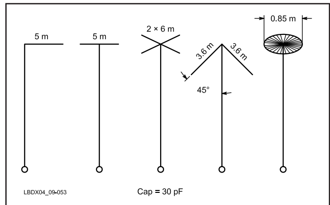
Fig 9-53—Capacitance hats can have various shapes, such as a disk, one or two wires, forming an inverted L or a T with the vertical. The lengths indicated are approximate values for a capacity of 30 pF.
