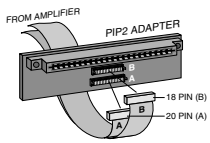
Fig. 8.1 PIP2 Adaptor Connection
