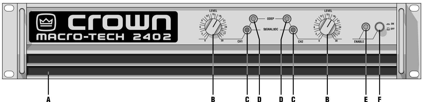
Fig. 2.1 Front Panel Controls &amp; Indicators
