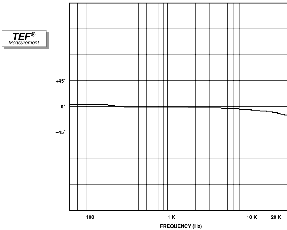
Fig. 6.10 Typical Phase Response
