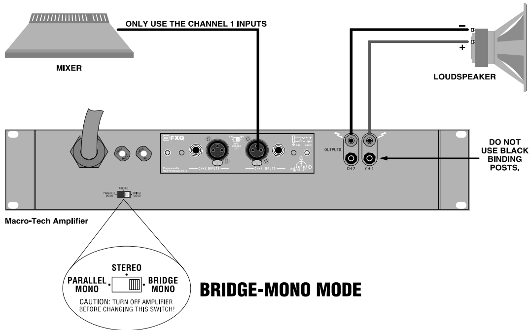
Fig. 3.5 Bridge-Mono Wiring
