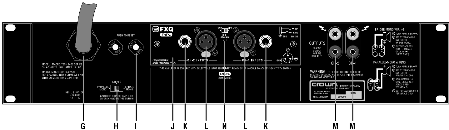
Fig. 2.2 Rear Panel Controls & Connectors (Note: Reset Switches (Item I) only available on the Macro-Tech 2402 model.)
