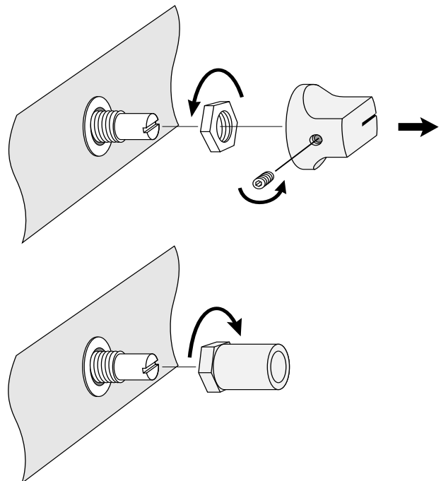
Fig. 8.4 Installing a Level Control Shaft Lock
