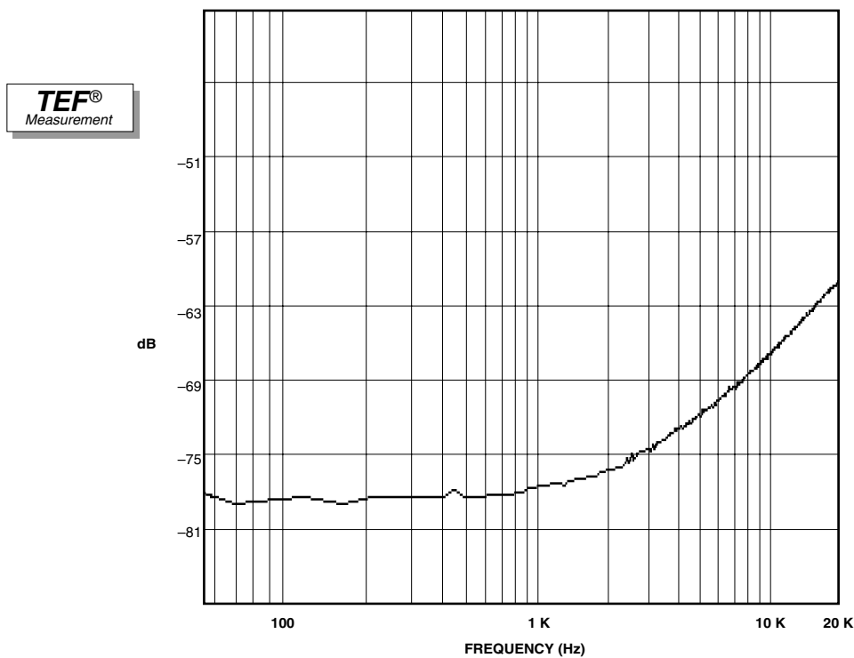
Fig. 6.11 Typical Crosstalk for the Macro-Tech 602
