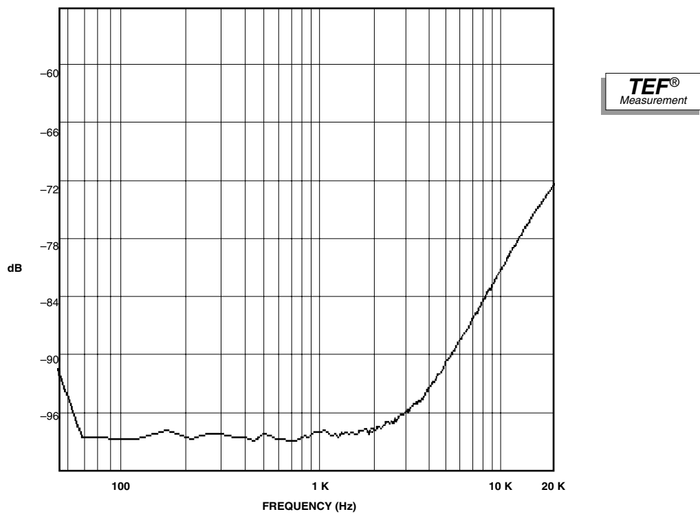
Fig. 6.13 Typical Crosstalk for the Macro-Tech 2402
