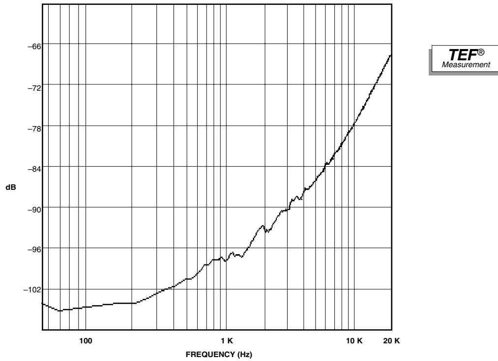
Fig. 6.12 Typical Crosstalk for the Macro-Tech 1202
