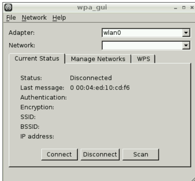
Figure 9-6. wpa_gui window
