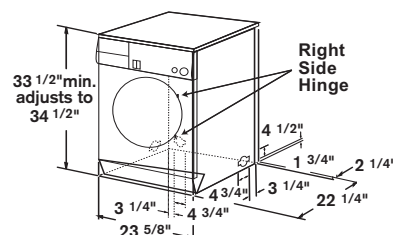
Dimensions for WTA4400US and CN (Vented)
