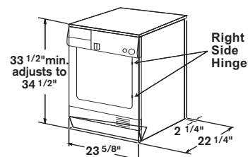
Dimensions for WTL5410UC (Condensation — no ducting required)
