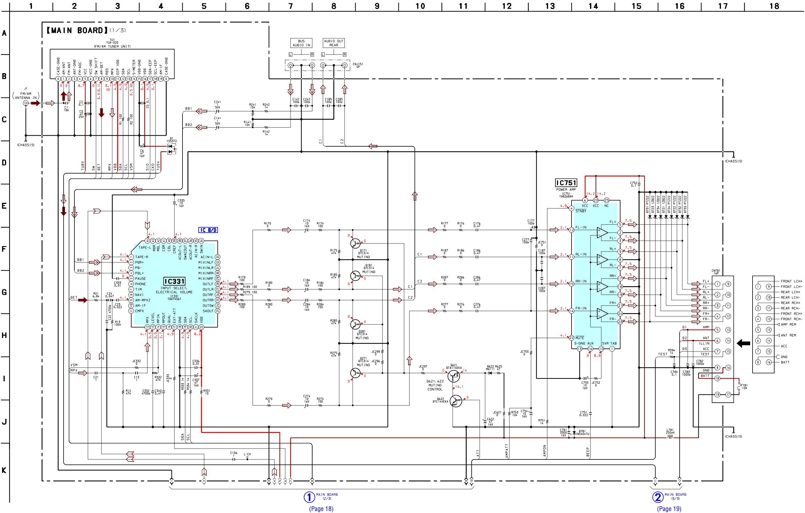
6-3. SCHEMATIC DIAGRAM – MAIN Board (1/3) – • See page 21 for IC Block Diagram.
