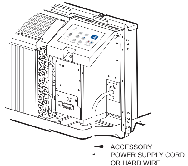
Figure 26 Power Connection
