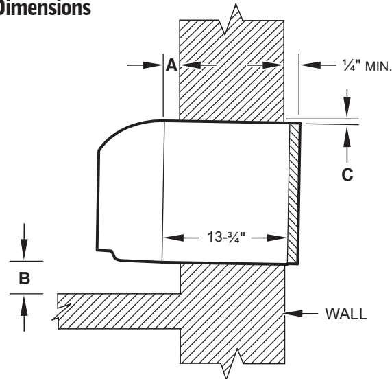
Figure 9 Dimensions
