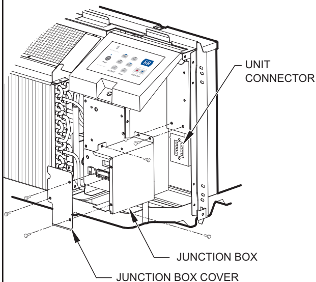
Figure 25 Junction Box Location
