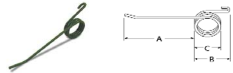
A-257SE Rake tooth
