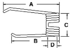
A-4100302080 Tedder Tooth (LH)
