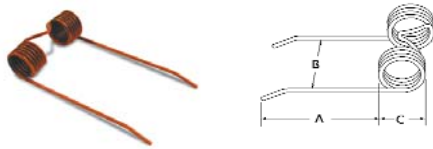
A-MA74528 Baler tooth
