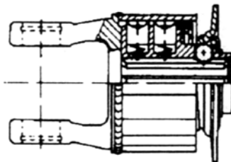
Radial Pin Clutch
