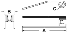
A-58505210 Hay tedder tooth
