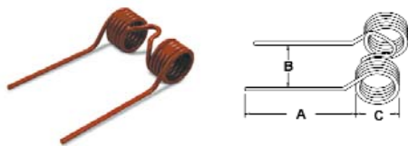
A-7751621 Tedder tooth
