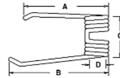
A-4101101390 Tedder Tooth (RH)
