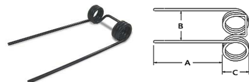
A-76-156 Harrow Tooth
