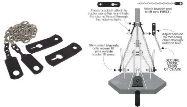
A-159335 Mower Deck Height Stabilizer Kit Contains 2 Chains With Brackets MISCELLANEOUS applications
