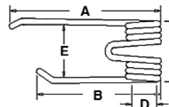
A-4101601590 Tedder Tooth (LH)
