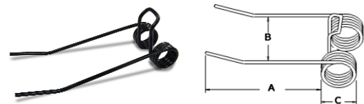
A-TEO01236 Rake tooth
