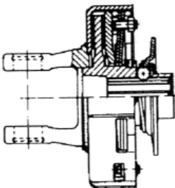
Friction Clutch
