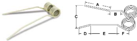
A-PZ110 Tedder Tooth
