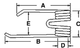
A-4101601490 Tedder Tooth (RH)
