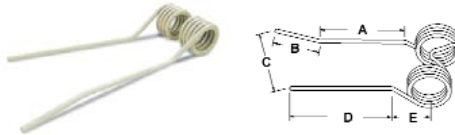
A-PZ111 Tedder Tooth
