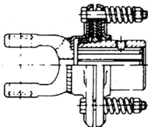
Adjustable Friction Clutch
