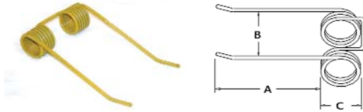
A-128102 Baler tooth
