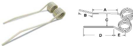
A-51001286 Tedder Tooth
