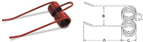
A-7893746 Baler tooth
