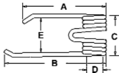
A-4101701380 Tedder Tooth (RH)
