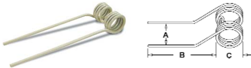
A-57609000 Tedder tooth
