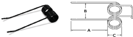
A-210614C1 Baler tooth
