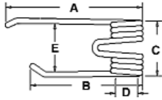
A-4101701260 Tedder Tooth (LH)
