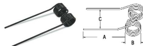
A-665930M1 Baler tooth
