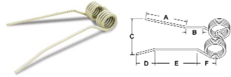
A-PZ110 Tedder tooth
