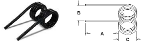
A-96LL2 Peanut Combine tooth
