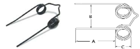
A-146545 Rake tooth
