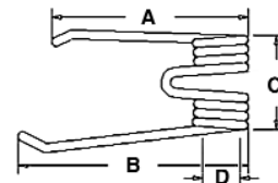
A-4101500680 Tedder Tooth
