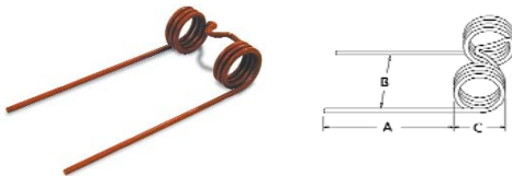
A-290141 Rake Tooth
