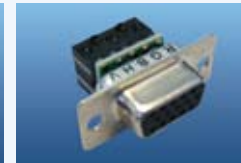
Part #: PC-V66 HD-15 Female to Screw Terminal (use 25-30 AWG)
