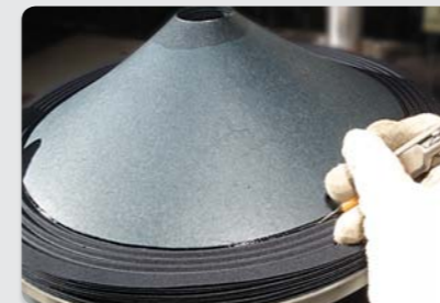
Cone/surround attachment process
