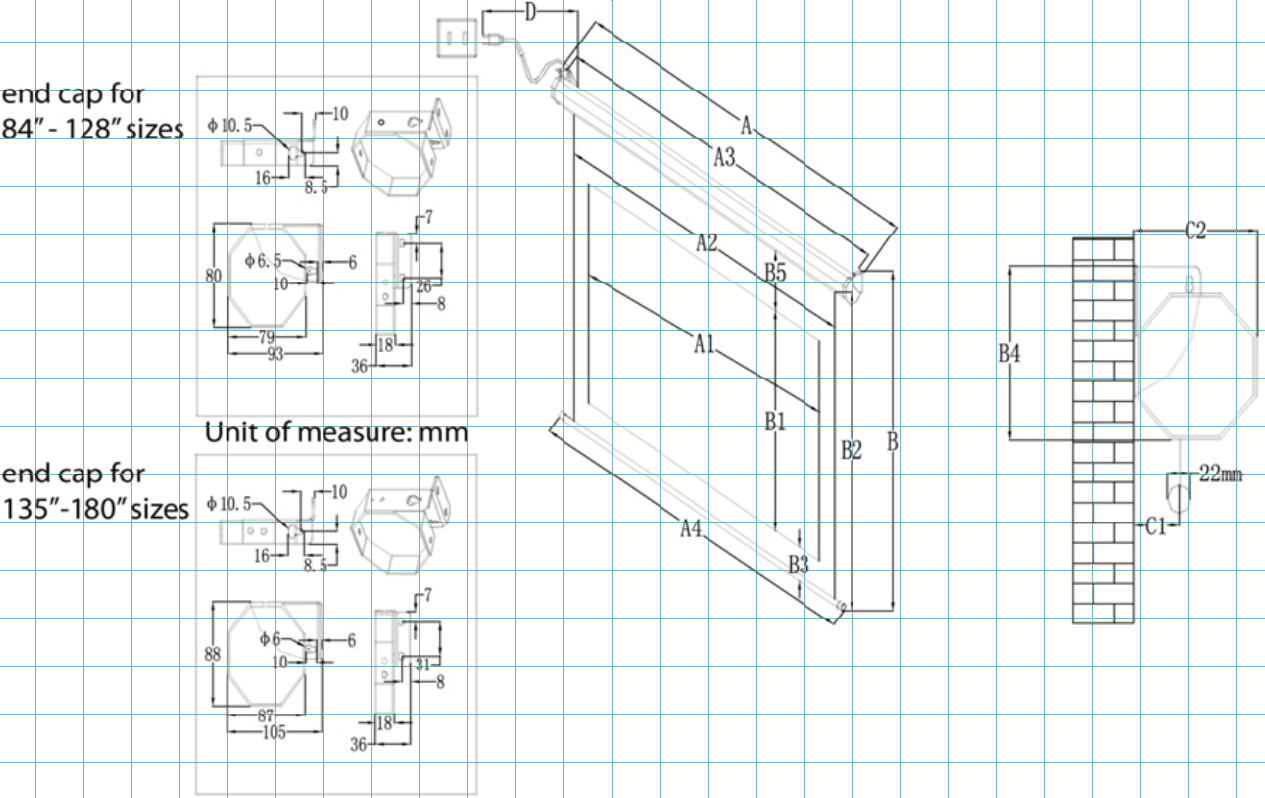
VMAX2 Series Dimensions Table (200" and above)
