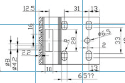
Wall/Ceiling Brackets Unit of measure: mm
