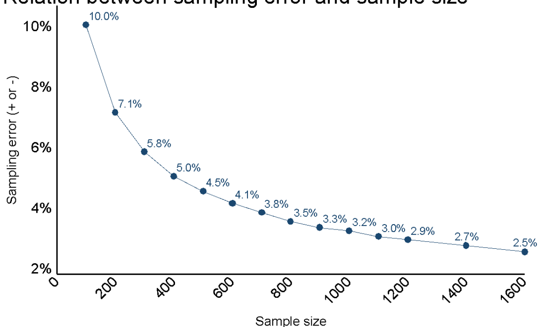
Relation between sampling error and sample size
