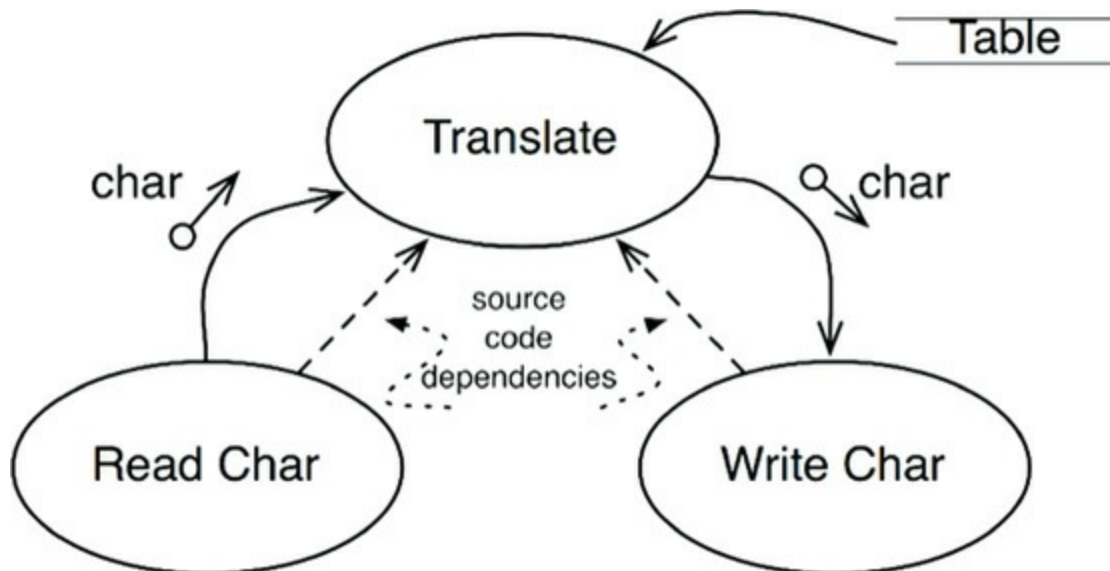
Figure 19.1 A simple encryption program
