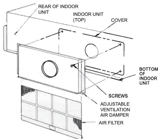
Fig. 2 – Fresh Air Intake Kit
