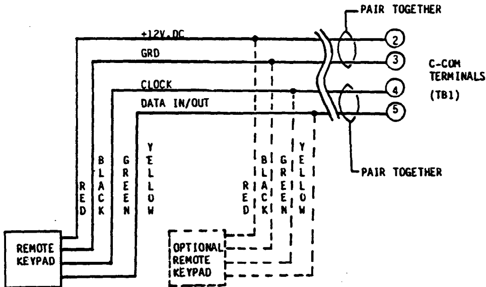
Diagram 2: KEYPAD CONNECTIONS
