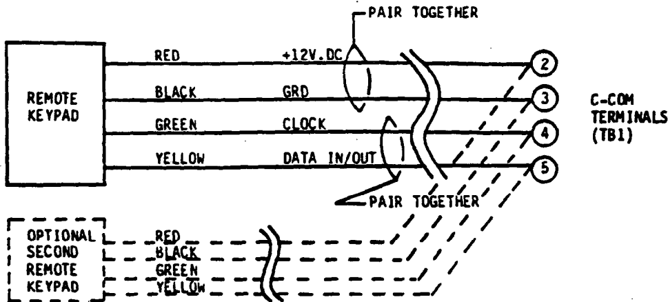
Diagram 1: KEYPAD CONNECTIONS
