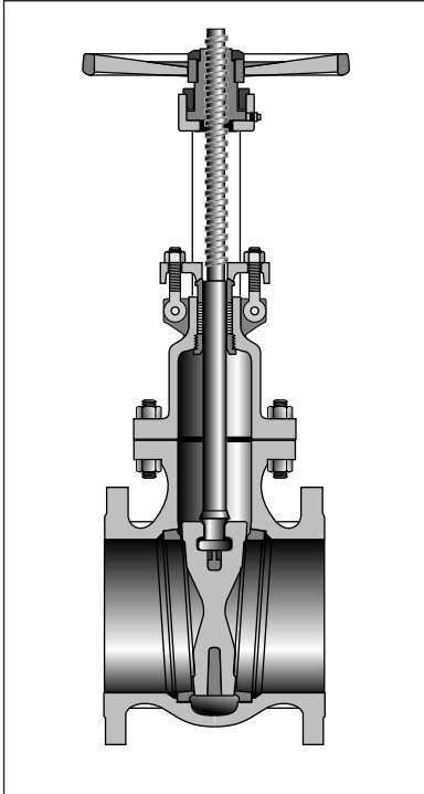
Figure 47XU-F Flanged
