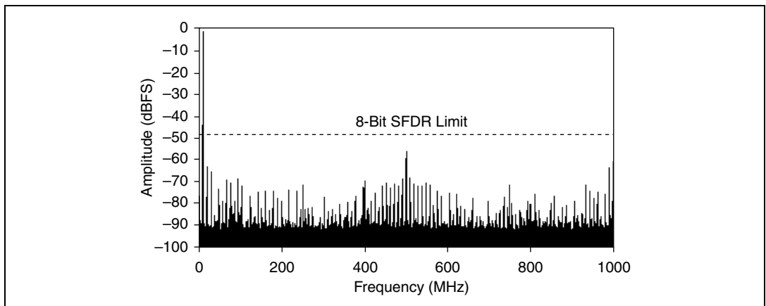
Figure 6. NI 5152 TIS Typical Dynamic Performance, 50 \Omega , 1 V pk-pk Range, 9.425 MHz, -1 dBFS Input Signal
