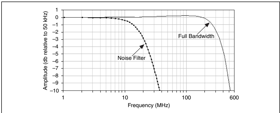
Figure 1. NI 5152 Frequency Response, 50 \Omega , 1 V (Typical)
