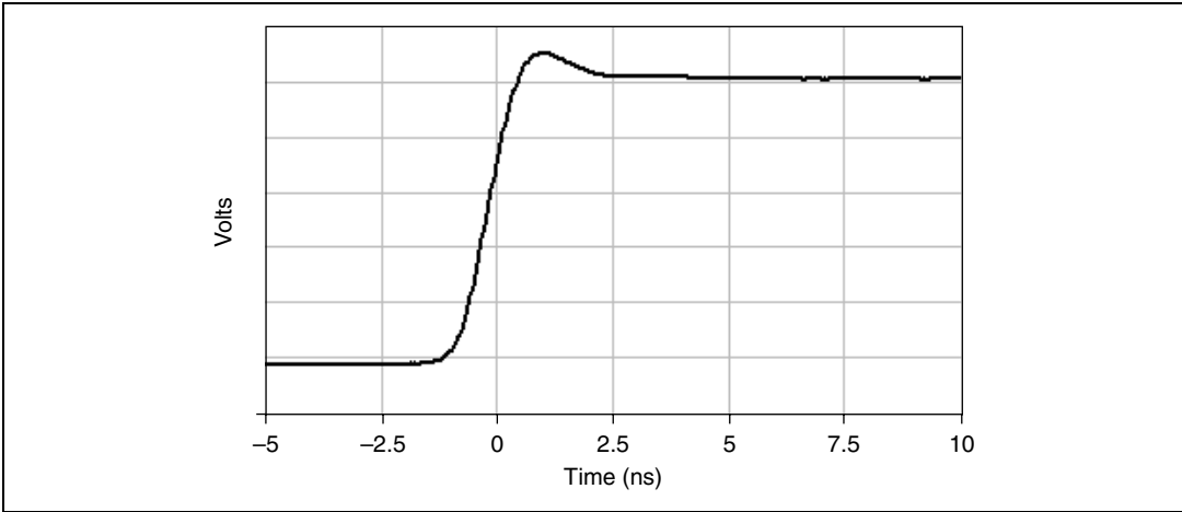
Figure 3. NI 5152 Step Response, 50 \Omega , 10 V_{pk-pk} through 0.2 V_{pk-pk} Range, Typical
