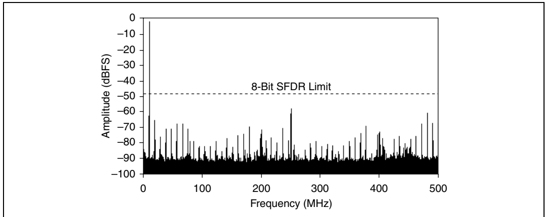
Figure 5. NI 5152 Typical Dynamic Performance, 50 \Omega , 1 V pk-pk Range, 9.425 MHz, -1 dBFS Input Signal
