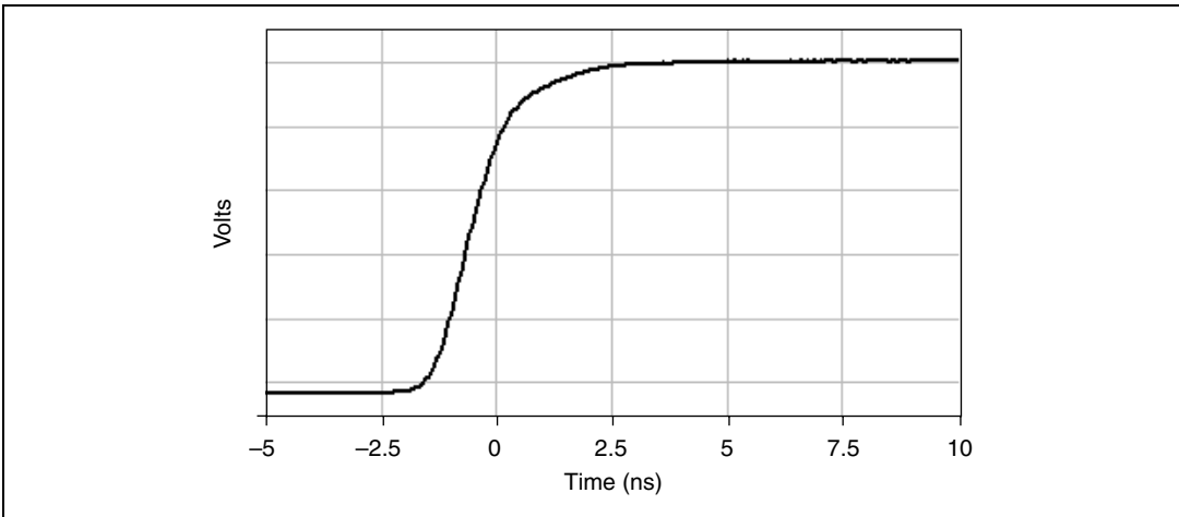
Figure 4. NI 5152 Step Response, 50 \Omega , 0.1 V_{pk-pk} Range, Typical
