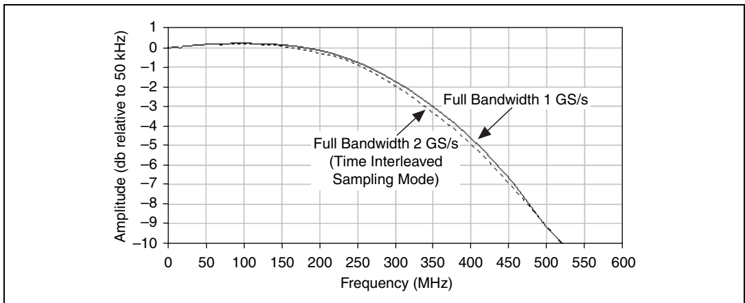
Figure 2. NI 5152 Frequency Response, 50 \Omega , 1 V (Typical)
