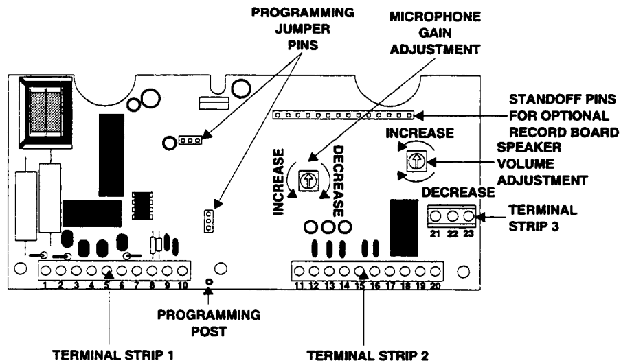
Figure 1.1. Interrogator Components
