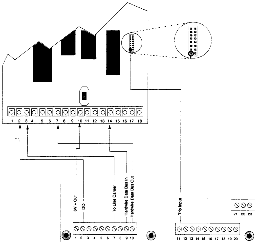
Figure 2.6 SX-V to Interrogator Wiring Diagram
