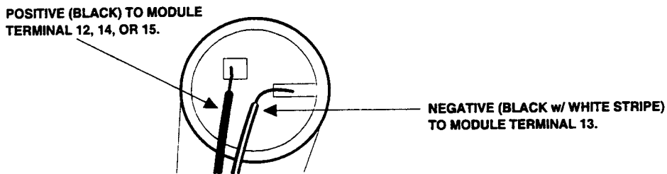
Figure 2.13 Speaker Cover Microphone Wiring Polarity and Termination
