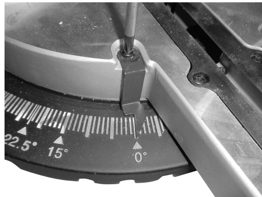
Figure G: Miter Table Angle Indicator Adjustment
