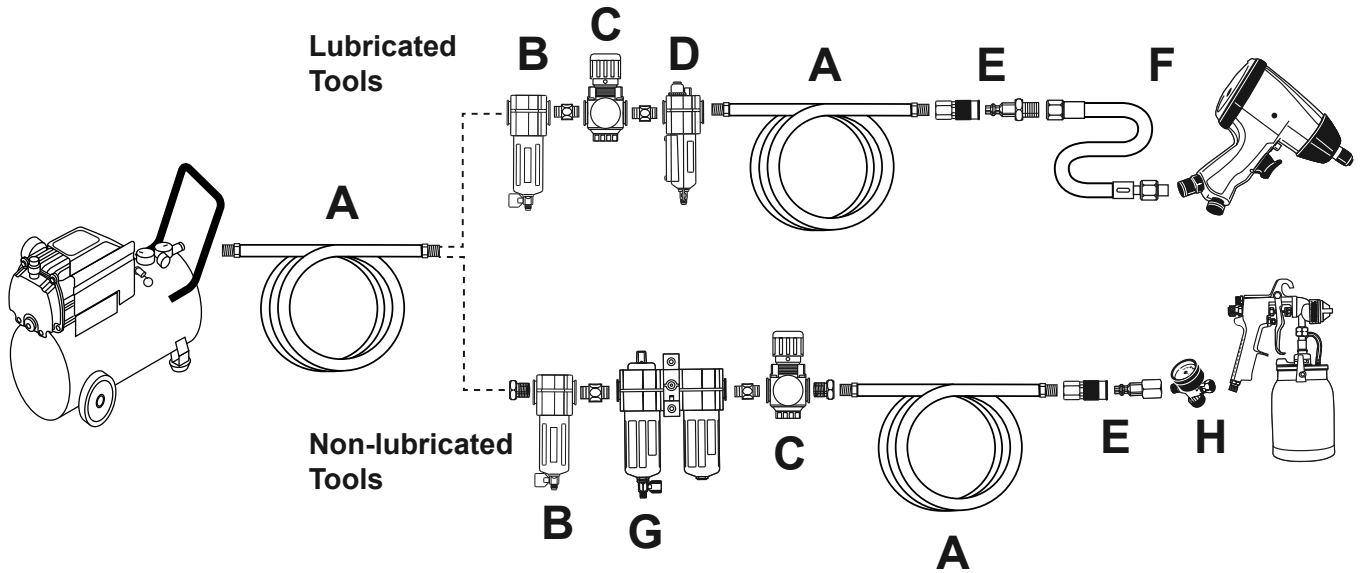
Figure C: Portable Air Supply Setup
