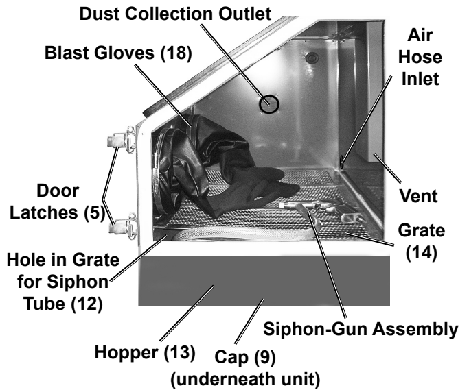
Figure A: Cabinet Setup
