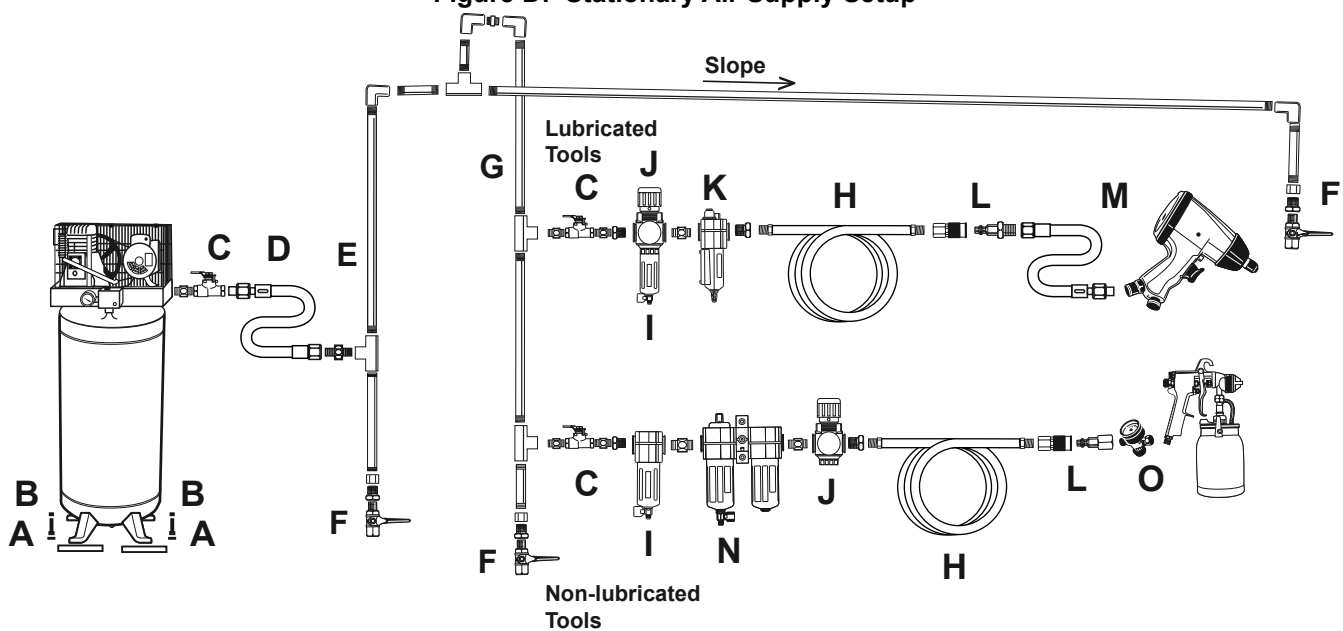
Figure D: Stationary Air Supply Setup
