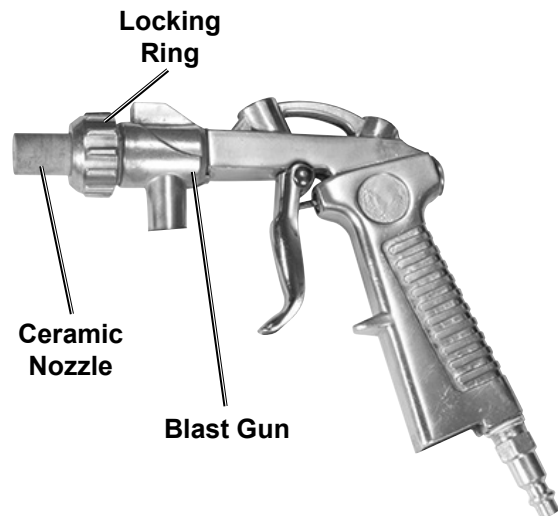
Figure B: Blast Gun Detail
