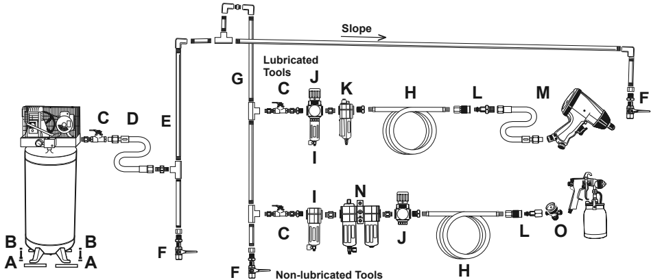
Figure B: Stationary Air Supply Setup
