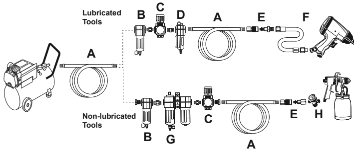
Figure A: Portable Air Supply Setup
