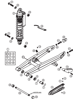
SCHWINGARM, FEDERBEIN SWINGARM, MONOSHOCK
