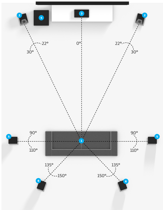
Speaker placement for 7.1.2 setup
