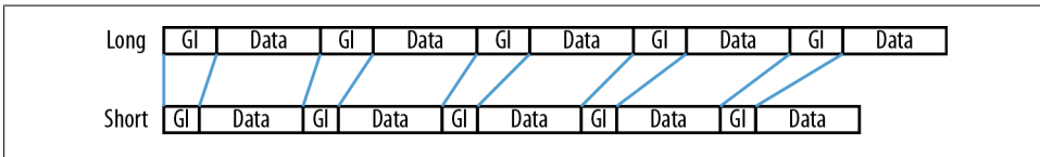
Figure 3-4. Long and short guard interval compared
