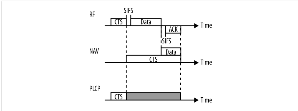
Figure 5-11. L-SIG duration
