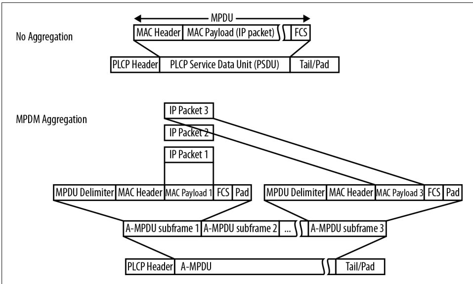
Figure 5-4. A-MPDU aggregation
