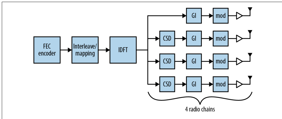
Figure 2-3. 4x4 802.11n interface block diagram
