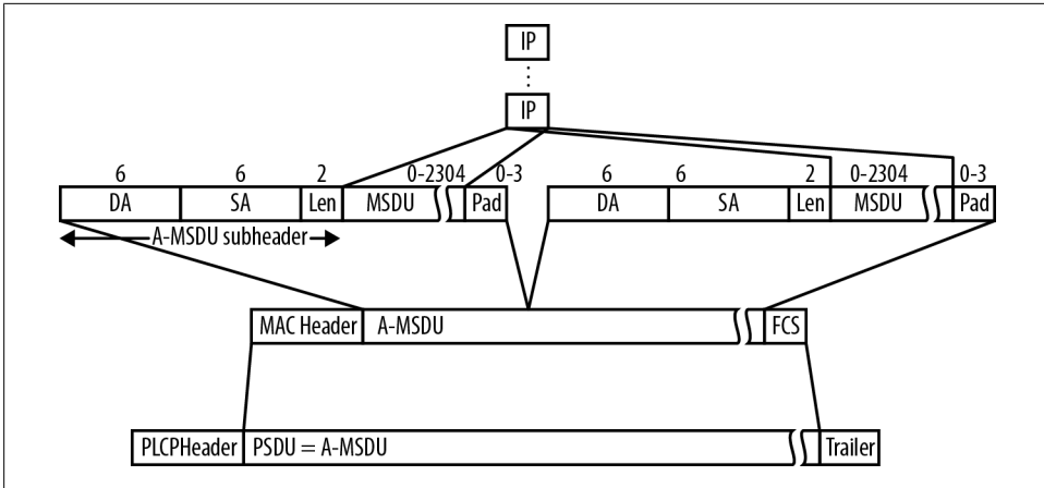
Figure 5-5. A-MSDU aggregation
