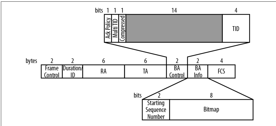
Figure 5-9. Compressed Block ACK frame
