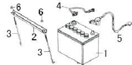
Battery Tray
