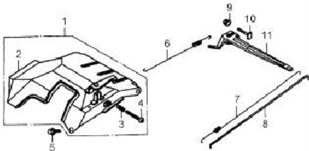
Speed Control
