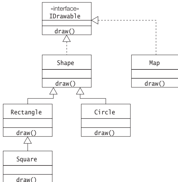
Figure 7.4 Type Hierarchy to Illustrate Polymorphism
