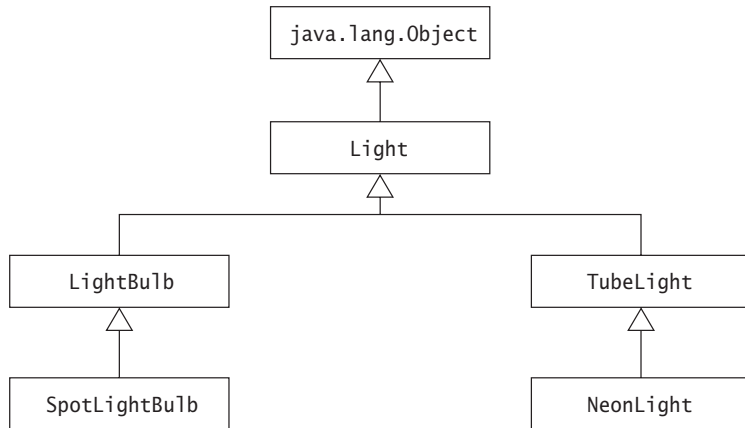
Figure 7.1 Inheritance Hierarchy
