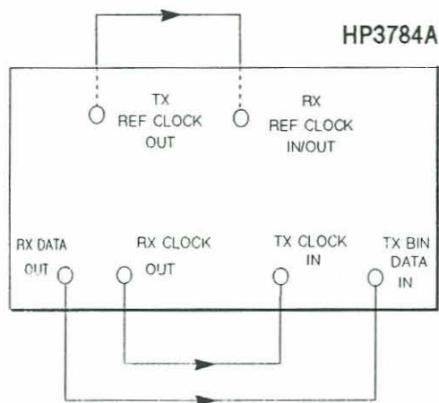
Figure 3-3 Jitter Measurements on a Binary Clock.
