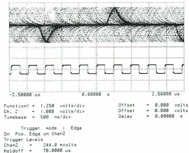
Figure 8-22 8UI p-p Jitter
