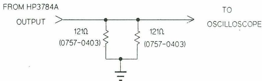
Figure 8-35 Termination Network
