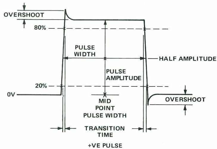
Figure 8-38 Pulse Characteristics
