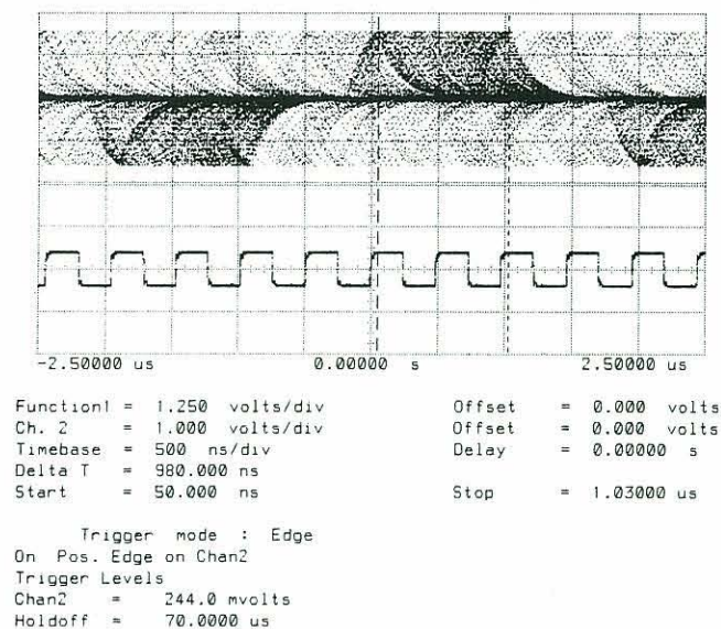
Figure 8-23 10UI p-p Jitter
