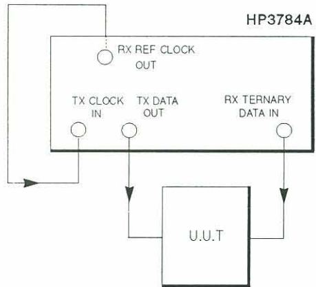
Figure 3-12 Equipment Setup.
