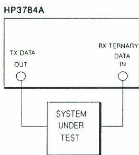
Figure 3-5 Equipment Setup
