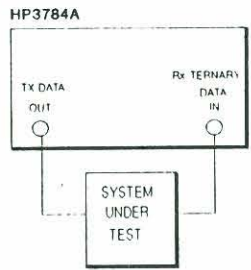
Figure 3-4 Equipment Setup
