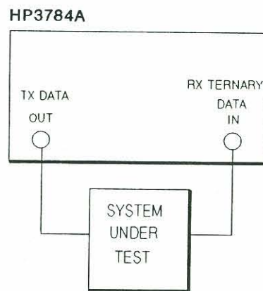
Figure 3-11 Equipment Setup
