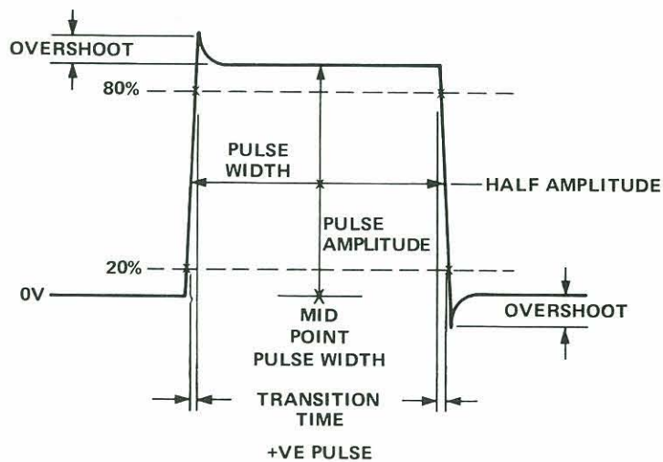
Figure 8-9 Pulse Characteristics
