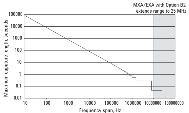
Figure 4a. MXA (RF mode) and EXA capture length vs. span.
