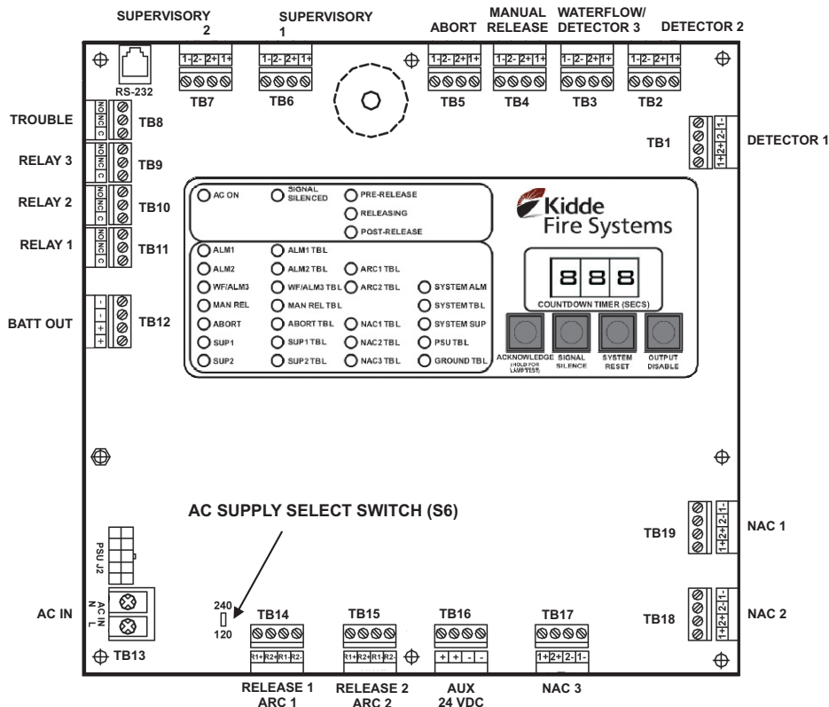
Figure 1. Printed Circuit Board (PCB)
