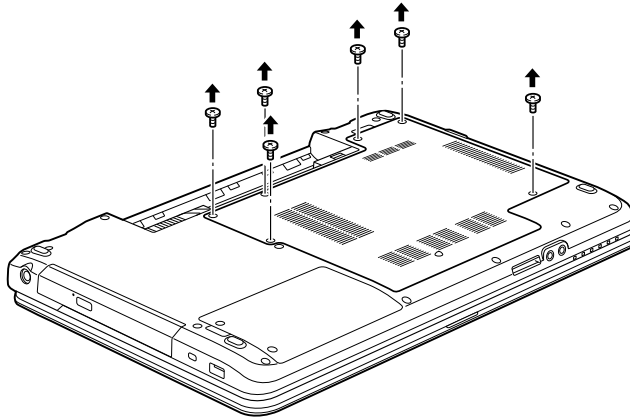
Figure 29. Removing the Memory Cover Screws
