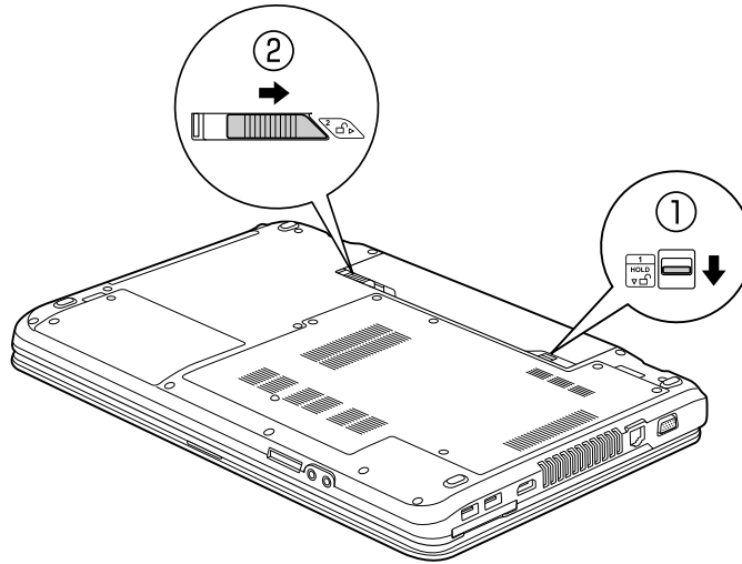
Figure 21. Battery lock and latch
