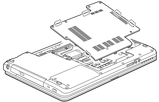
Figure 30. Removing the Memory Cover
