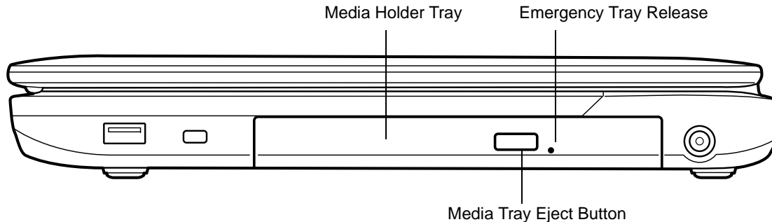
Figure 23. Optical Drive
