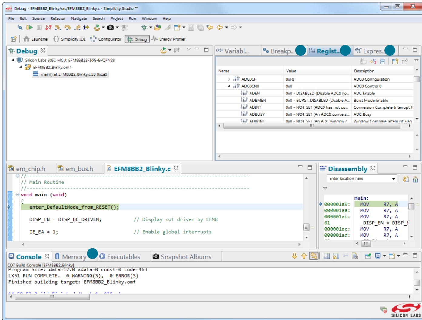
Figure 4.2. Navigating the IDE while Debugging
