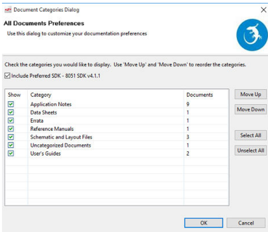
Figure 2.6. Documentation Preferences
