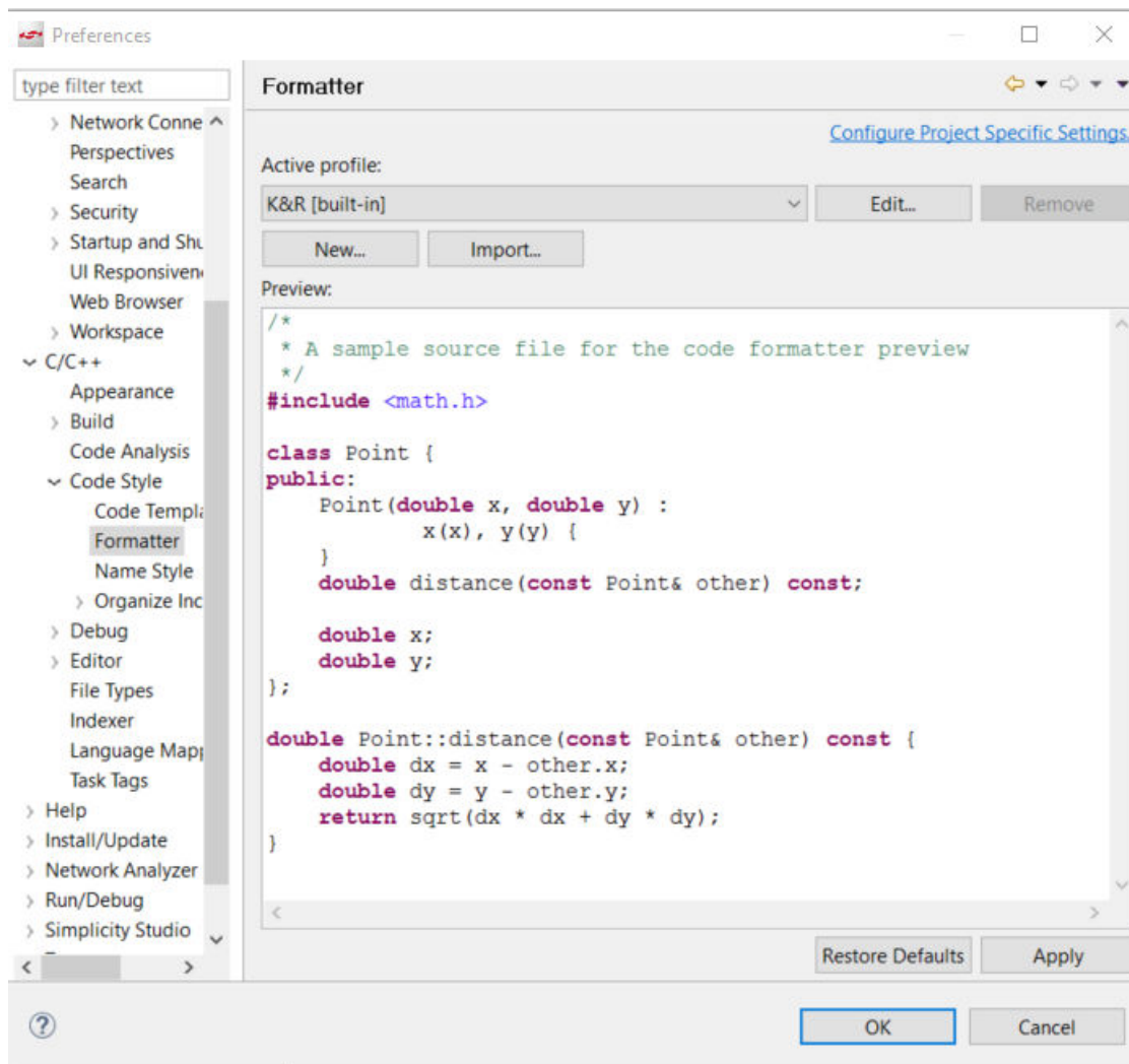
Figure 11.2. Code Style Formatter Preferences
