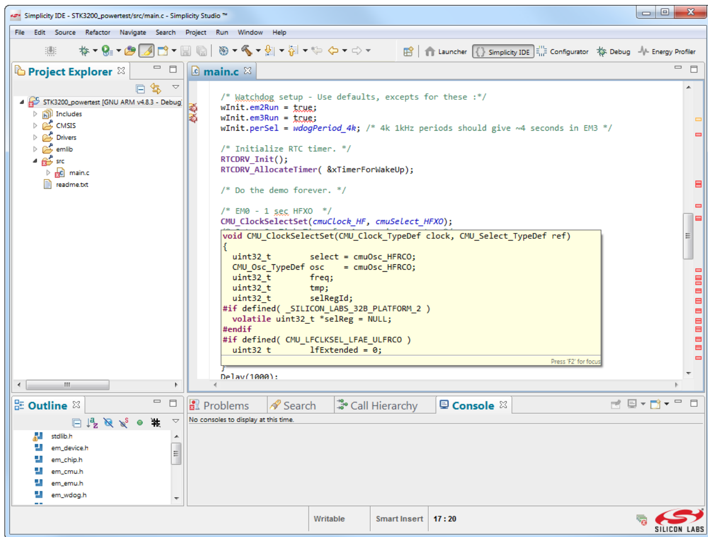
Figure 3.1. Simplicity IDE
