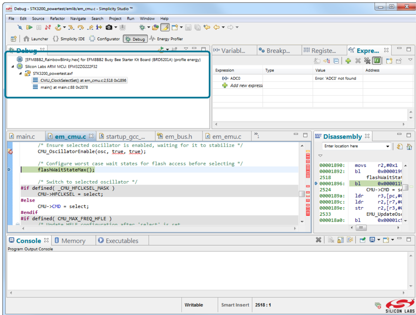
Figure 4.3. Debugger Call Hierarchy
