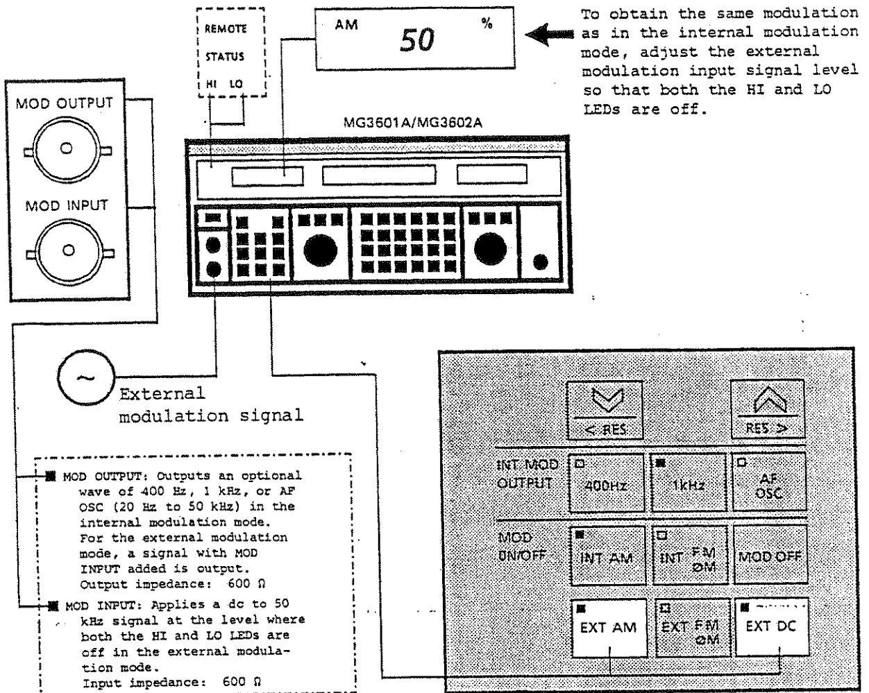
Fig. 5-22 External AM Modulation
