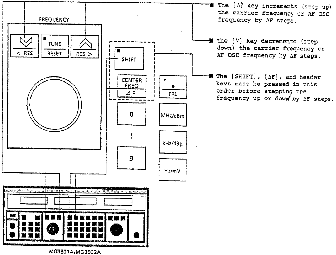
Fig. 5-16 Setting AF OSC Modulation Frequency Using Step Keys
