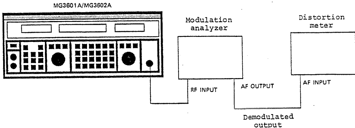
Fig. 4-7 AM Modulation Factor and AM Distortion
