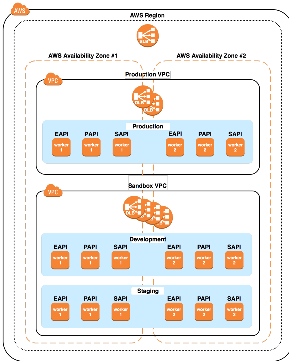
Figure 90. Two Anypoint VPCs were created in a CloudHub region: The Production VPC is associated with the Production environment and hosts two CloudHub Dedicated Load Balancers (DLB; presumably one for public APIs and the other for VPC-private APIs) while the Sandbox VPC is associated with the Development and Staging environments and hosts four CloudHub Dedicated Load Balancers (presumably separating public and VPC-private APIs for the two environments). Several API implementations from all tiers of API-led connectivity have been deployed to all environments using two CloudHub workers each. The CloudHub workers for a given Mule application are assigned to different AZs. The CloudHub Shared Load Balancer (SLB) for the region is available for public APIs (but may go unused given the configured CloudHub Dedicated Load Balancers).
