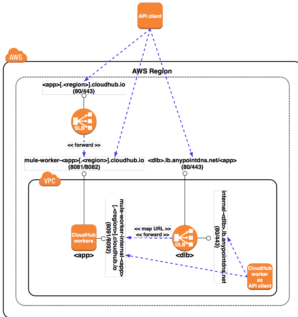
Figure 93. An API implementation/Mule application <app> is deployed to an Anypoint VPC, under management of the US Anypoint Platform control plane. This <app> exposes HTTP/HTTPS endpoints on ports 8081/8082 as well as on ports 8091/8092 (this combination in the same API implementation is unusual): depicted are the default access routes for API clients inside and outside this VPC, both directly to the CloudHub workers (unusual) as well as via the CloudHub Shared Load Balancer (SLB) and a CloudHub Dedicated Load Balancer <dlb>. The latter depends on <dlb>'s URL mapping rules, which are not shown.
