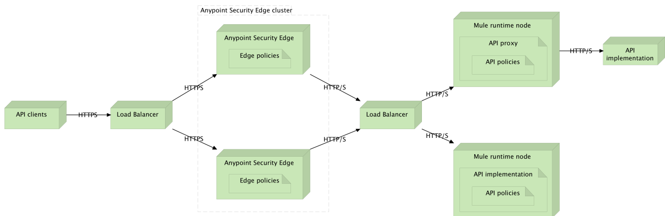
Figure 77. In a deployment of Anypoint Security Edge, API clients access an API via a cluster of Anypoint Security Edge nodes (acting as edge gateways) which enforce Edge policies for an entire group of APIs. This is independent of Anypoint API Manager-defined API policies enforced within Mule runtimes.
