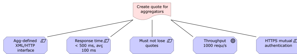
Figure 59. Essential NFRs for the "Create quote for aggregators" feature.
