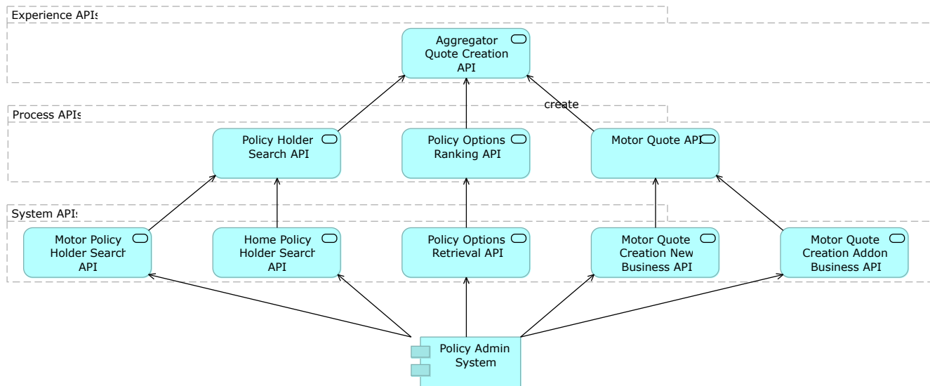
Figure 141. An example of the collaboration of APIs in the three tiers of API-led connectivity. Note the use of the simplified notion of API in this diagram, as lower-level APIs are shown serving higher-level APIs
