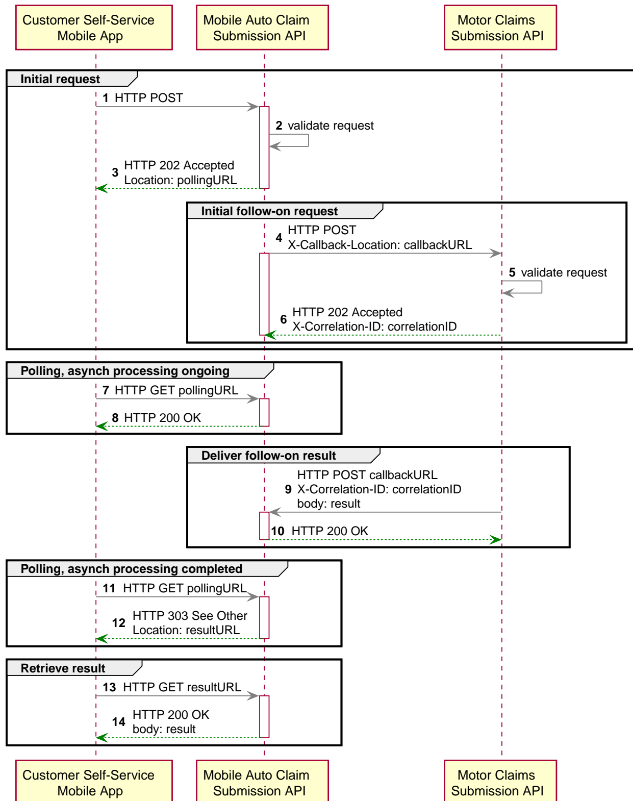
Figure 82. Asynchronous execution of the "Mobile Auto Claim Submission EAPI", with polling from the Customer Self-Service Mobile App, feeding into asynchronous execution of the "Motor Claims Submission PAPI", with callback to the "Mobile Auto Claim Submission EAPI".
