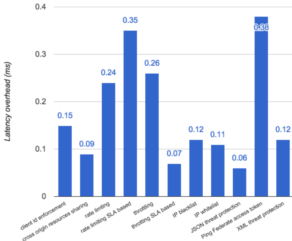
Figure 76. Increase in HTTP request-response latency through the application of various API policies, which are enforced embedded in the API implementation.
