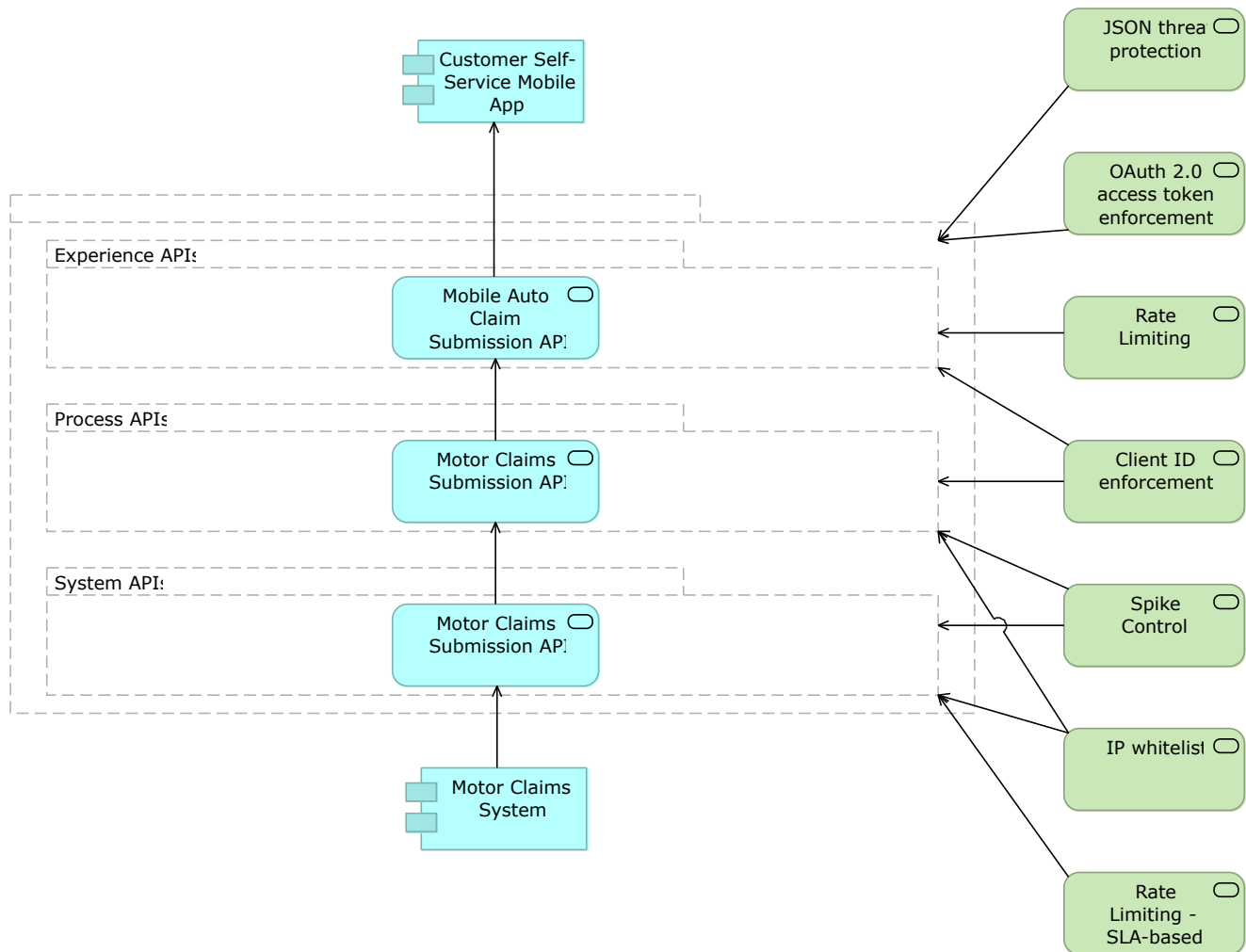
Figure 75. API policies applied to APIs in all tiers collaborating for the "Submit auto claim" feature (the suggested order of API policies is not visible in this diagram).
