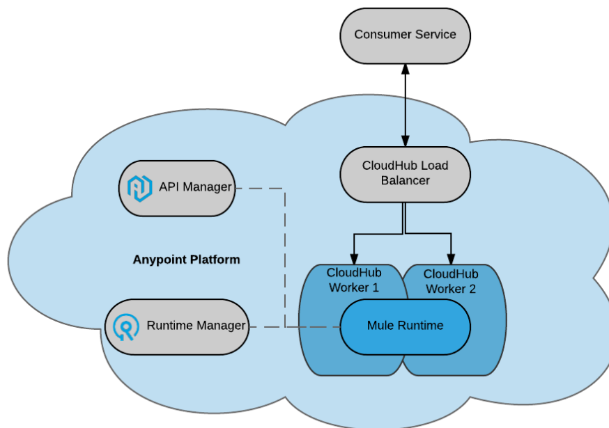
Figure 28. MuleSoft-hosted Anypoint Platform control plane managing MuleSoft-hosted Anypoint Platform runtime plane. Runtime plane comprises iPaaS-provisioned Mule runtimes on CloudHub in the public AWS cloud.
