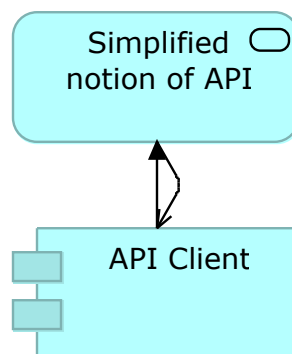
Figure 6. The simplified notion of API merges the aspects of application interface, technology interface, API implementation, application service and business service and is here represented visually as an application service element with the name of the API. An API in this simplified sense directly serves an API client and is invoked (triggered) by that API client.
