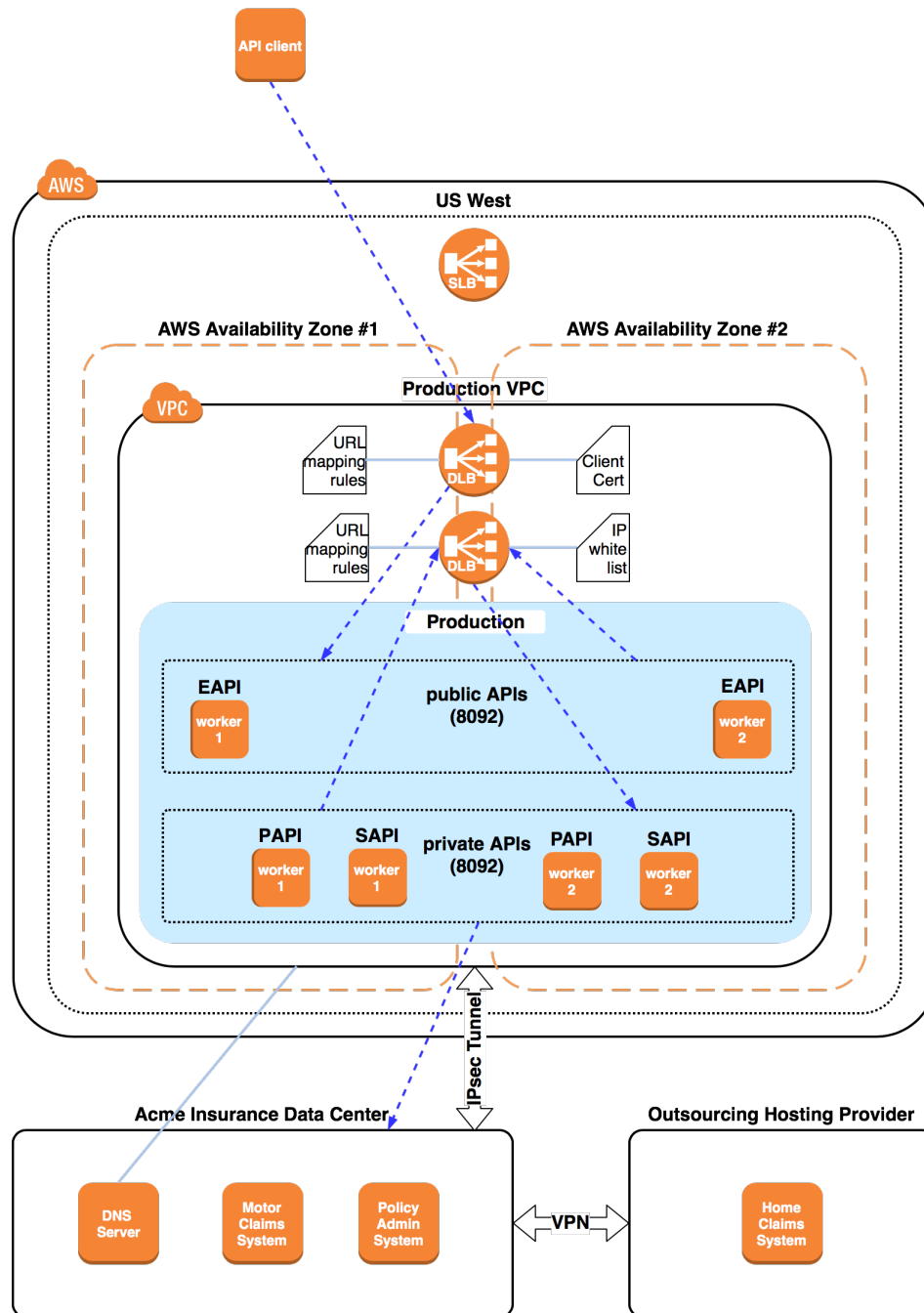
Figure 94. CloudHub Technology Architecture for Acme Insurance. Blue dashed arrows indicate typical request flows (over HTTPS unless from a System API to a backend system), which are subject to firewall restrictions in the Anypoint VPC and Acme Insurance data center (not shown) and IP whitelisting in the private CloudHub Dedicated Load Balancer (DLB). Also not shown are: individual concrete API implementations, CloudHub worker sizes, hostnames and URLs. The grouping around public APIs and private APIs is not reflected in any configuration and only serves to visualize the association of these API groups with the respective CloudHub Dedicated Load Balancers. The CloudHub Shared Load Balancer (SLB) for the region is shown but not used.
