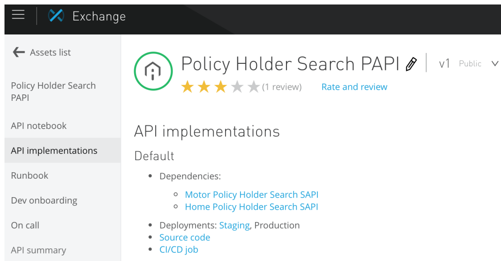
Figure 131. The Anypoint Exchange entry section dedicated to all known API implementations of a particular major version of an API.
