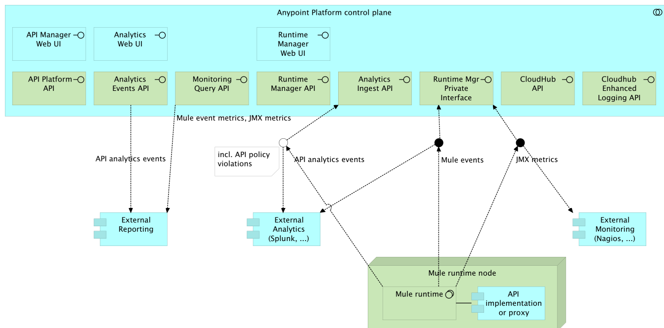
Figure 115. Different types of data used for monitoring, analytics and alerting flow from Mule runtimes to Anypoint Platform control plane components like Anypoint Runtime Manager, Anypoint API Manager and Anypoint Analytics and/or to external systems. Not all options are available in all Anypoint Platform deployment scenarios.
