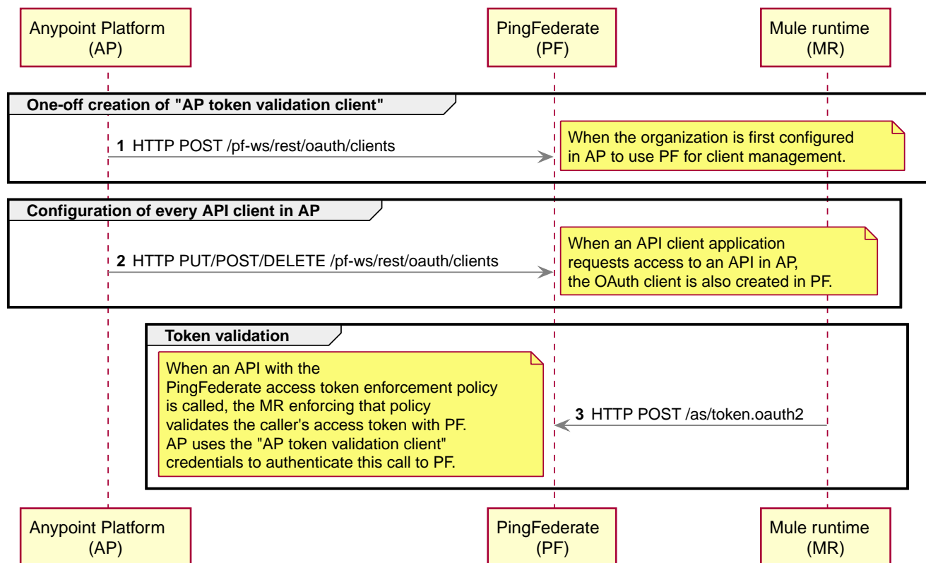
Figure 65. The interaction between Anypoint Platform, PingFederate as an Identity Provider configured for Client Management, and a Mule runtime enforcing the PingFederate access token enforcement API policy.
