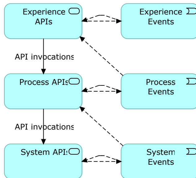
Figure 104. Flow of events and API invocations in API-led connectivity augmented with elements from Event-Driven Architecture (permitted API invocations between Process APIs are not shown).
