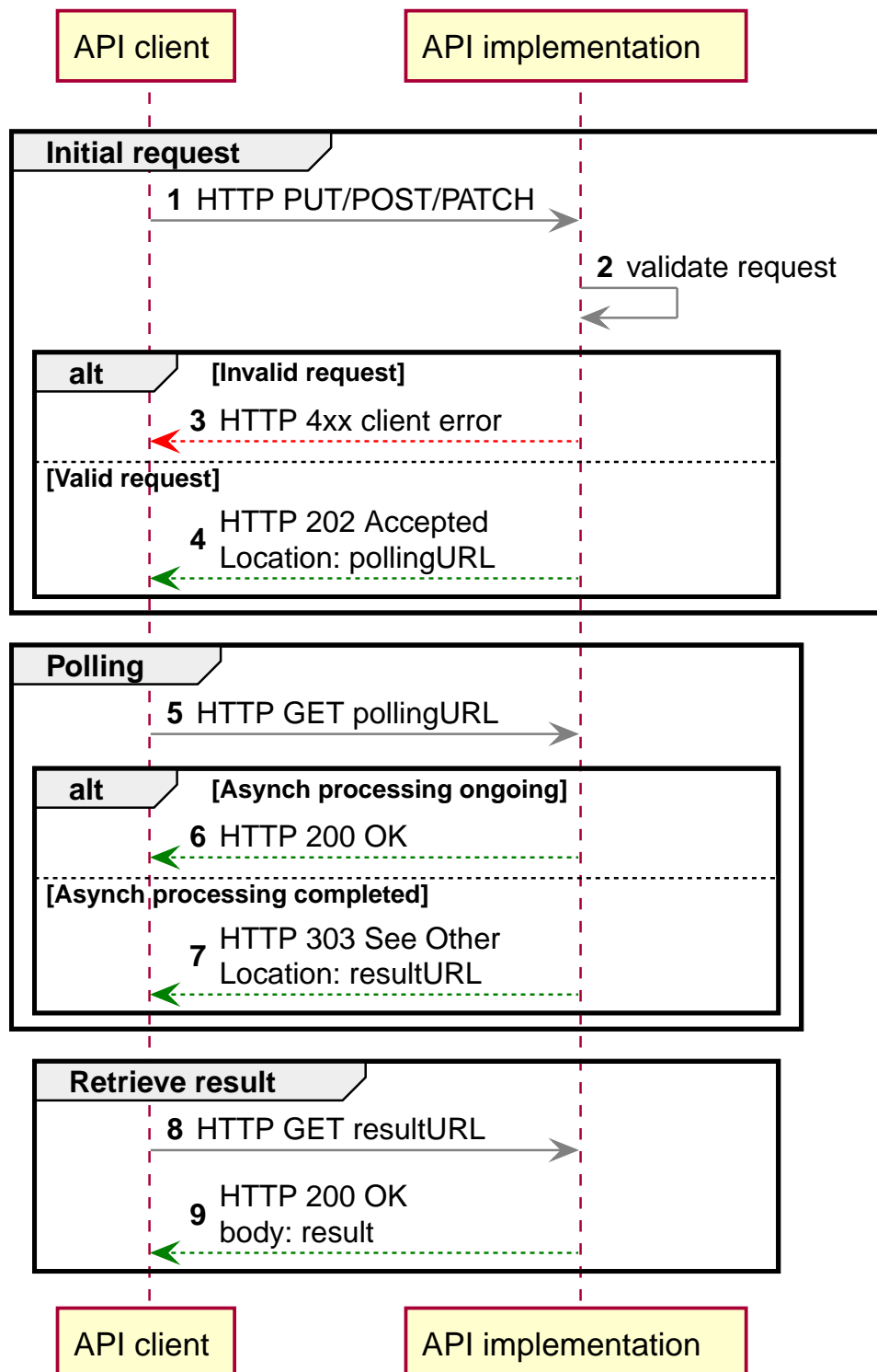
Figure 80. Asynchronous processing triggered by an API invocation from an API client to an API implementation, with polling by the API client to retrieve the final result from the API implementation.
