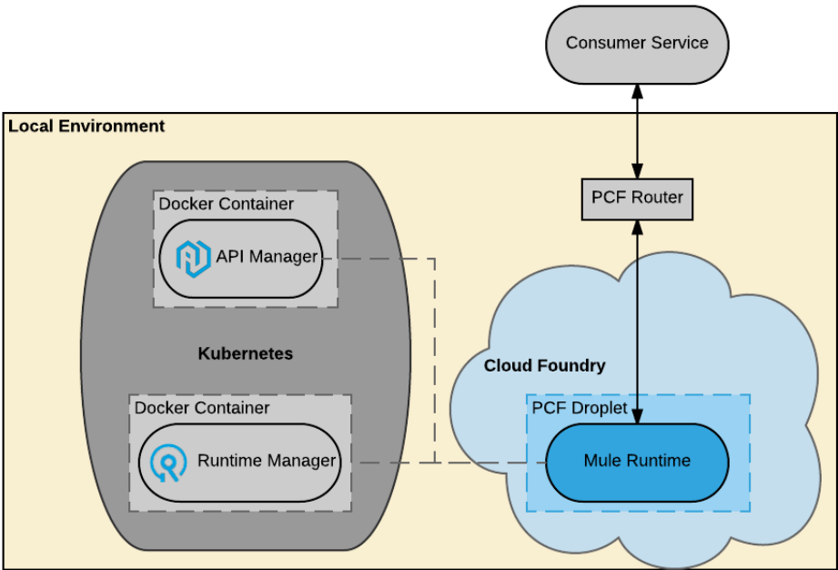
Figure 33. Anypoint Platform for Pivotal Cloud Foundry: Customer-hosted Anypoint Platform control plane managing customer-hosted Anypoint Platform runtime plane. Runtime plane comprises iPaaS-provisioned Mule runtimes on PCF.
