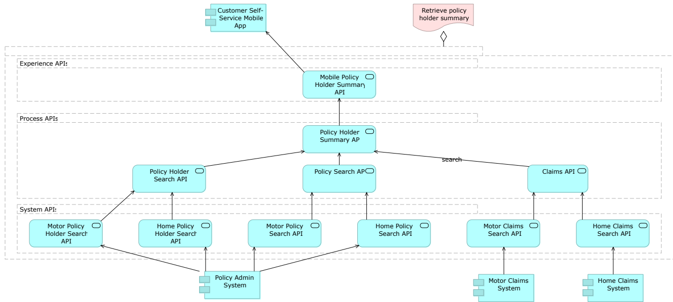
Figure 56. Experience API, Process APIs and System APIs collaborating for the "Retrieve policy holder summary" feature of the "Customer Self-Service App" product.
