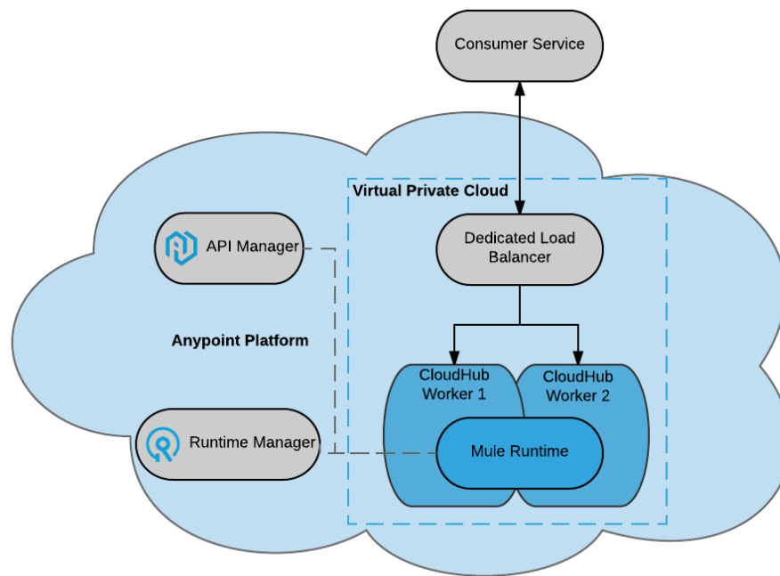
Figure 29. MuleSoft-hosted Anypoint Platform control plane managing MuleSoft-hosted Anypoint Platform runtime plane. Runtime plane comprises iPaaS-provisioned Mule runtimes on CloudHub in an Anypoint VPC.
