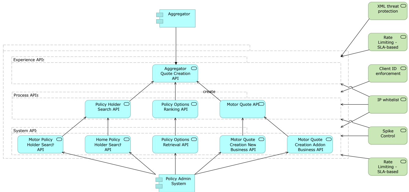
Figure 73. API policies applied to APIs in all tiers collaborating for the "Create quote for aggregators" feature (the suggested order of API policies is not visible in this diagram).
