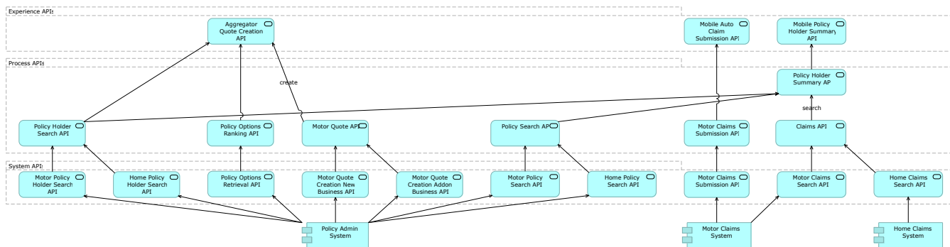
Figure 58. All APIs in the Acme Insurance application network after addressing the functional requirements of the "Aggregator Integration" product and "Customer Self-Service App" product.
