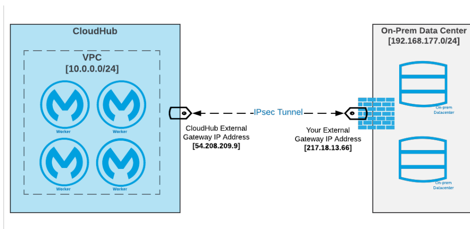
Figure 91. Private network connection via IPsec tunnel between an on-premises network (right side) and the AWS VPC underlying an Anypoint VPC (left side).
