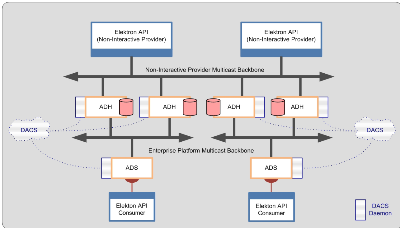
Figure 18. NIP: Multicast
