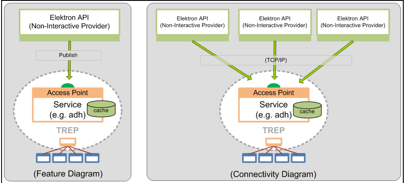
Figure 17. NIP: Point-To-Point
