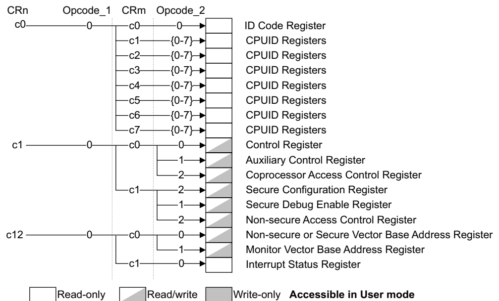
Figure 3-1 System control and configuration registers
