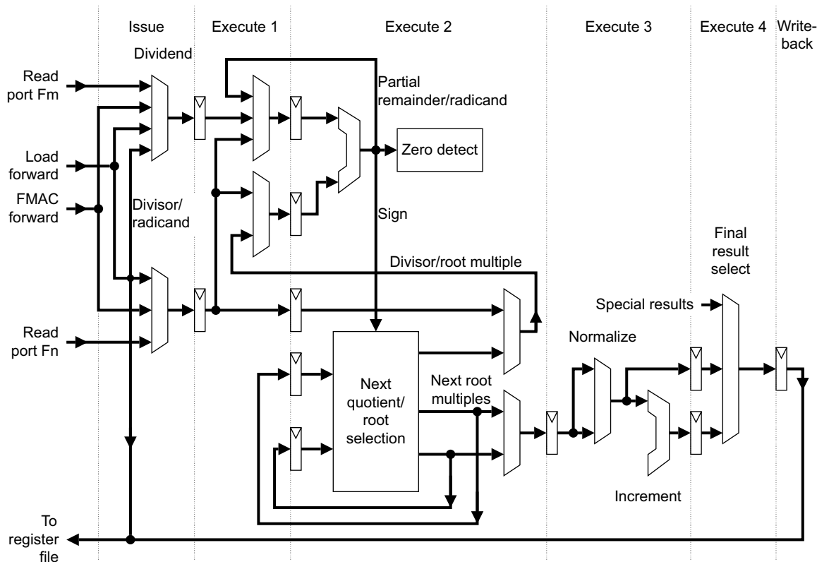
Figure 18-2 DS pipeline
