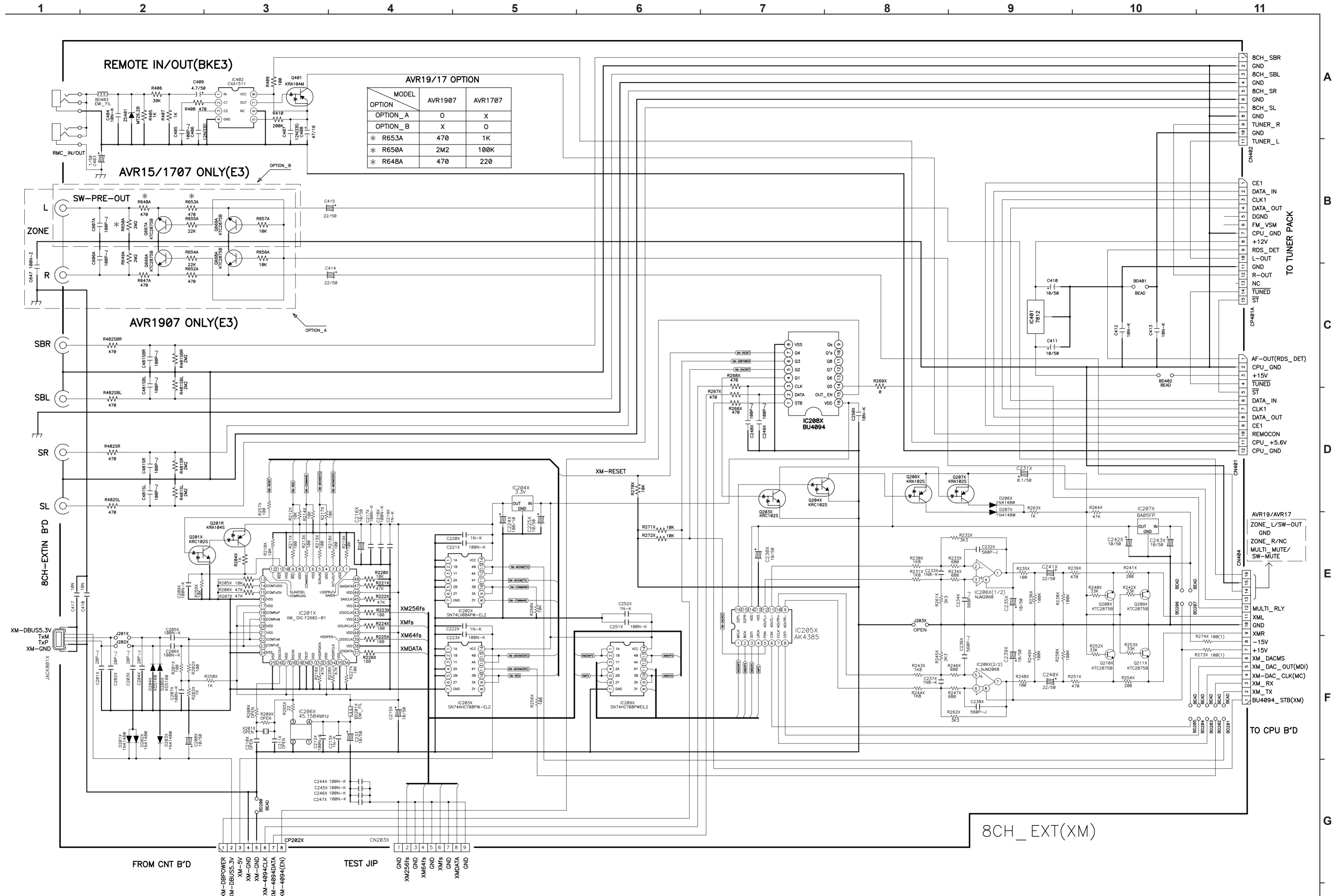
SCHEMATIC DIAGRAMS (15/17) 8CH-EXT(XM) UNIT (For AVR-1707/1507 E3 MODEL)
