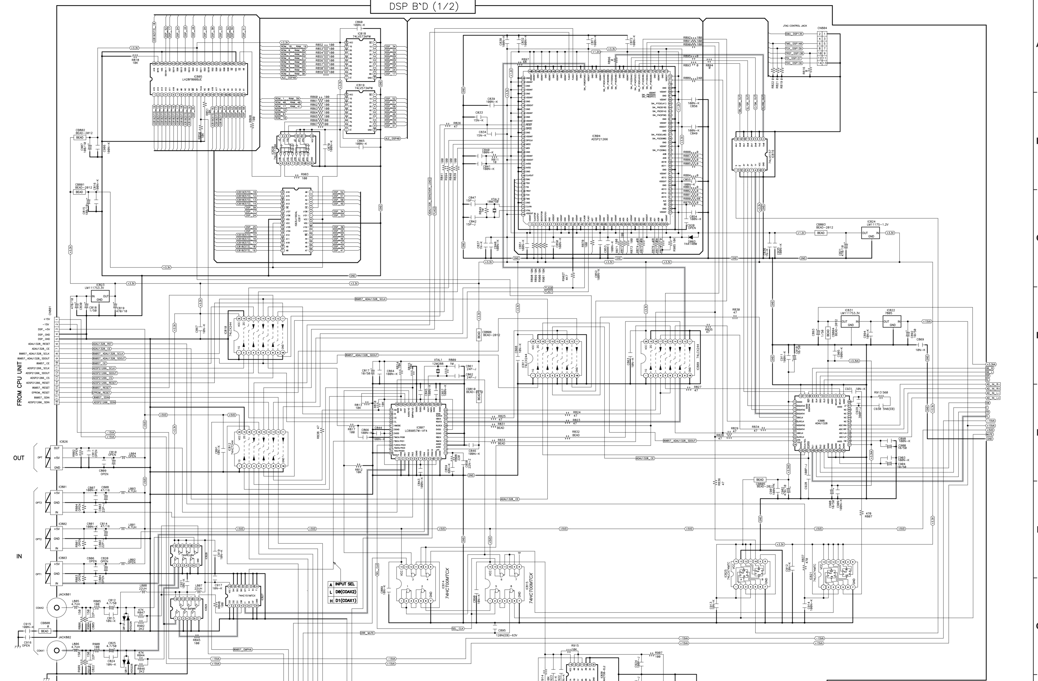
SCHEMATIC DIAGRAMS (13/17) DSP 2 UNIT (1/2) (For AVR-1507 MODEL)
