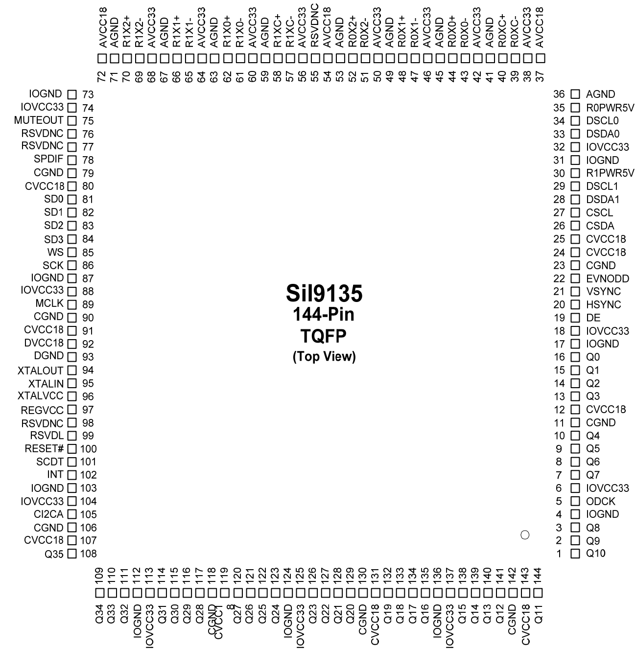
Figure 2. Pin Diagram
