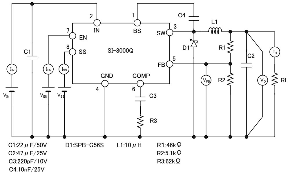
4-3測定回路図 Measurement circuit diagram
