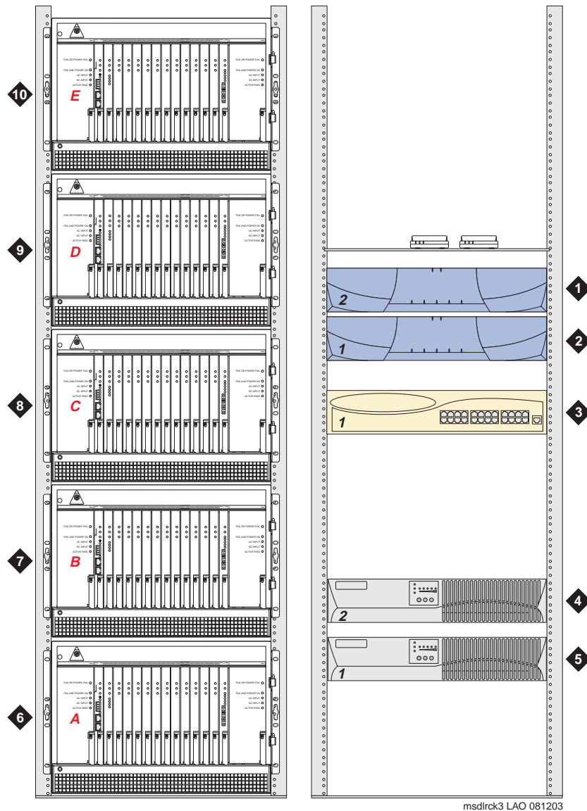
Figure 45: G650 stack
