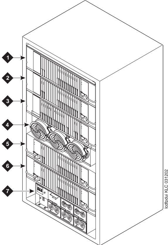
Figure 58: Typical MCC1 Media Gateway layout
