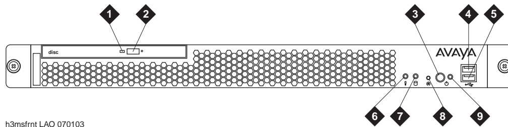
Figure 11: S8500 Media Server (front)
