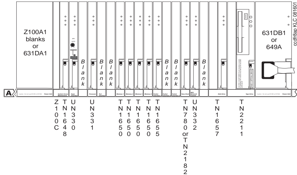
Figure 62: Processor Carrier
