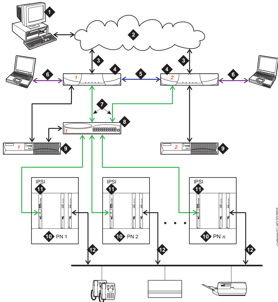
Figure 27: Duplex-reliability configuration when sending voice bearer over CSS or ATM
