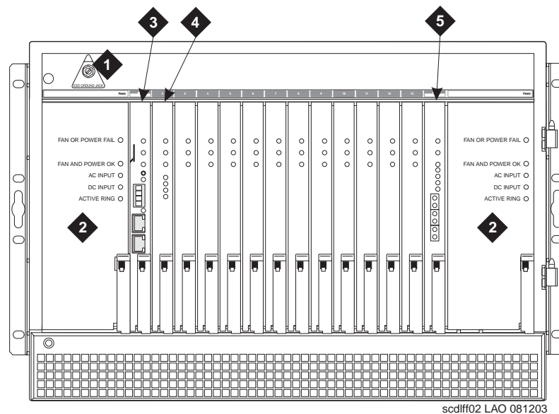
Figure 43: G650 Media Gateway
