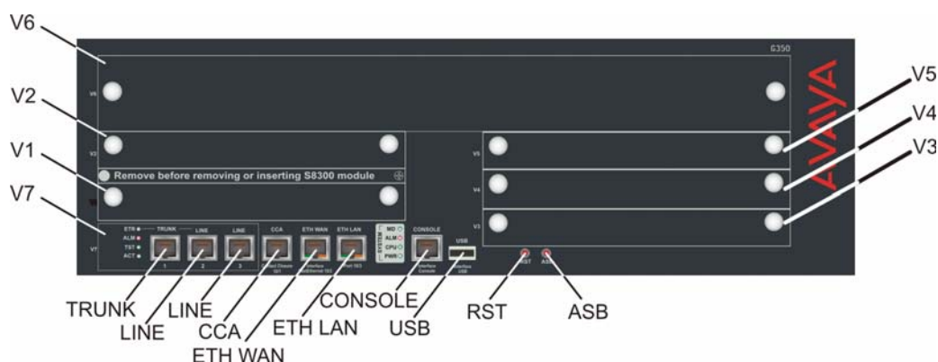
Figure 41: G350 chassis
