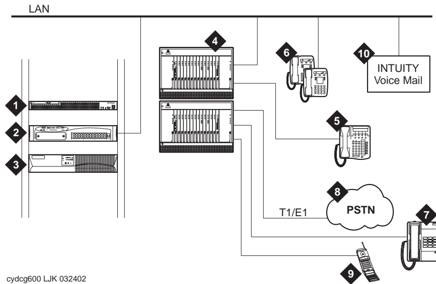
Figure 85: Medium-sized business solution using the Avaya S8500 Media Server and the G650 Media Gateway
