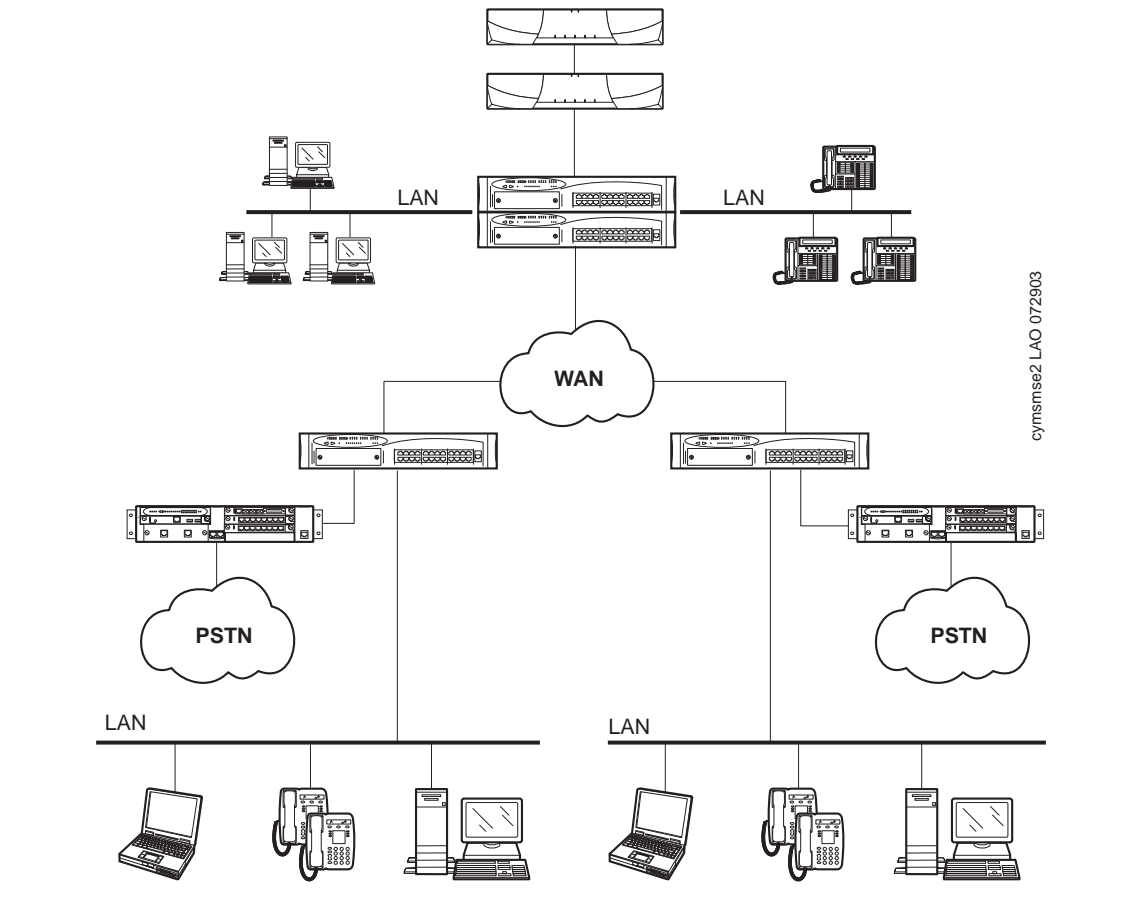
Figure 88: Multi-Site Configuration
