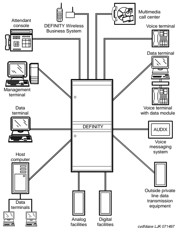
Figure 29: DEFINITY Server SI with Communication Manager
