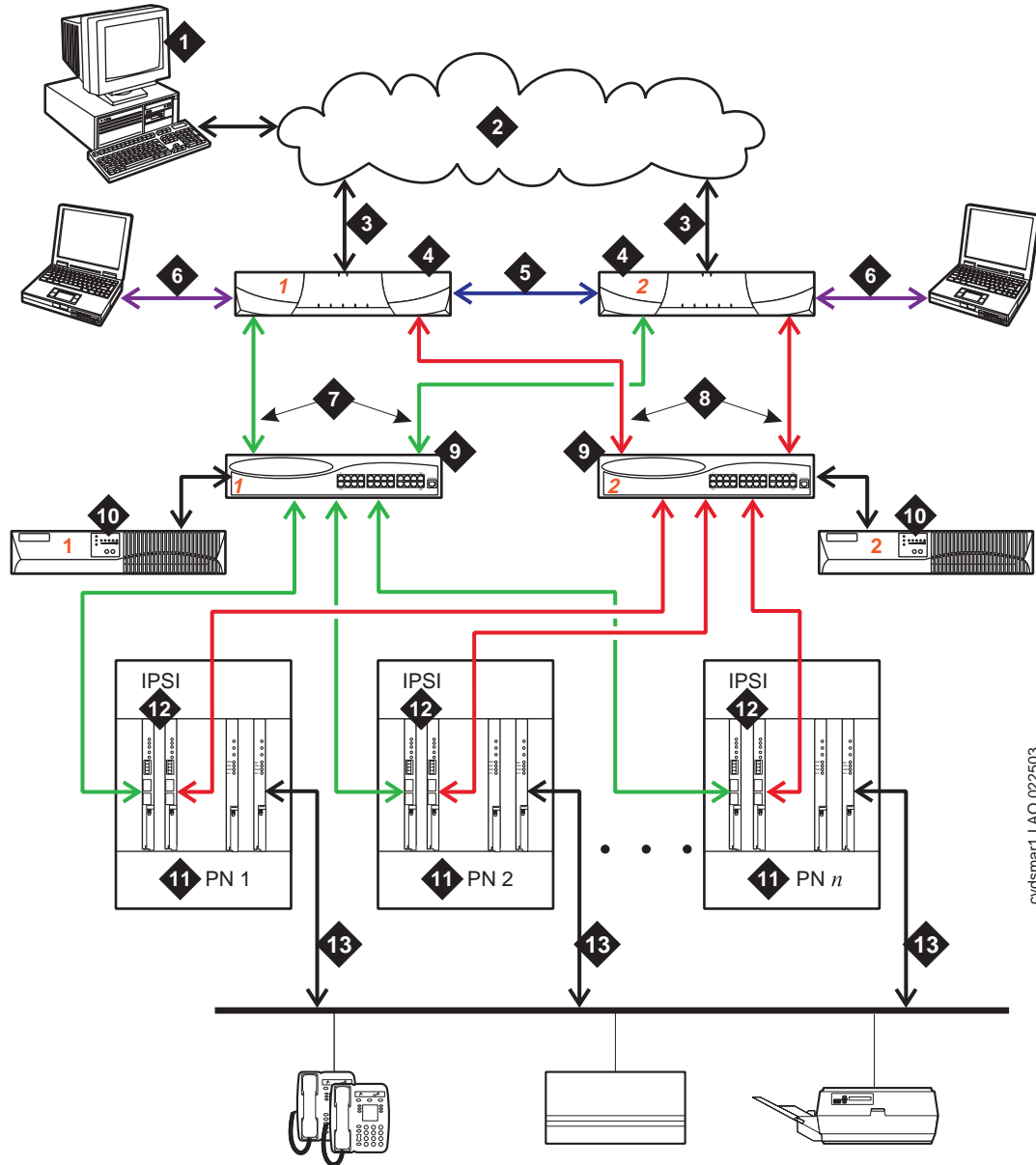
Figure 28: High-reliability configuration when sending voice bearer over CSS or ATM
