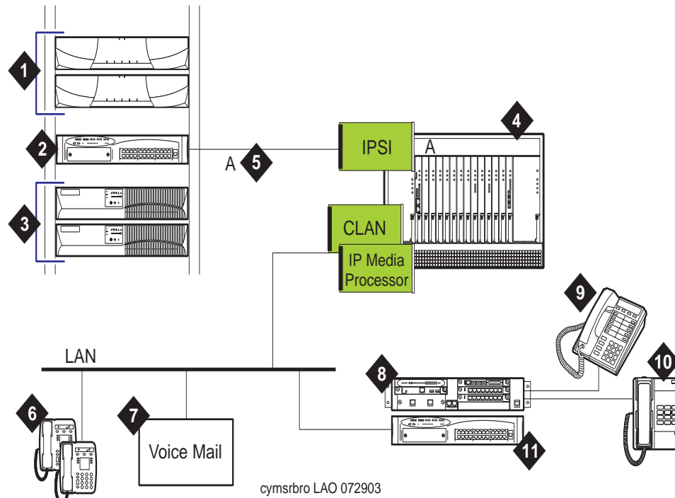
Figure 87: Branch Office Configuration
