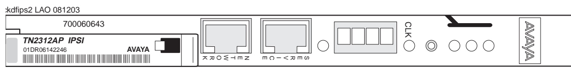
Figure 18: IPSI faceplate
