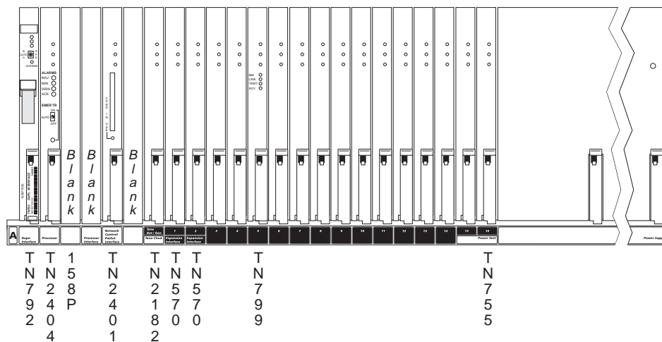
Figure 54: SCC1 basic control cabinet (front)
