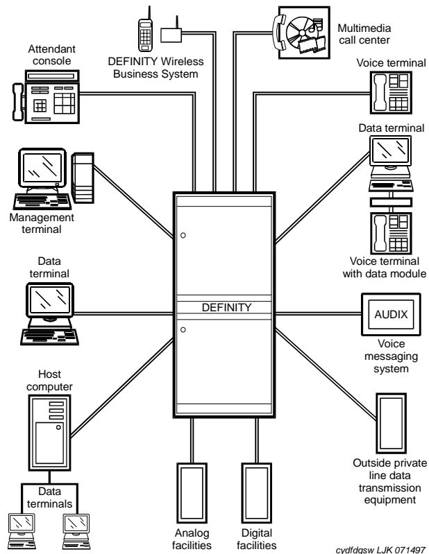
Figure 34: DEFINITY Server R
