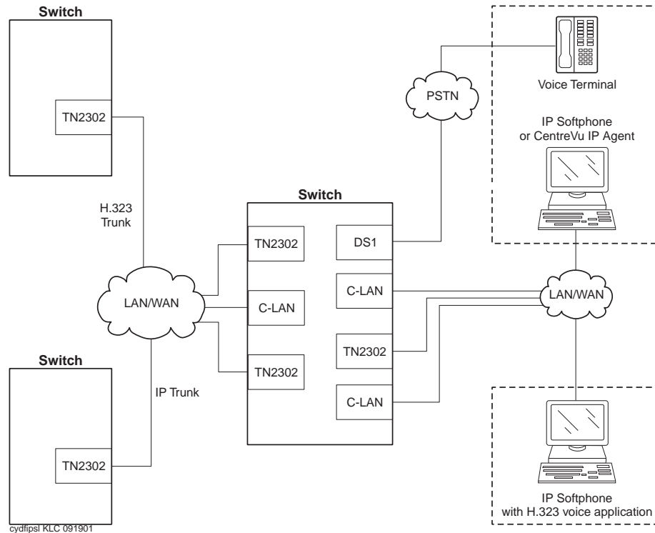
Figure 33: IP Solutions
