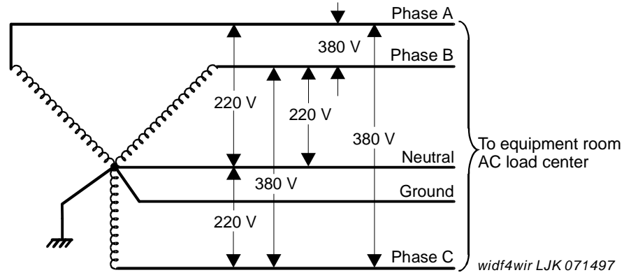
Figure 72: International, 3-phase, 220- to 380-VAC, 50-Hz source
