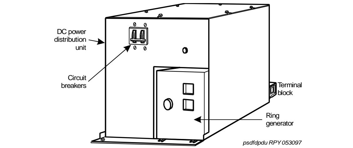
Figure 80: DC power-distribution unit (J58890CF-2) (front view)
