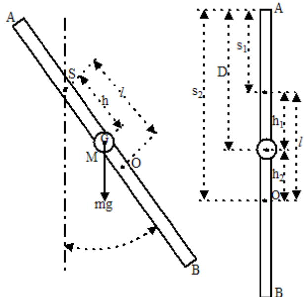
Fig. 1. Compound pendulum
