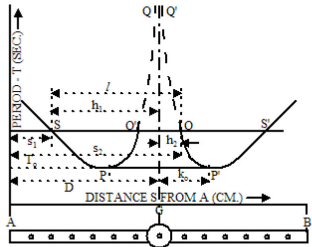
Fig. 2. Graphical analysis of the compound pendulum
