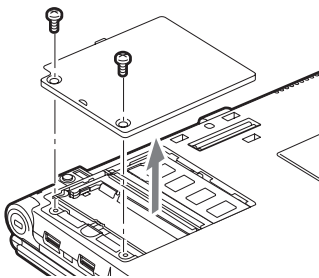
Figure 4-10. Removing the Memory Module Cover
