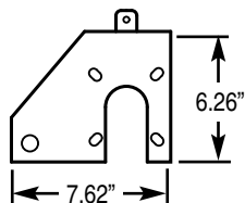
NEW STYLE SHIELD BRACKET
