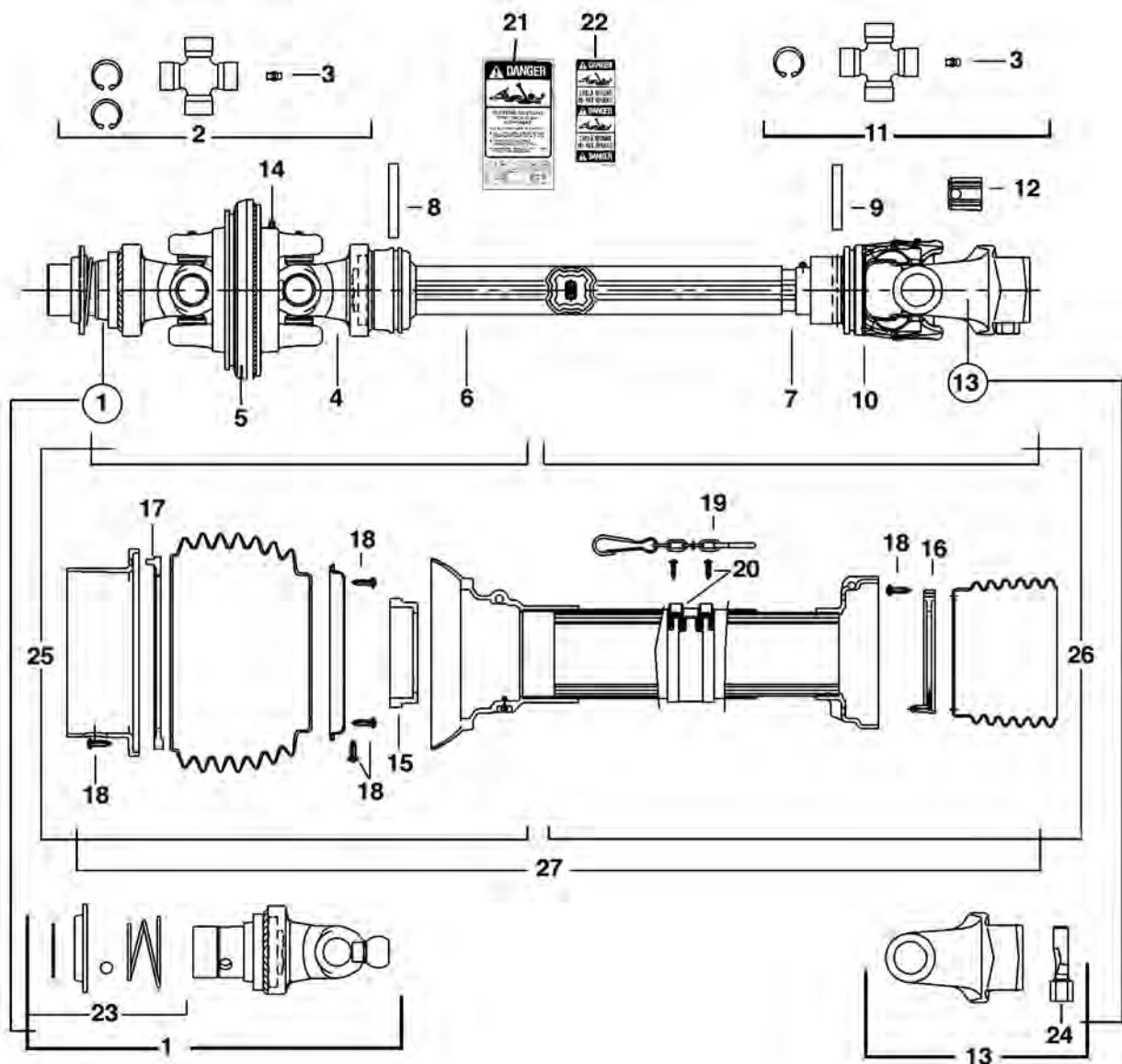
76842 CV DRIVESHAFT ASSEMBLY 1000 RPM, 1-3/8"- 21 SPLINE TRACTOR YOKE ASAE SIZE 4 MANUFACTURED BY BONDIOLI & PAVESI Used On: 1000 RPM Pull Models 3209, 3210, 3214 Replaced by 50053301SP (May Substitute 76624SP)
