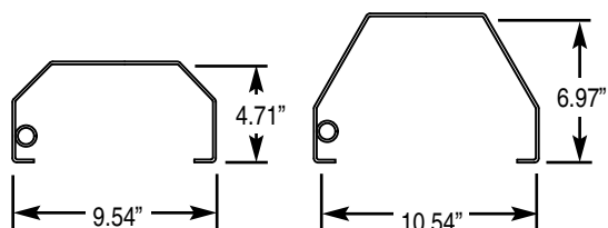
OLD STYLE CROSS SHIELD
