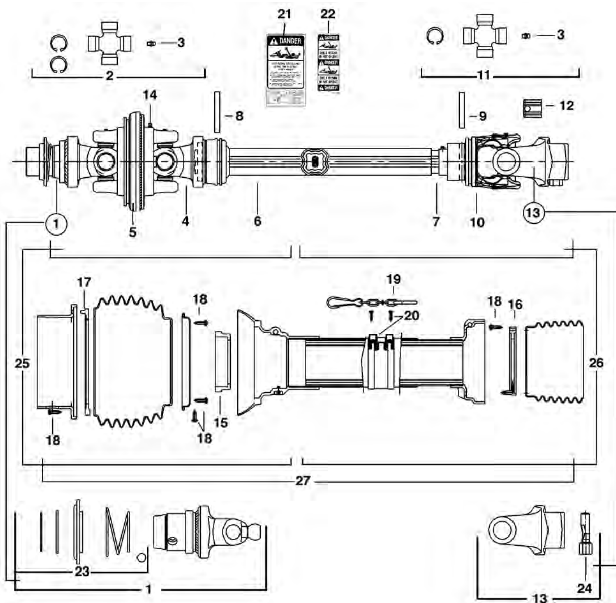
76843 CV DRIVESHAFT ASSEMBLY 1000 RPM, 1-3/4" - 20 SPLINE TRACTOR YOKE ASAE SIZE 4 MANUFACTURED BY BONDIOLI & PAVESI Used On: 1000 RPM Pull Models 3209, 3210, 3214 Replaced by 50053300
