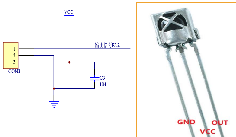
Figure .3.2.5.1 Circuit Diagram and Physical Map of Infrared Receiving Head
