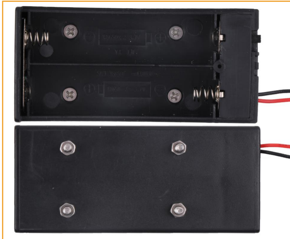
Figure 3.1.5.4 Effect diagram of Battery box fixed
