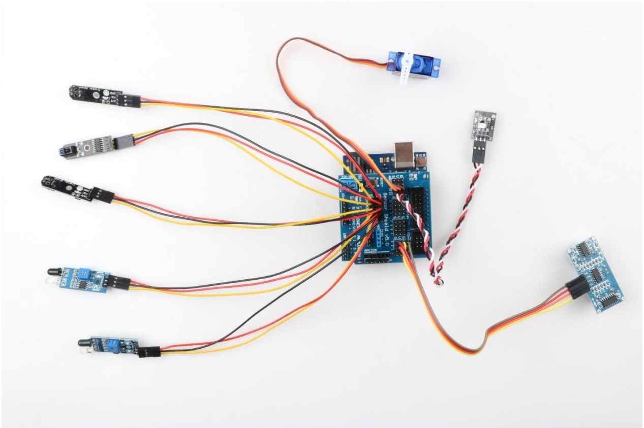
Figure 3.1.11.2 Extension board wiring diagram
