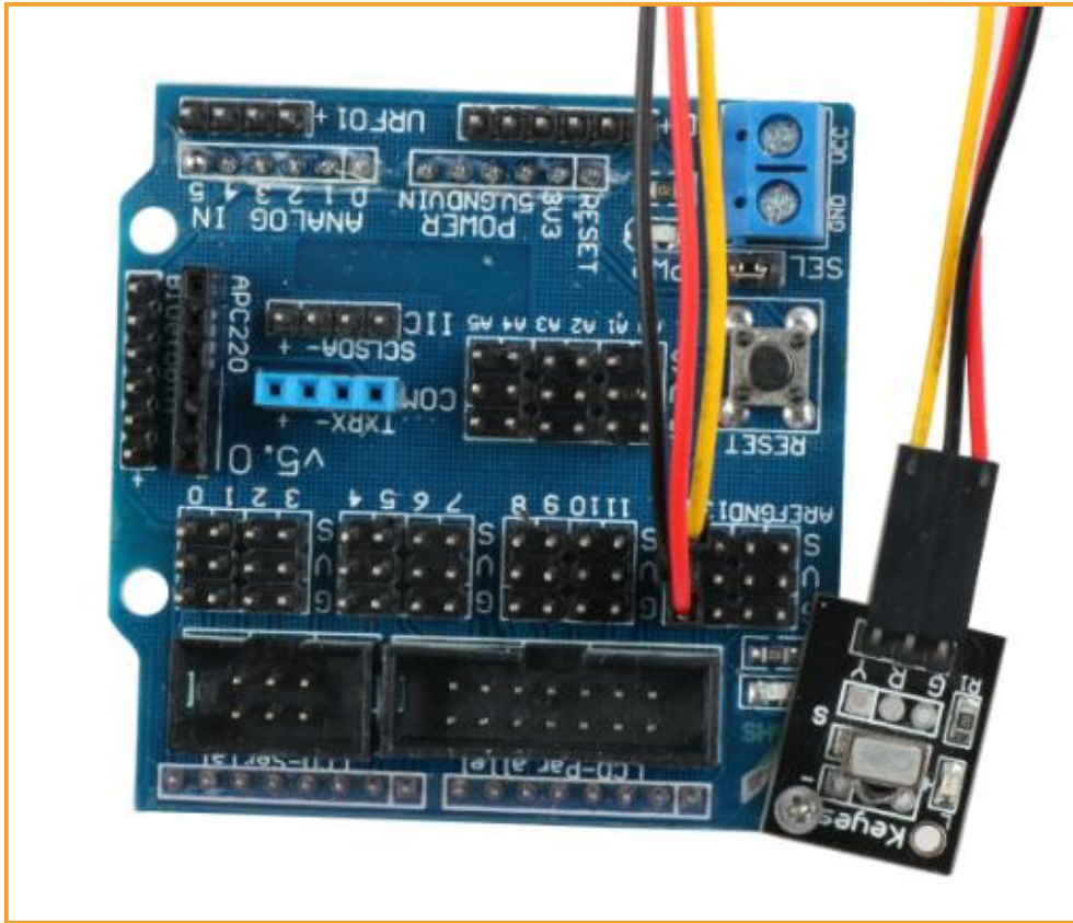
Figure 3.1.9.2 Effect diagram of infrared remote control receiver installation
