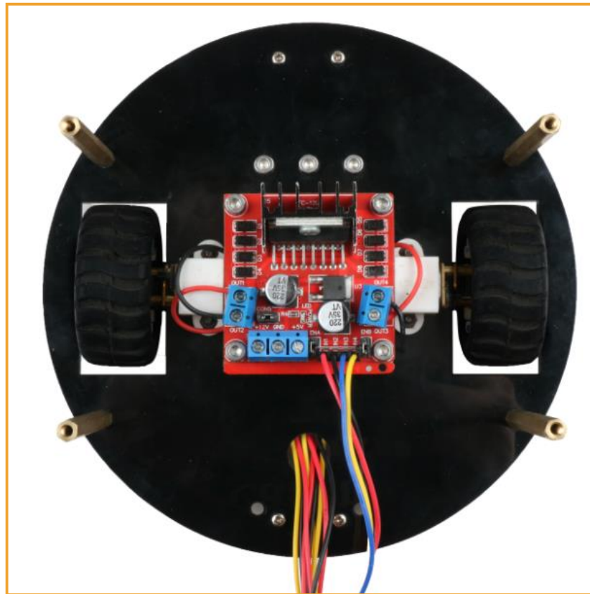
Figure 3.1.10.1 Effect Diagram of Wires Arrangement
