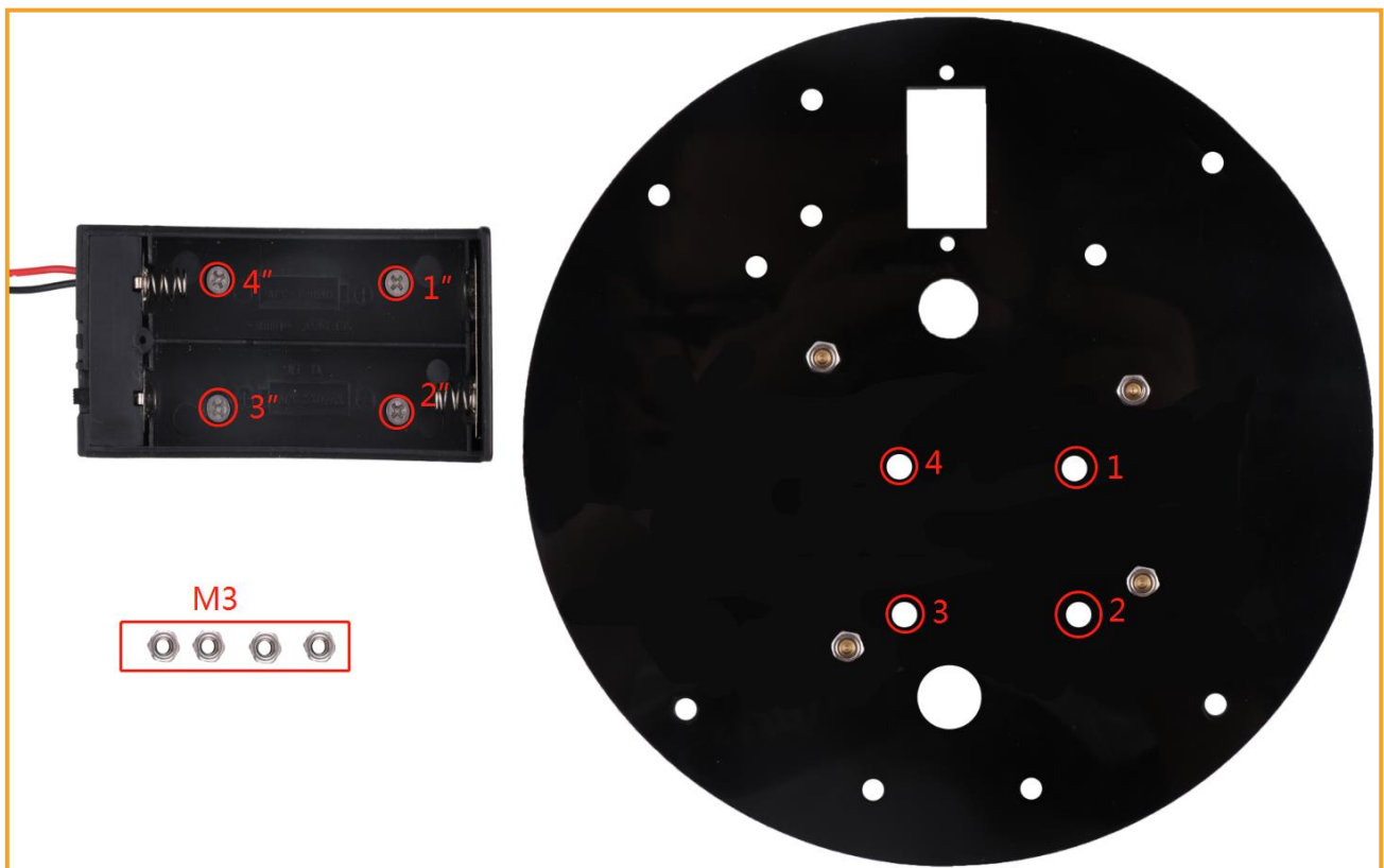
Figure 3.1.5.5 Schematic diagram of Battery box installation
