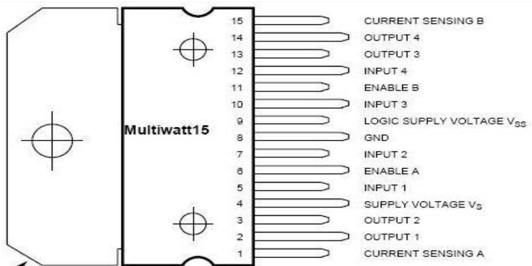
Figure .3.2.1.1 Arrangement of Chip Pins
