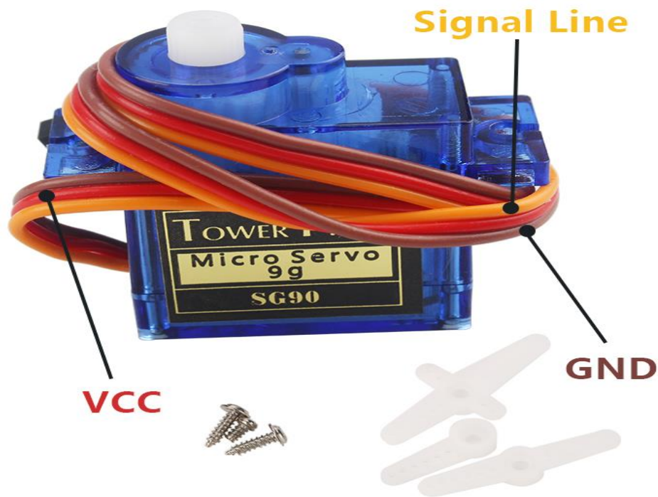
Figure .3.2.4.2 Physical Map of Steering Gear
