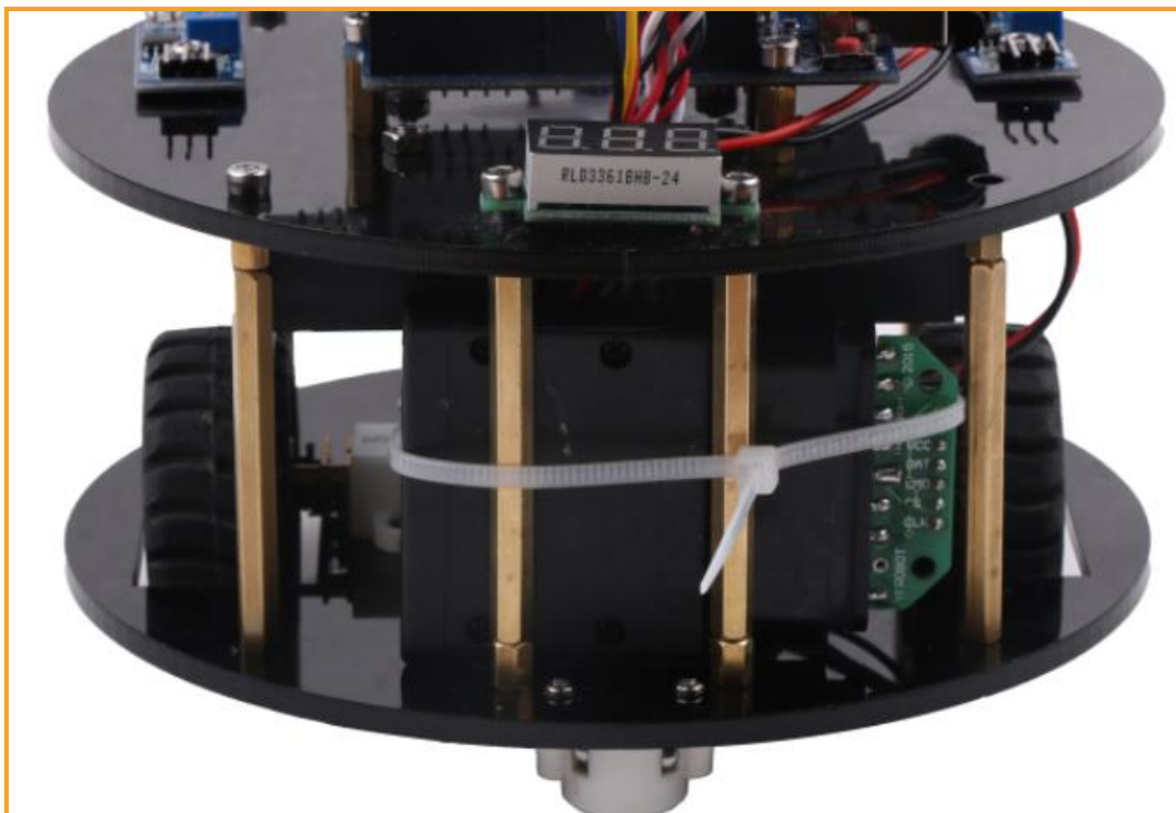
Figure 3.2.7.4 PS2 Receiver Fixed Overall Effect Diagram
