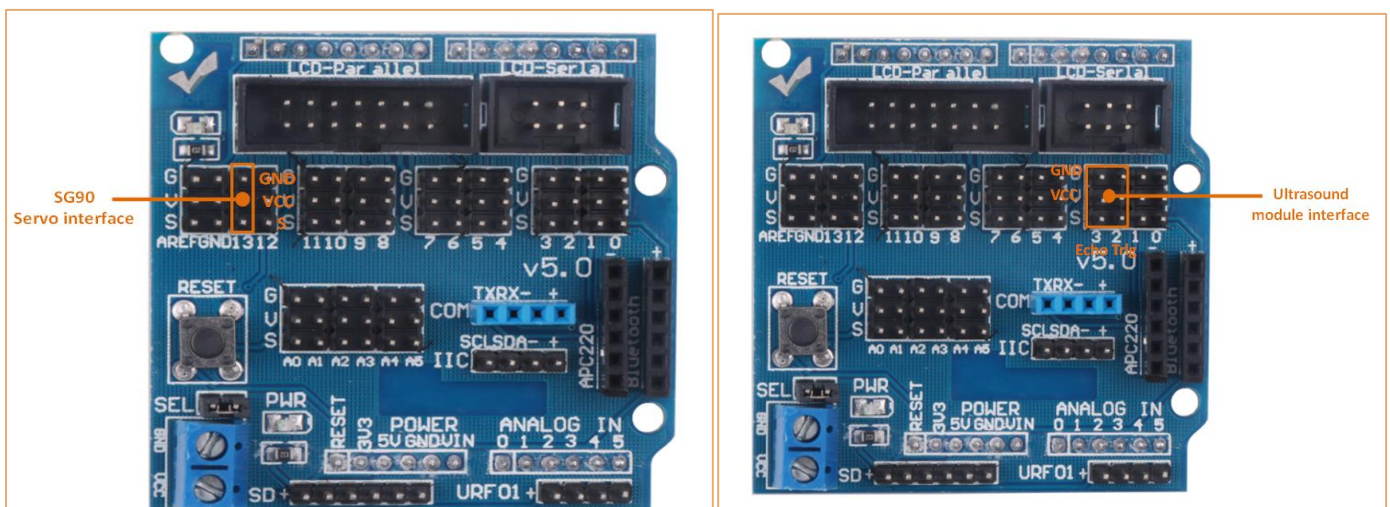
Figure 3.2.4.9 Wiring diagram of steering gear, ultrasonic wave and expansion board
