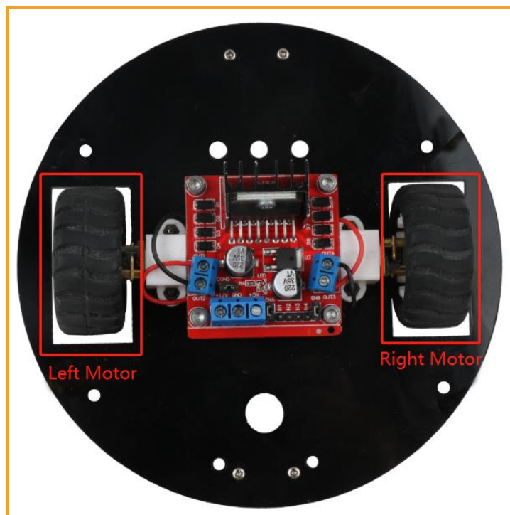
Figure 3.1.3.4 Effect diagram of Motor Driver Board Installation
