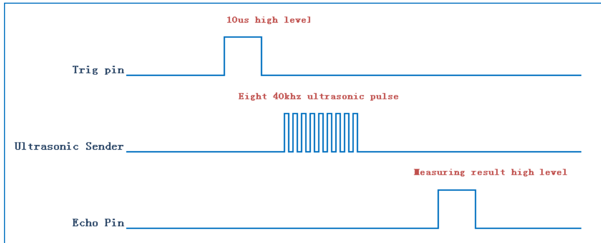
Figure .3.2.4.5 the Ultrasonic Working Sequence
