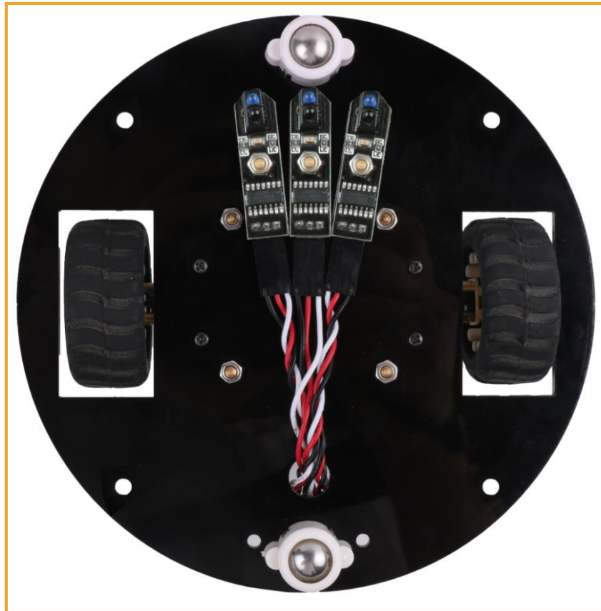
Figure 3.1.4.3 Effect diagram of the tracing module installation
