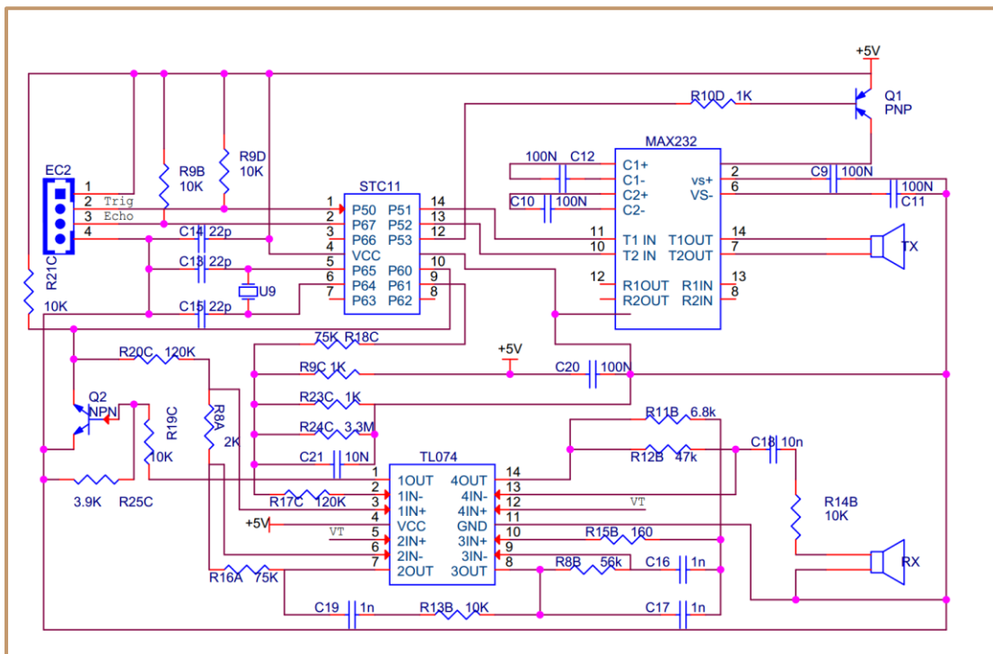
Figure .3.2.4.7 Schematic Diagram of Ultrasonic Transmitting and Receiving
