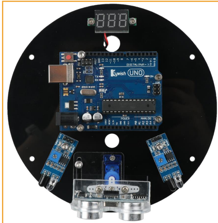
Figure 3.1.8.2 Effect diagram of voltage display module installation
