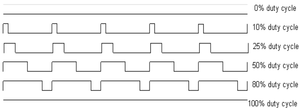
Figure .3.2.1.5 Sequence Diagram of PWM Duty Cycles
