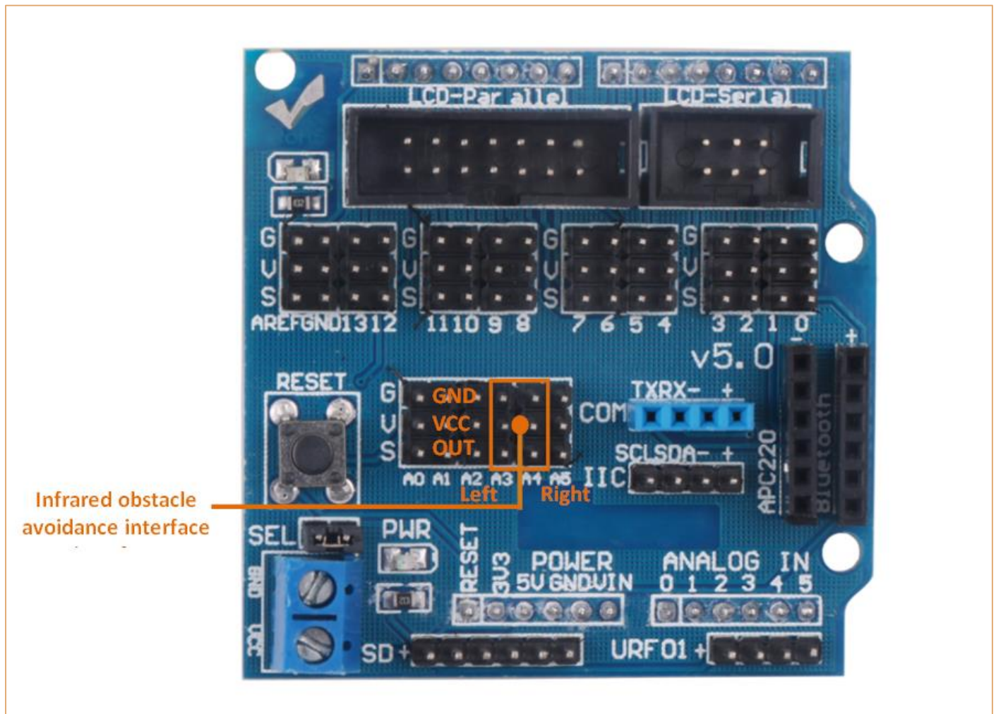
Figure 3.2.2.5 Wire connection diagram
