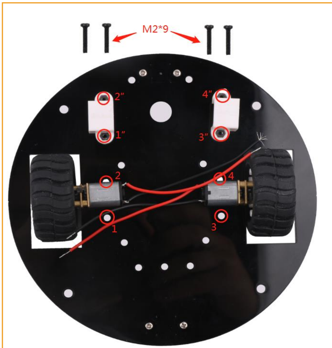
Figure 3.1.2.3 Effect diagram of motor mounting bracket installation
