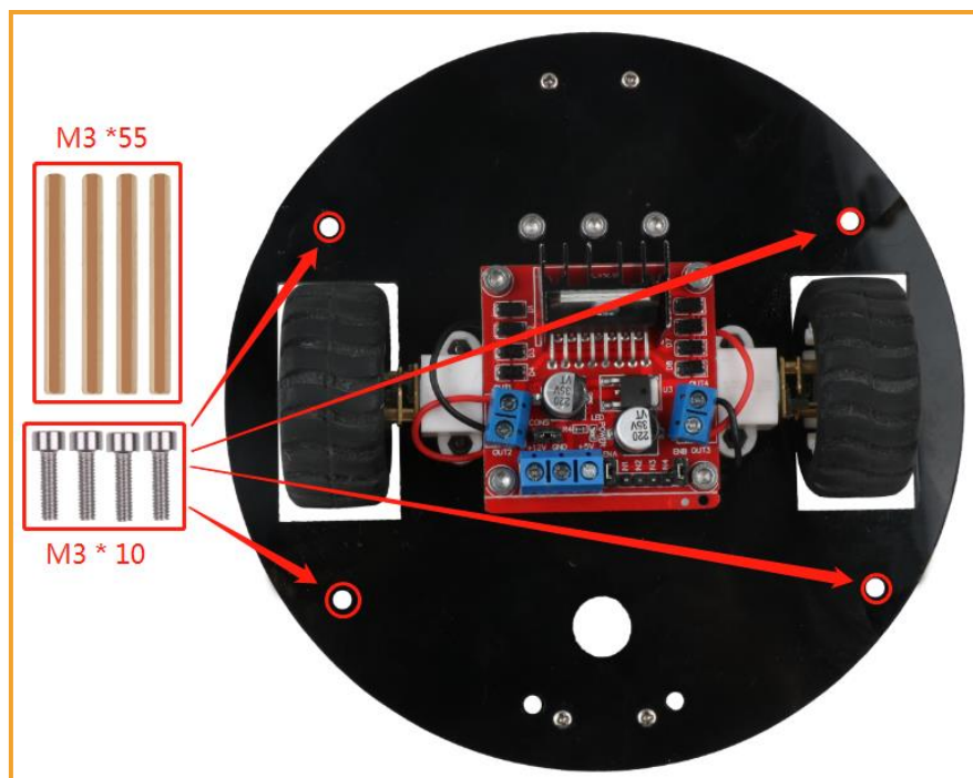
Figure 3.1.4.4 Schematic diagram of the installation of the upper acrylic plate pillar
