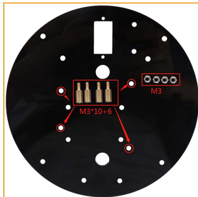
Figure 3.1.5.1 Schematic diagram of Keywish Uno R3 Motherboard pillar installation
