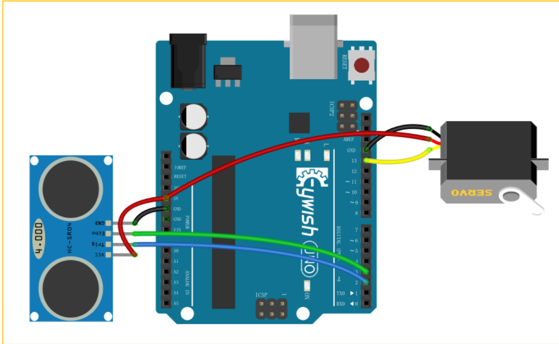
Figure .3.2.4.8 Wiring of the Steering Gear and Ultrasonic Module
