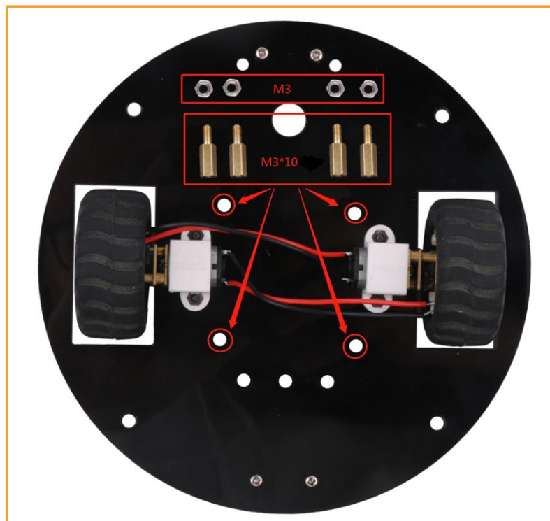
Figure 3.1.3.1 Schematic diagram of motor drive board pillar installation
