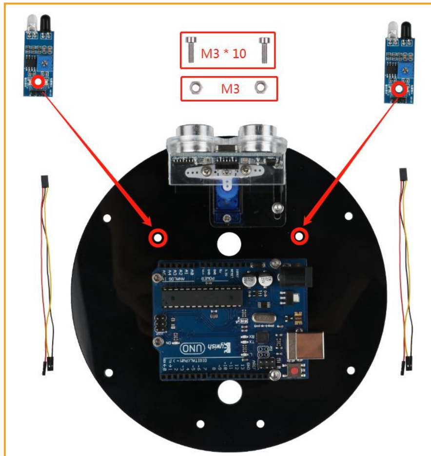
Figure 3.1.7.1 Schematic diagram of infrared obstacle avoidance module installation
