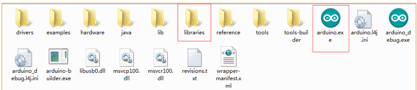
Figure 2.1.11 Software Catalog
