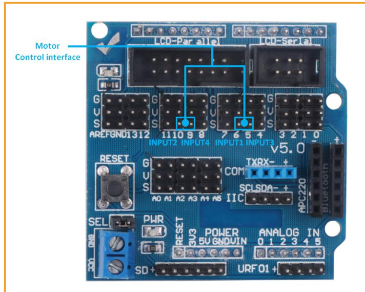
Figure.3.1.2.8 L298N and Arduino Expansion Board Connection Diagram
