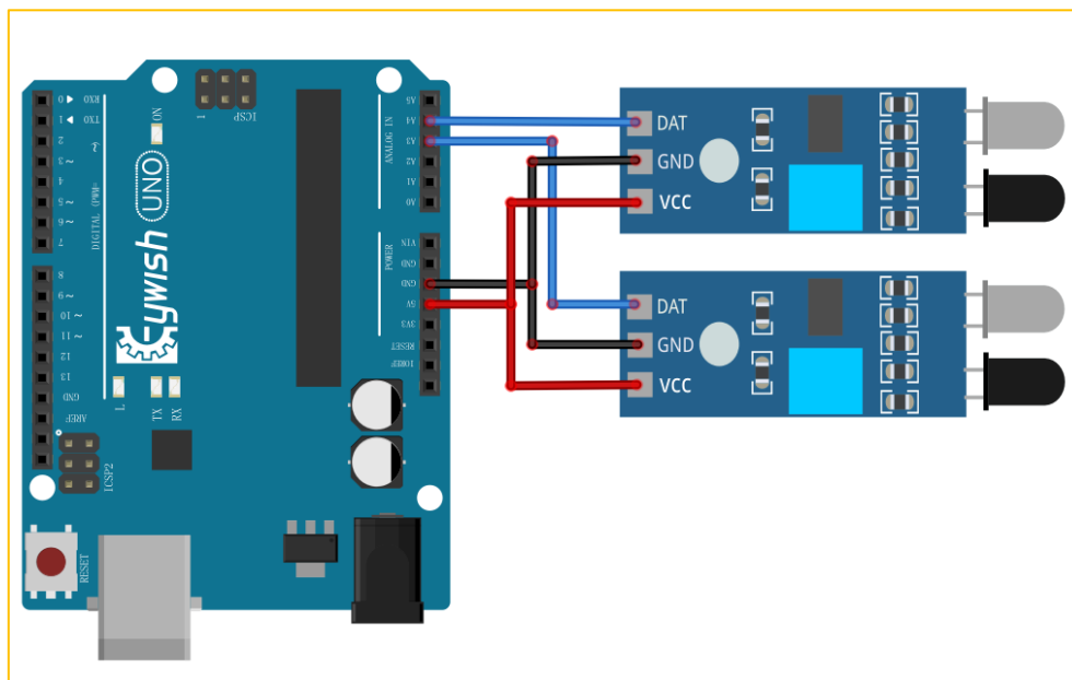
Figure 3.2.2.3 Connection of Arduino and Sensor
