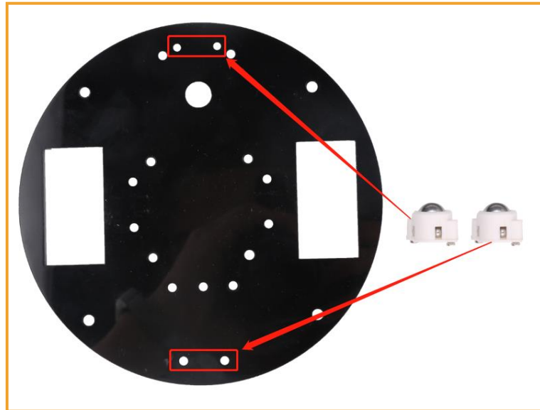
Figure 3.1.1.1 Schematic diagram of the universal wheel installation
