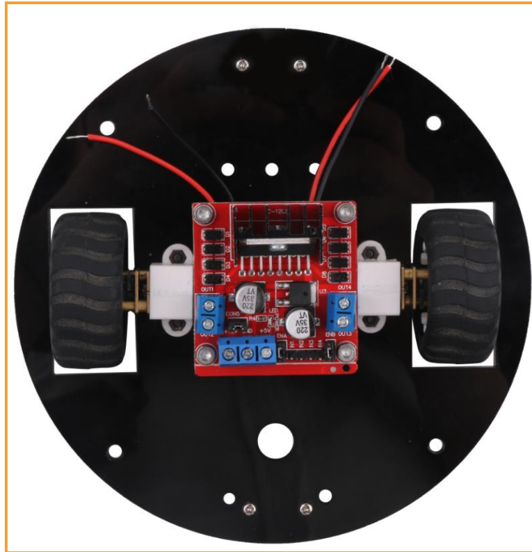
Figure 3.1.3.4 Effect diagram of Motor Driver Board Installation
