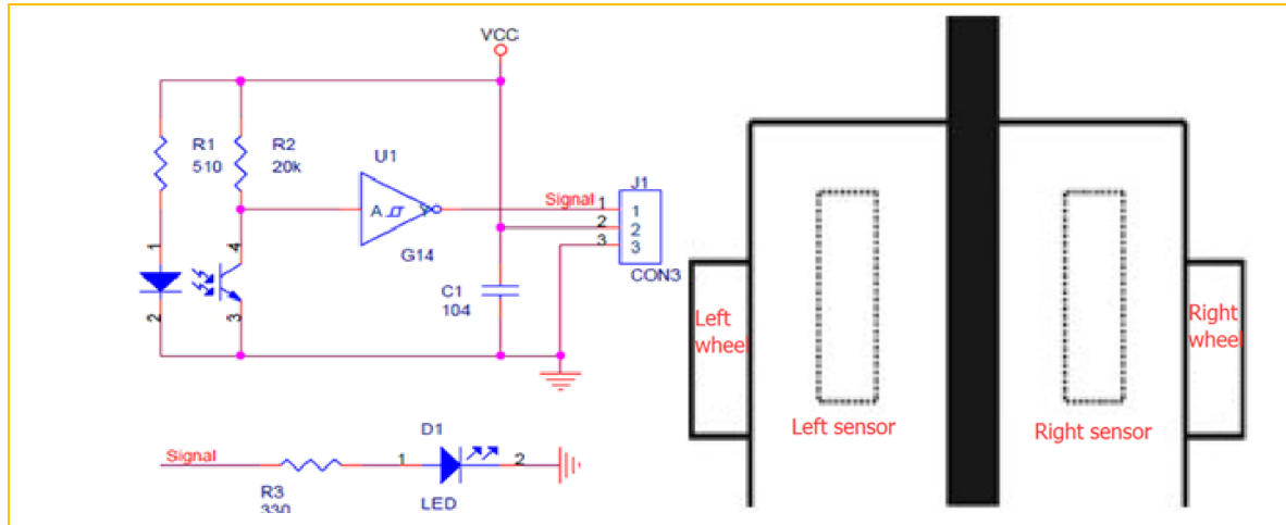
Figure 3.2.3.2 Schematic Diagram of Tracing Module Figure 3.2.3.3 Diagram of Tracing Module Installation
