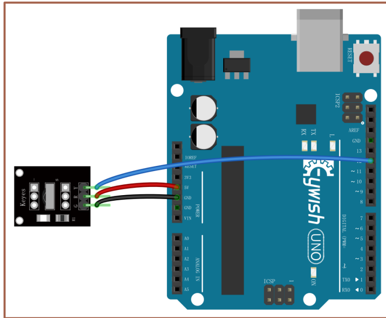
Figure .3.1.5.3 Infrared Module Connection Diagram
