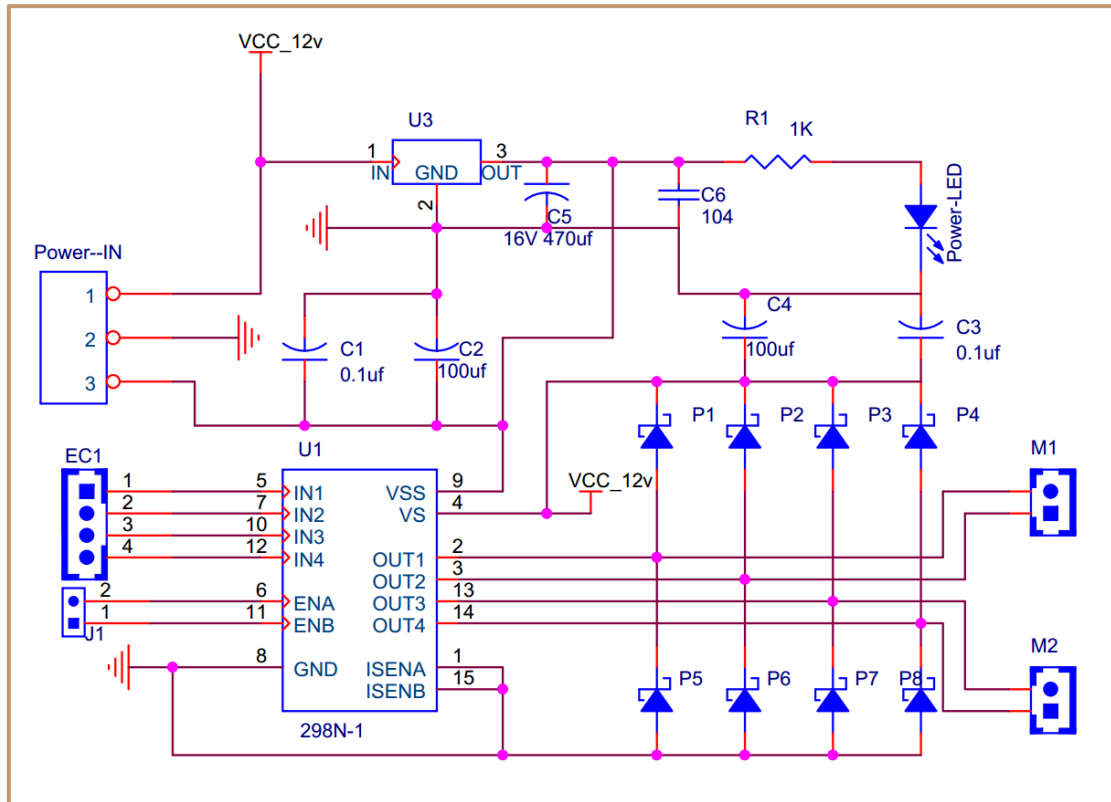
Figure .3.2.1.4 Schematic Diagram of Motor Drive
