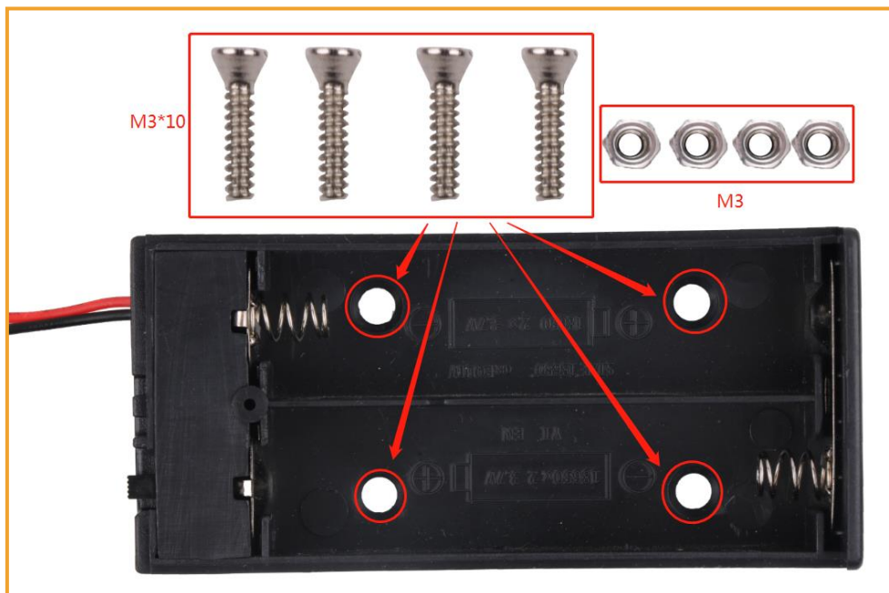
Figure 3.1.5.3 Schematic diagram of Battery box fixed
