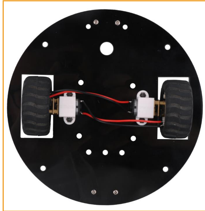
Figure 3.1.2.5 Motor installation effect diagram
