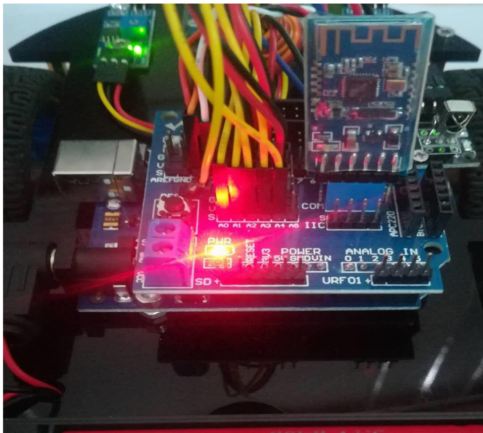
Figure .3.2.6.4 Installation of Bluetooth Module
