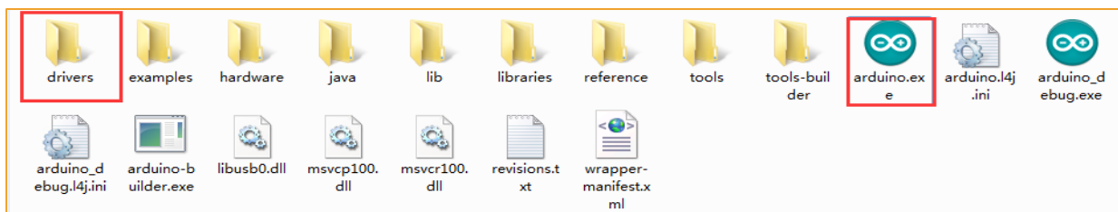
Figure 2.1.3 Extracted files
