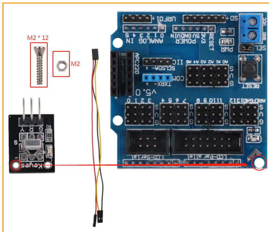
Figure 3.1.9.1 Schematic diagram of infrared remote control receiver installation
