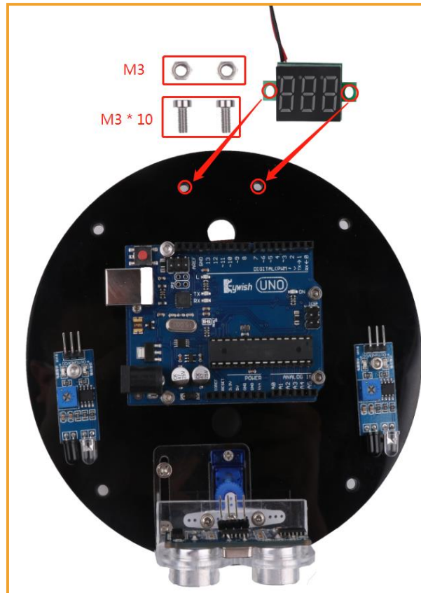
Figure 3.1.8.1 Schematic diagram of voltage display module installation
