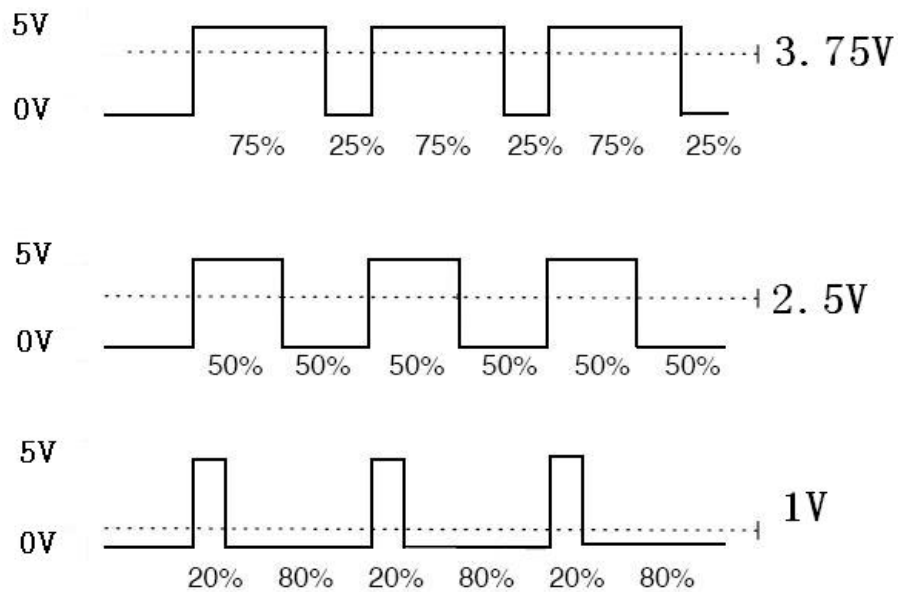
Figure 3.2.1.6 Relation between Pulse and Voltage
