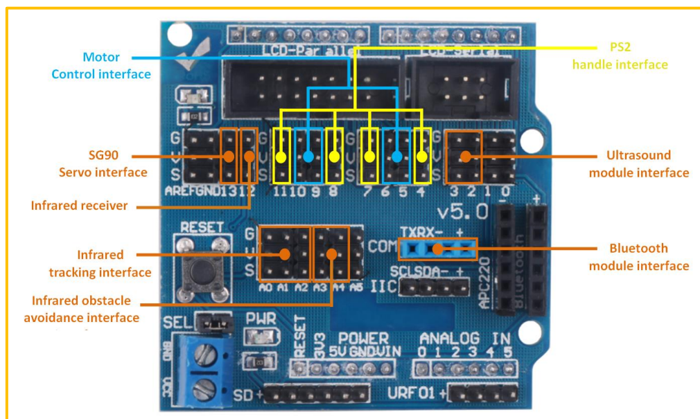
Figure 3.1.11.1 Expansion board connection diagram
