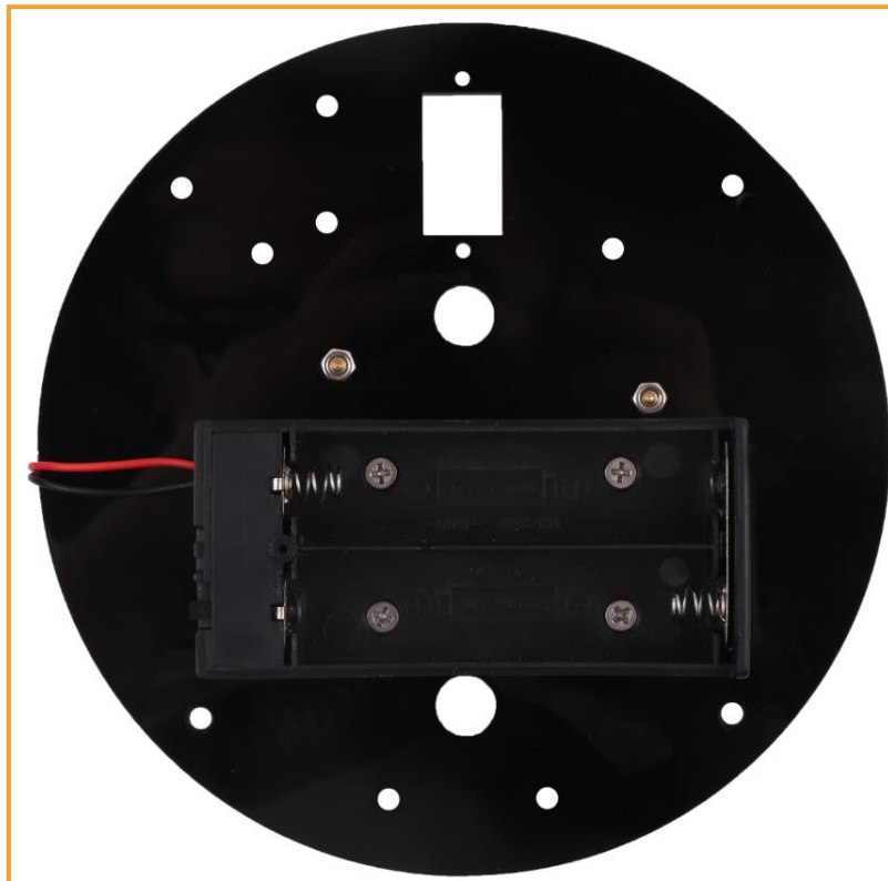
Figure 3.1.5.6 Effect diagram of Battery box installation
