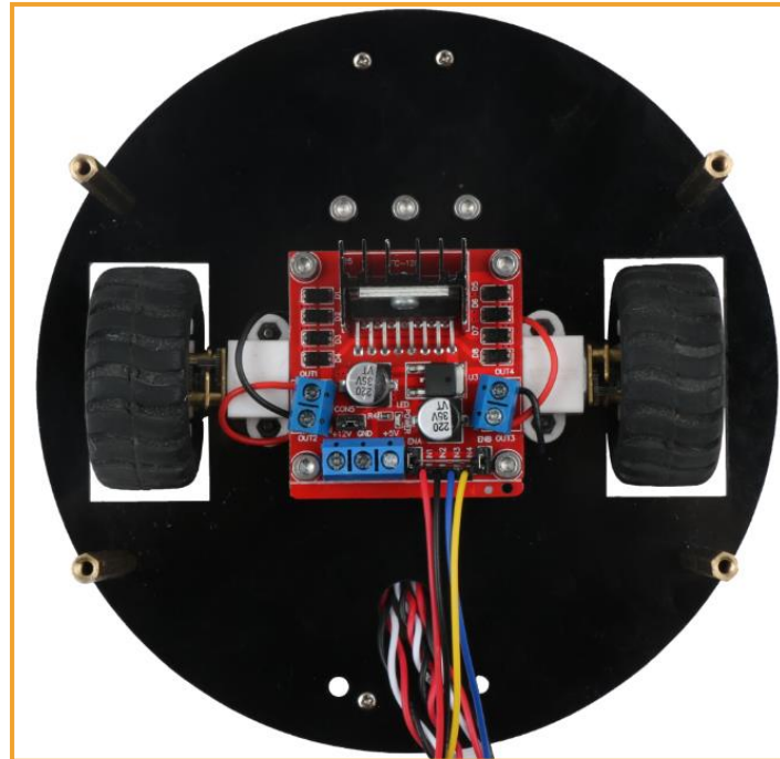
Figure 3.1.4.5 Effect diagram of the installation of the upper acrylic plate pillar
