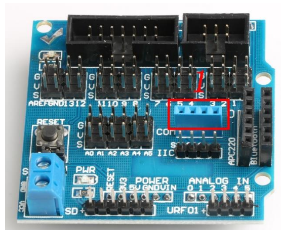
Figure .3.2.6.3 Wiring Positions of Bluetooth
