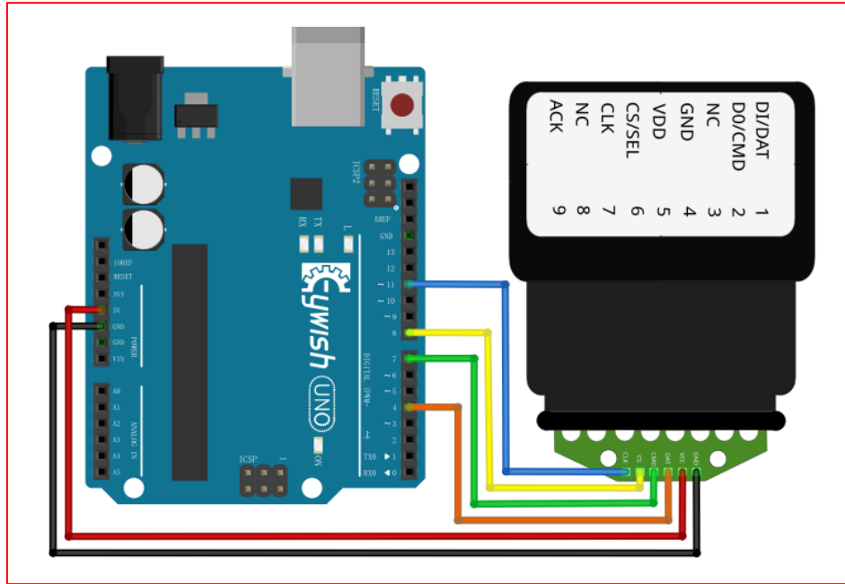
Figure 3.2.7.5 Connection of Arduino and Receiving Head Wires
