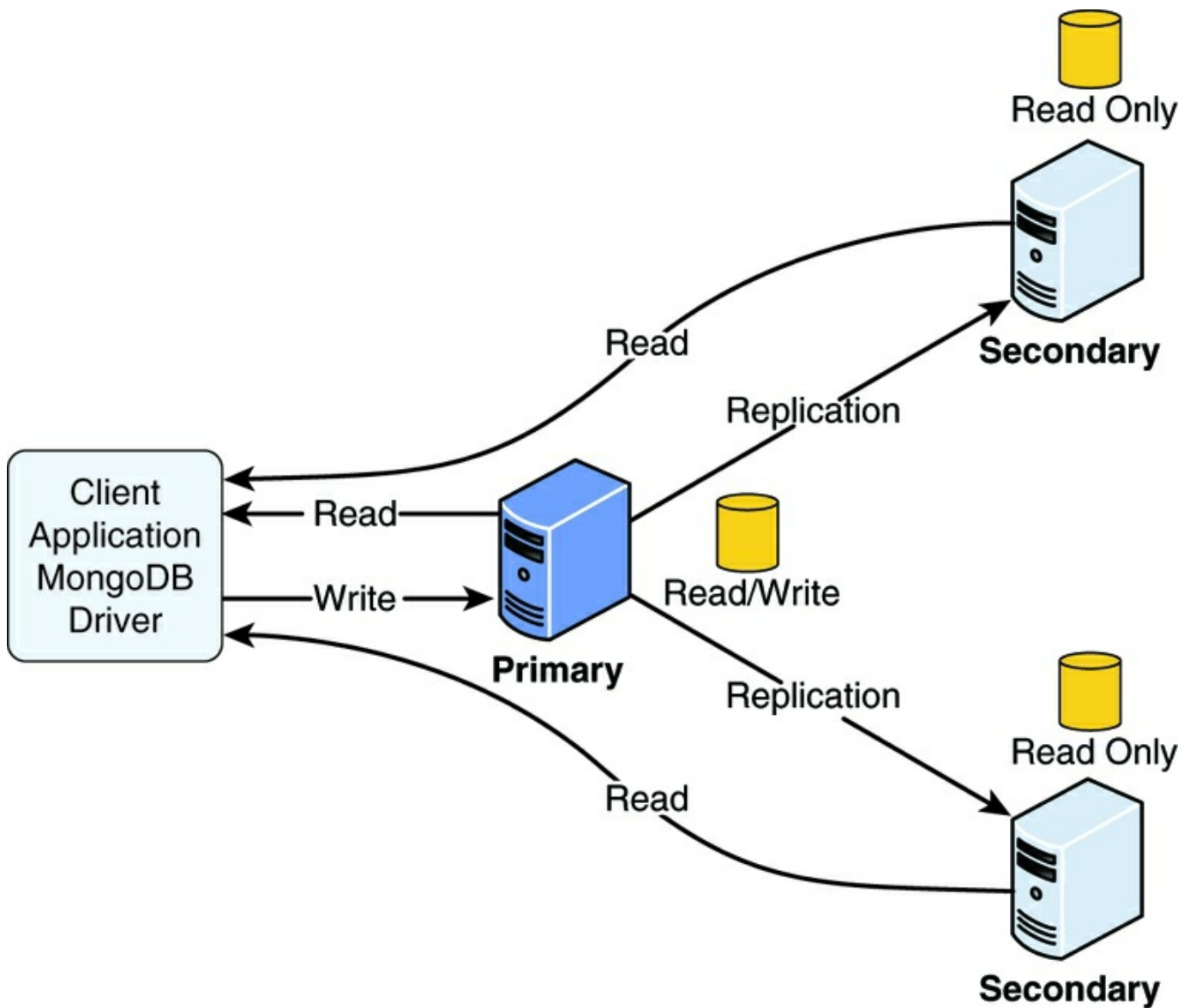
Figure 17.1 Implementing a replica set in MongoDB
