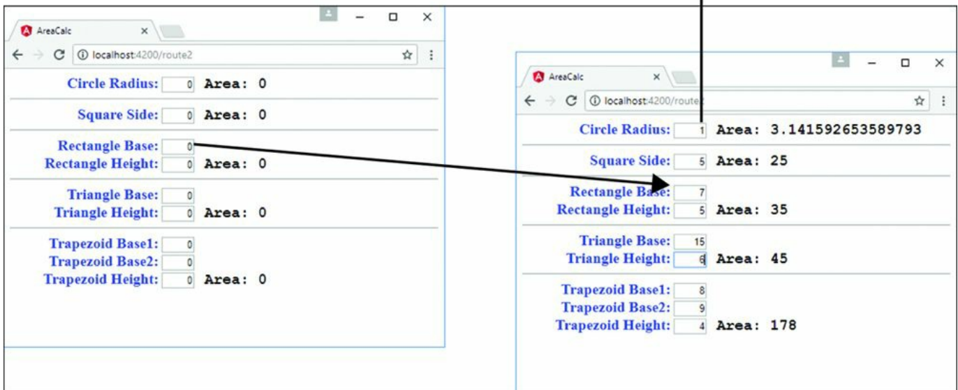
Figure 29.2 An Angular application that uses a custom service to automatically calculate the areas of different shapes
