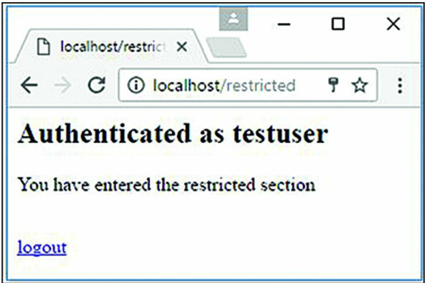
Figure 19.5 Implementing session authentication in Node.js using Express session middleware
