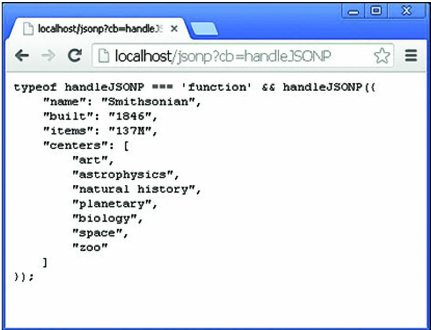
Figure 18.4 Sending JSON and JSONP data to the browser
