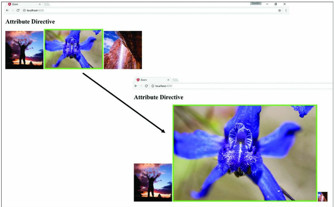
Figure 26.1 Applying a custom attribute directive
