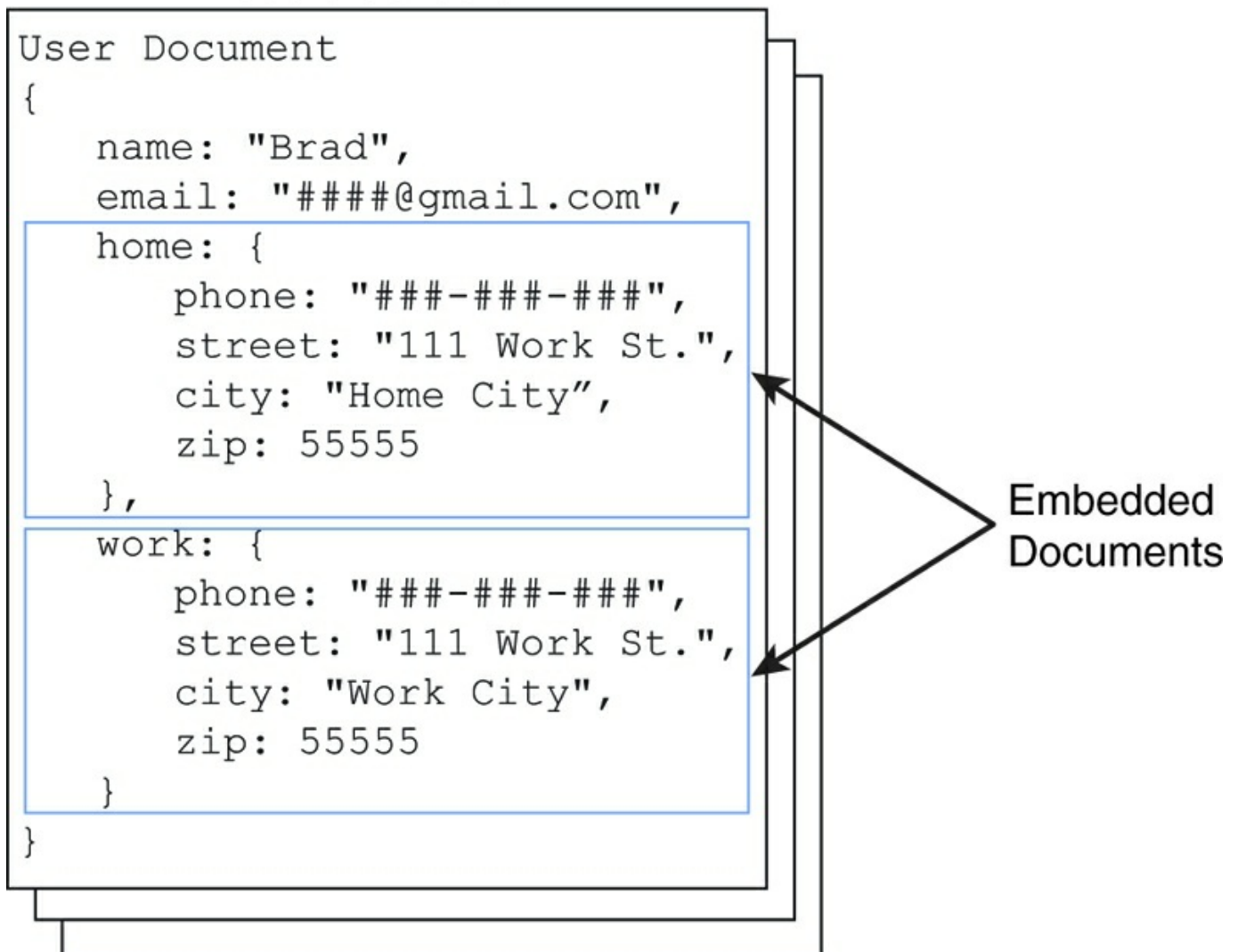
Figure 11.2 Defining denormalized MongoDB documents by implementing embedded objects inside a document
