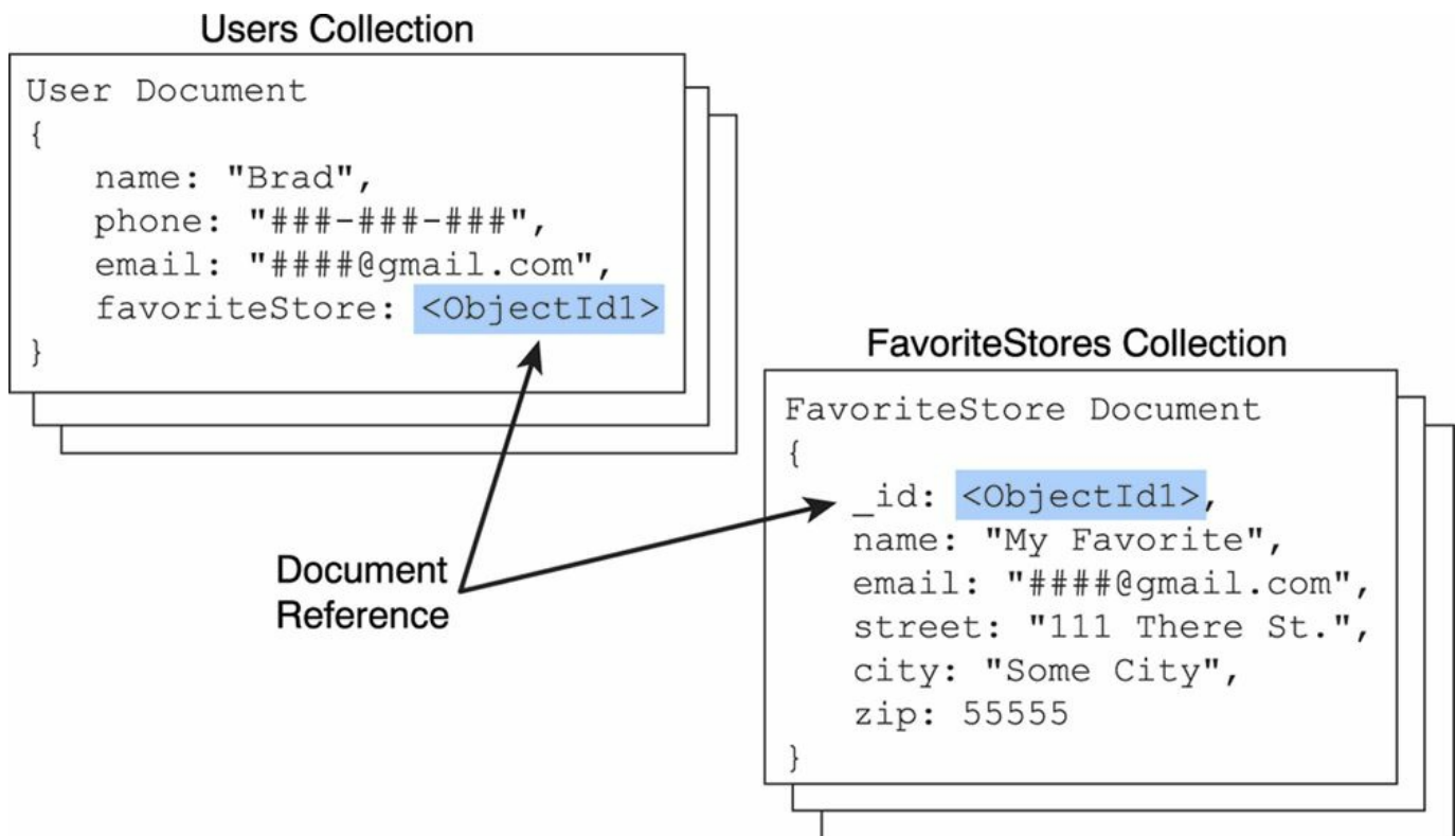
Figure 11.1 Defining normalized MongoDB documents by adding a reference to documents in another collection
