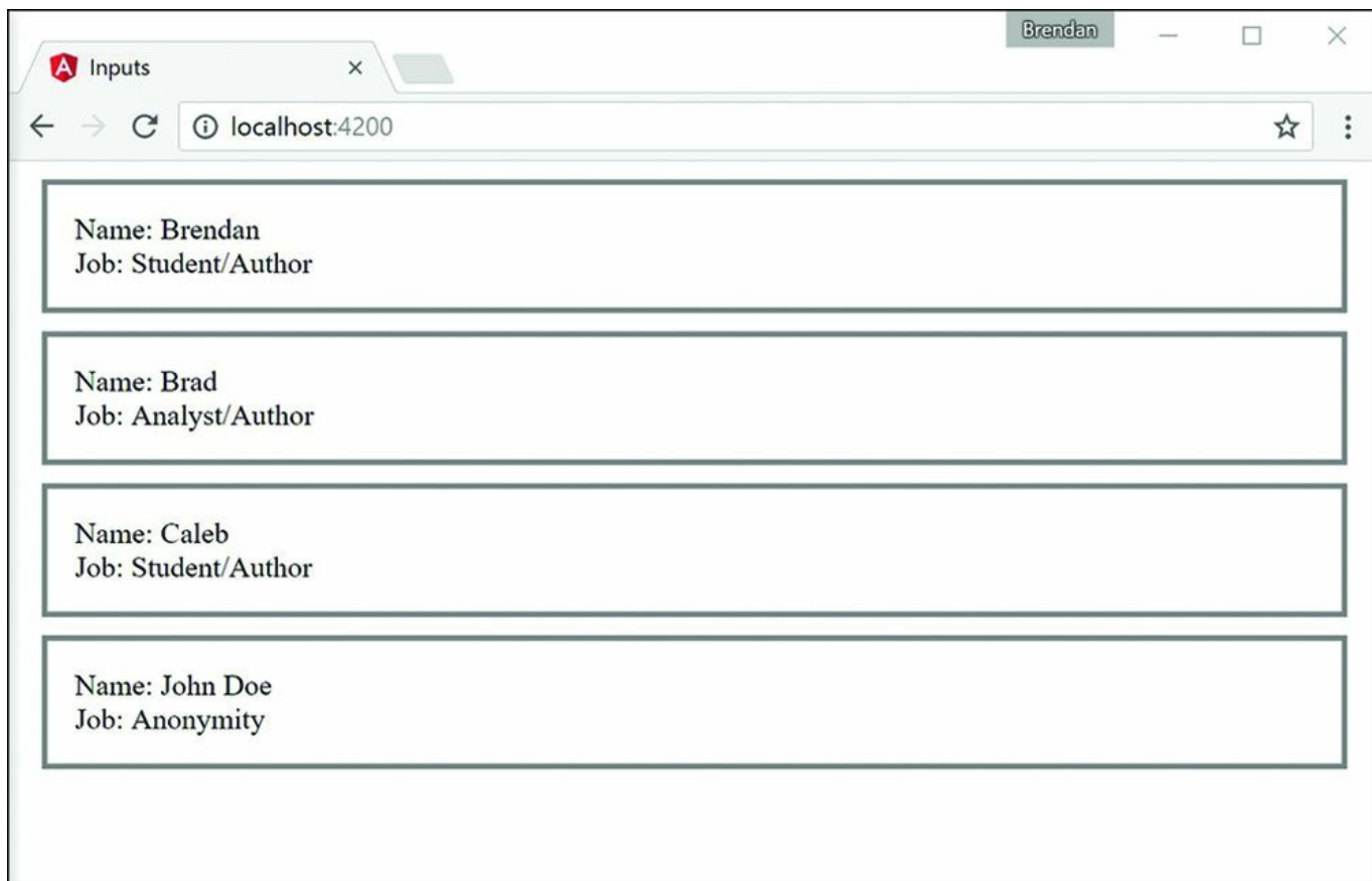
Figure 22.5 Displaying information passed down through inputs
