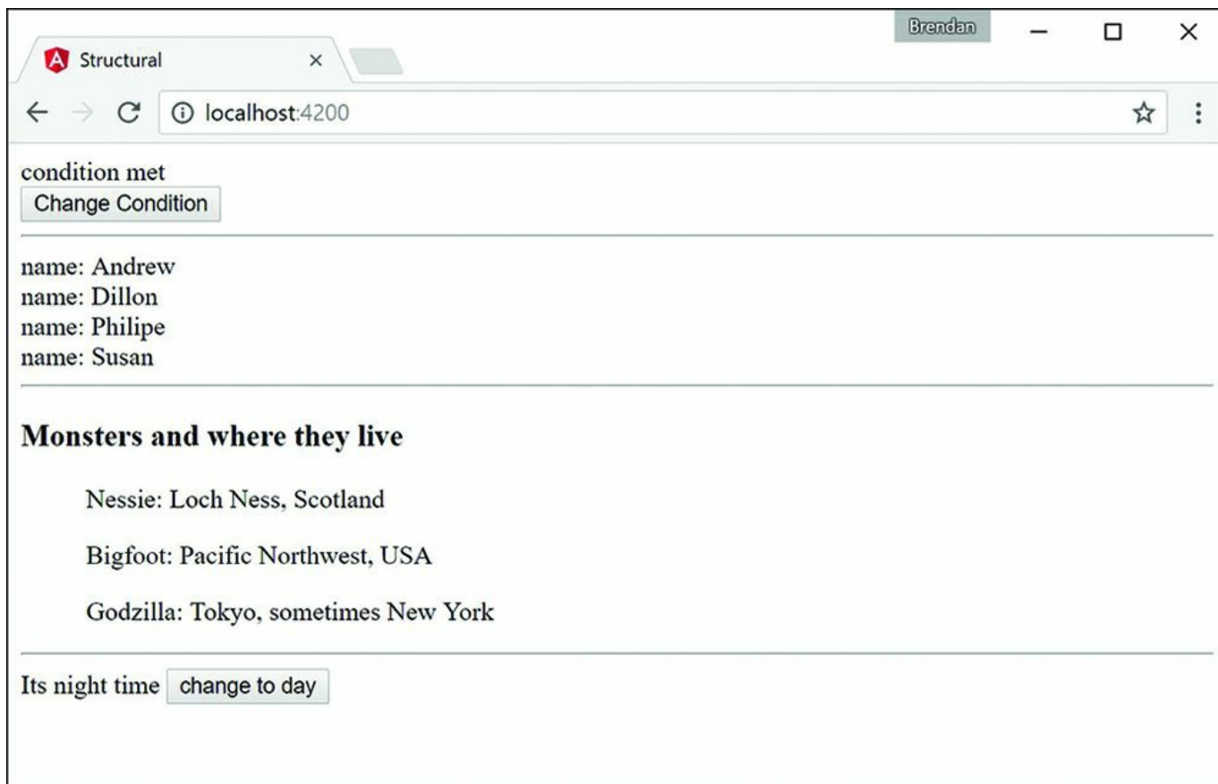
Figure 25.1 Using built-in structural directives
