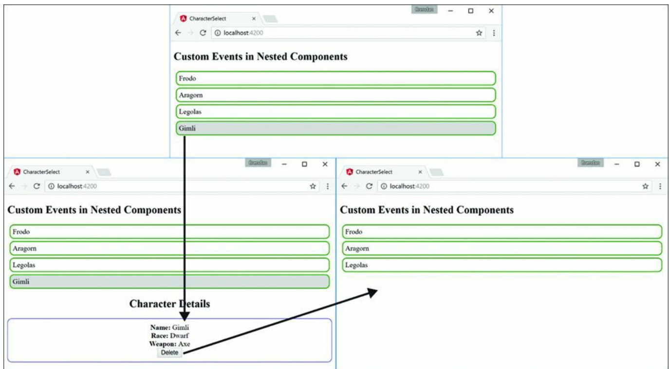
Figure 27.2 Using events to send and delete data
