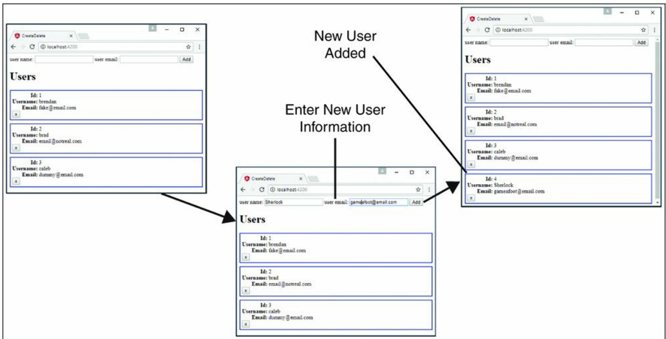
Figure 28.2 Implementing a simple mock server to create and delete items from a database
