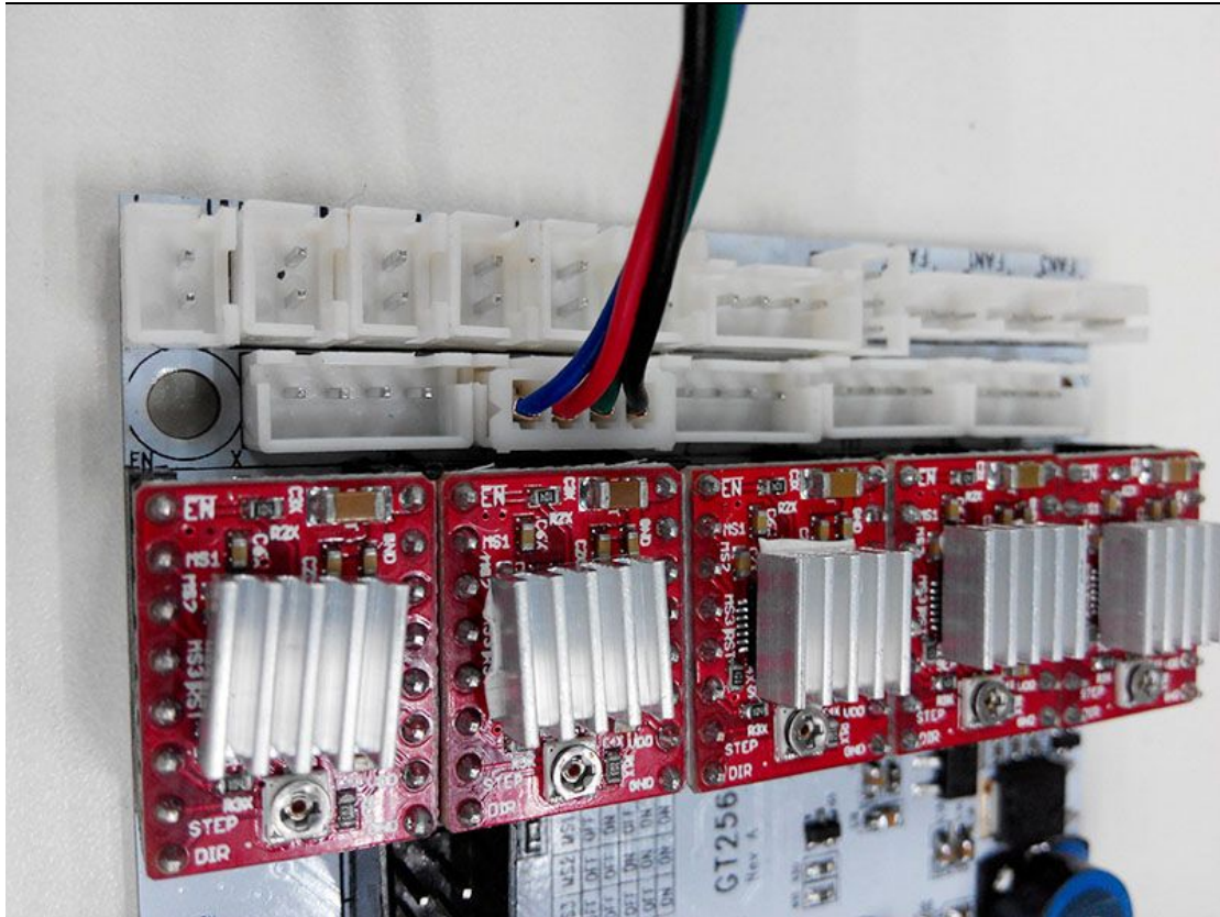
3) Connect wires for the 2 Z-axis motors.
