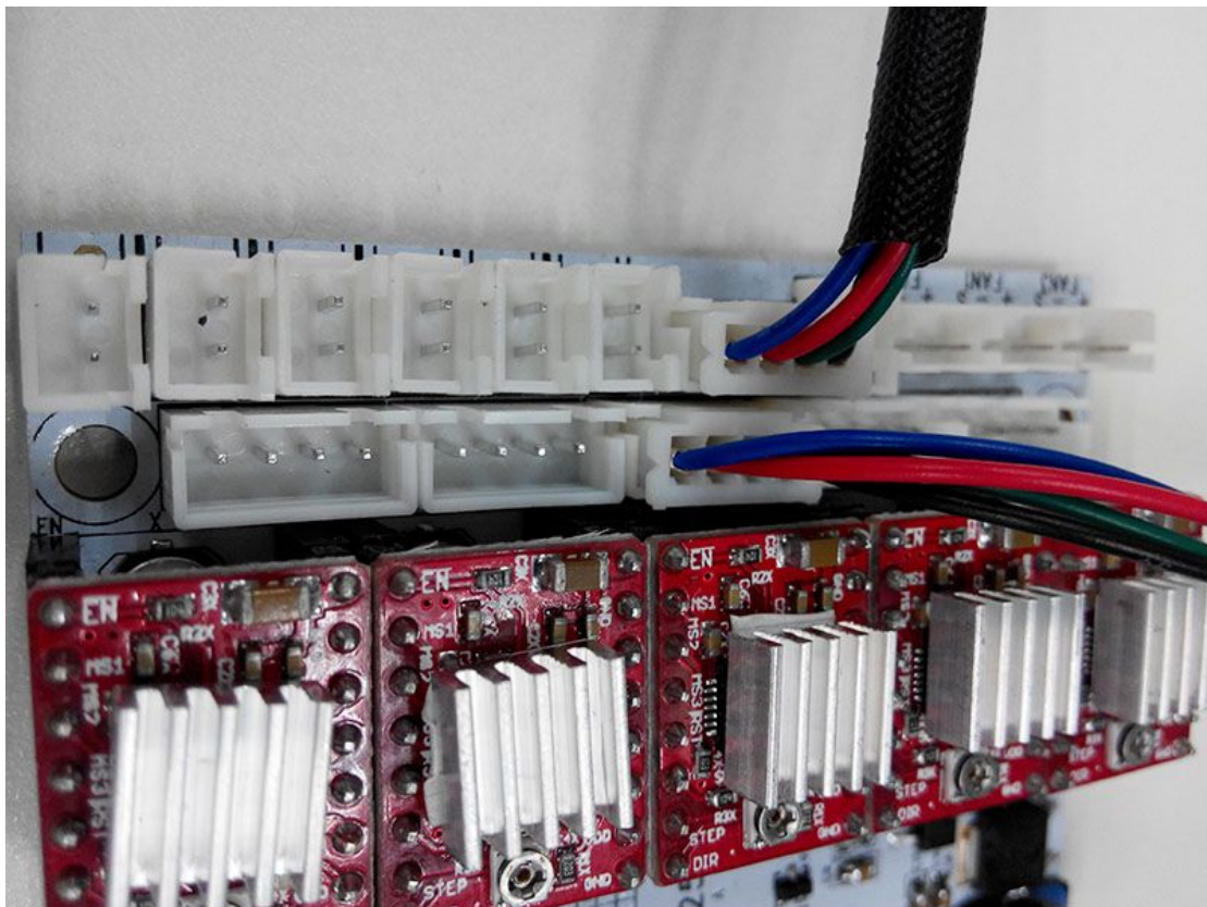
4) Connect Extruder motors
