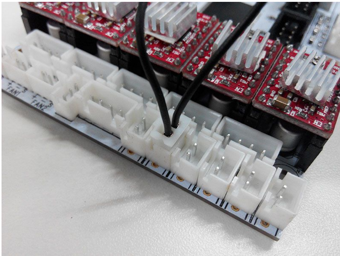
3) Connect wires for endstop of Z-axis at Z-Min.
