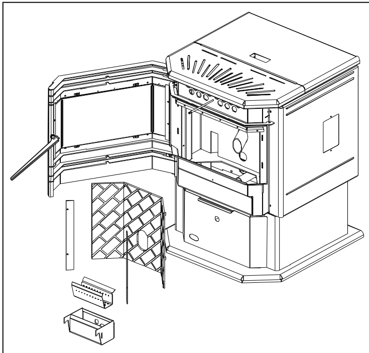
Figure 11: Firebox Components Removal.
