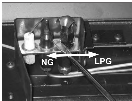
Figure 26: Setting Regulator gas type to LP.
