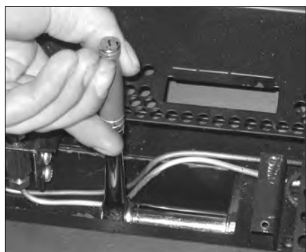
Figure 23: Orifice Removal.
