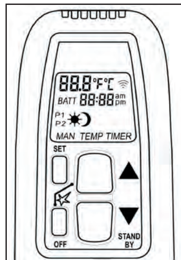
Figure 6: Remote Control.
