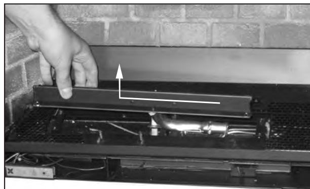
Figure 22: Burner Removal.
