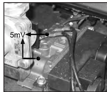
Figure 82: Voltage Across Valve & Spade.
