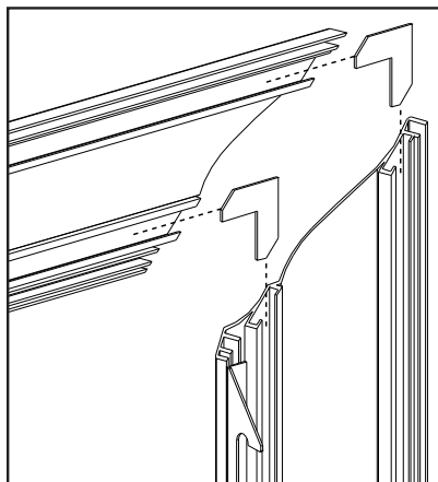
Figure 61: Corner brackets being Installed into Trim.
