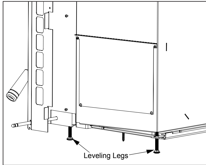
Figure 15: Leveling legs.
