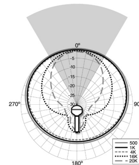
Figure 2b. Typical polar pattern (with full frequency response) of a conventional cardioid microphone
