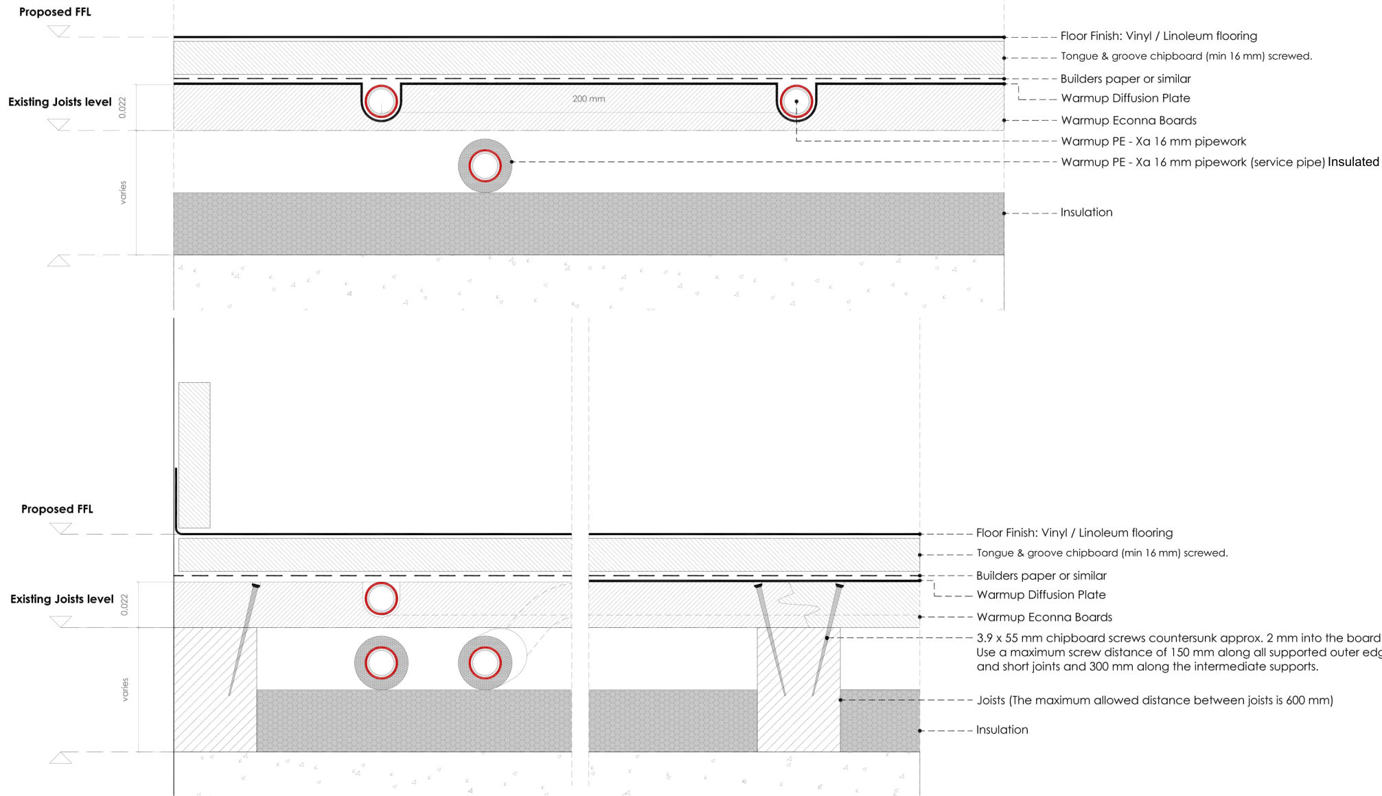
VINYL / LINOLEUM FLOORING _Warmup Eonna Joisted Floor System
