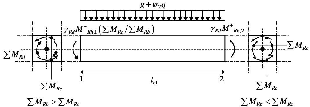
Figure 4-1 Capacity Design Shear Force for beams
